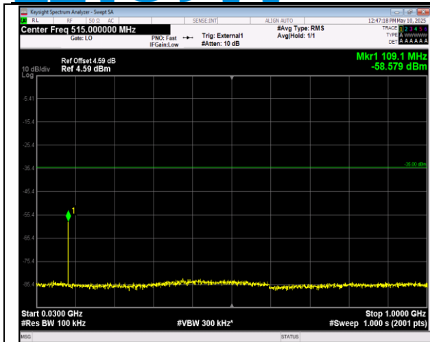
41-41-5MHz-20MHz-16QAM-16QAM-41373-41490-25RB #0-100RB#0-30~1000MHz-PASS
