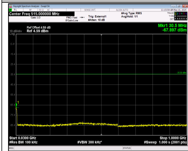
41-41-20MHz-5MHz-16QAM-16QAM-40595-40712-1RB# 0-0RB#0-30~1000MHz-PASS
