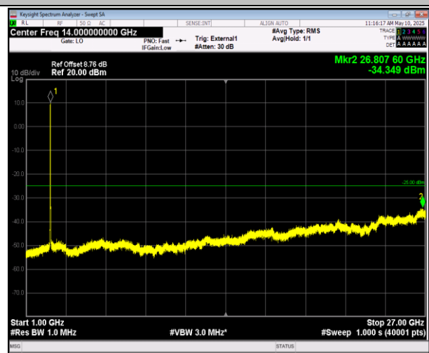
41-41-20MHz-5MHz-16QAM-16QAM-40595-40712-1RB#0- 0RB#0-1000~27000MHz-PASS
