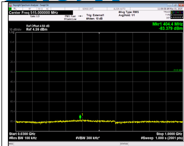
41-41-20MHz-5MHz-QPSK-QPSK-40595-40712-1RB#0-0RB#0-30~1000MHz-PASS
