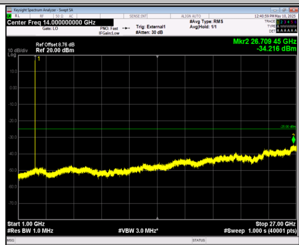
41-41-5MHz-20MHz-16QAM-16QAM-40528-40645-25RB#0 -100RB#0-1000~27000MHz-PASS
