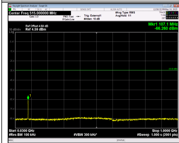
41-41-20MHz-5MHz-QPSK-QPSK-39750-39867-1RB#0-0 ORB#0-30~1000MHz-PASS
