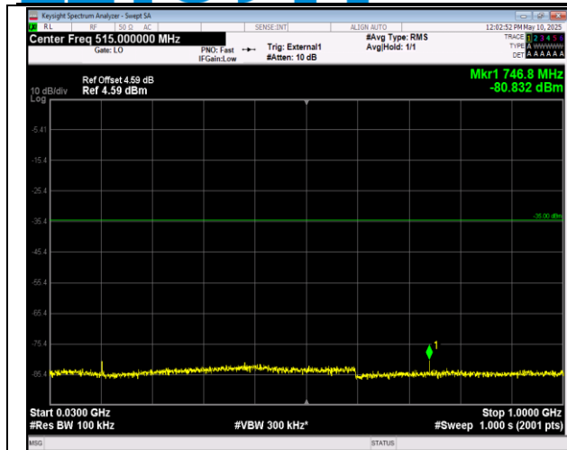
41-41-20MHz-10MHz-QPSK-QPSK-39750-39894-1RB#9 9-ORB#0-30~1000MHz-PASS
