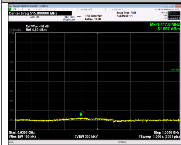
41-41-5MHz-20MHz-16QAM-16QAM-40528-40645-25RB #0-100RB#0-30~1000MHz-PASS
