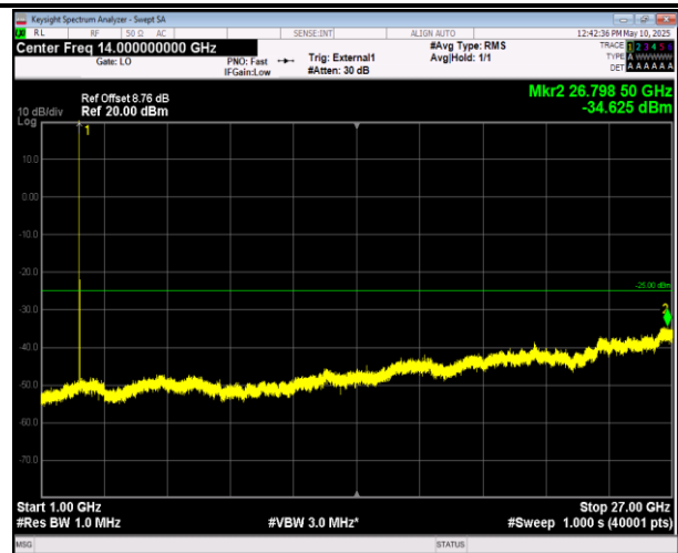
41-41-5MHz-20MHz-16QAM-16QAM-40528-40645-1RB#24 -ORB#0-1000~27000MHz-PASS
