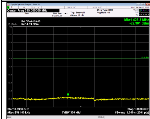
41-41-20MHz-5MHz-16QAM-16QAM-40595-40712-1RB# 0-1RB#24-30~1000MHz-PASS
