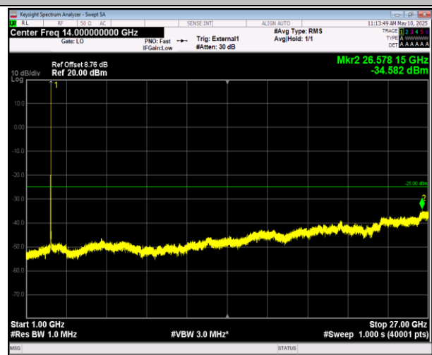
41-41-20MHz-5MHz-16QAM-16QAM-40595-40712-100RB# 0-25RB#0-1000~27000MHz-PASS
