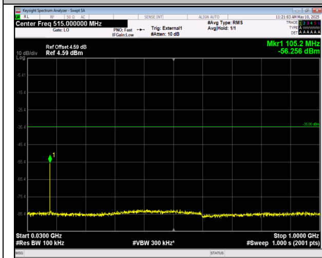
41-41-20MHz-5MHz-QPSK-QPSK-41440-41557-1RB#99-0RB#0-30~1000MHz-PASS
