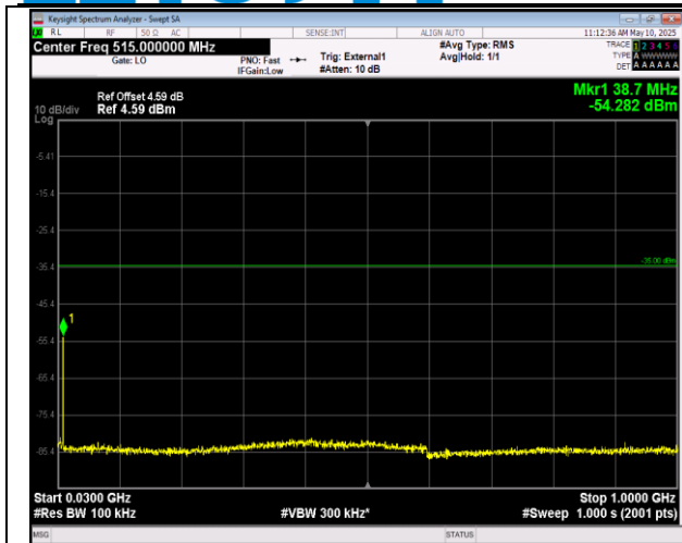
41-41-20MHz-5MHz-QPSK-QPSK-40595-40712-100RB# 0-25RB#0-30~1000MHz-PASS
