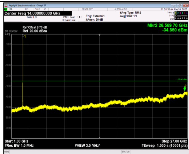
41-41-20MHz-5MHz-16QAM-16QAM-41440-41557-100RB# 0-25RB#0-1000~27000MHz-PASS
