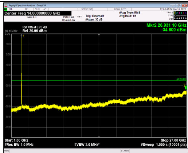
41-41-20MHz-10MHz-16QAM-16QAM-39750-39894-1RB#0 -1RB#49-1000~27000MHz-PASS
