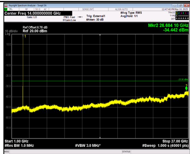
41-41-5MHz-20MHz-16QAM-16QAM-41373-41490-25RB#0 -100RB#0-1000~27000MHz-PASS
