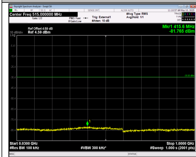
41-41-20MHz-5MHz-QPSK-QPSK-40595-40712-1RB#0-01RB#24-30~1000MHz-PASS
