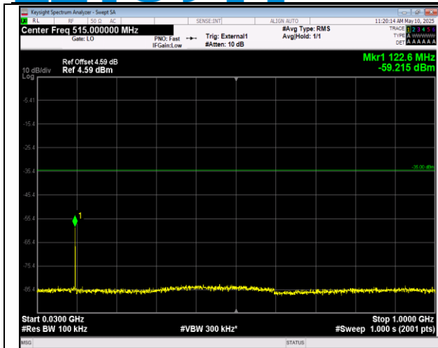
41-41-20MHz-5MHz-16QAM-16QAM-41440-41557-100R B#0-25RB#0-30~1000MHz-PASS
