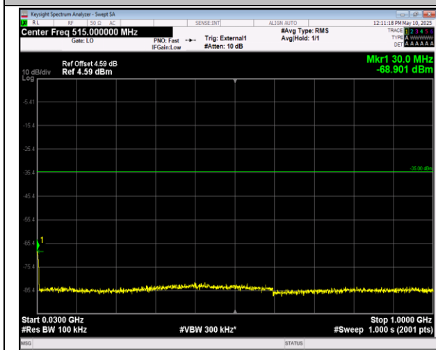
41-41-20MHz-10MHz-16QAM-16QAM-40571-40715-1RB #0-0RB#0-30~1000MHz-PASS
