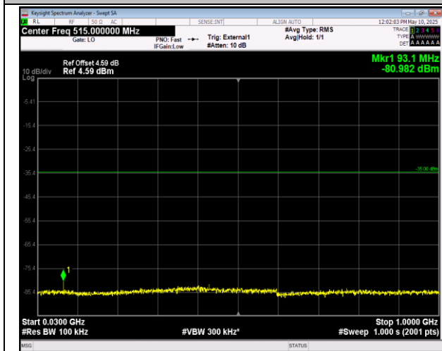
41-41-20MHz-10MHz-16QAM-16QAM-39750-39894-100 RB#0-50RB#0-30~1000MHz-PASS
