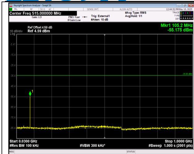
41-41-5MHz-20MHz-QPSK-QPSK-41373-41490-1RB#0-1RB#99-30~1000MHz-PASS
