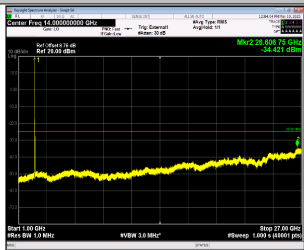
41-41-20MHz-10MHz-16QAM-16QAM-39750-39894-1RB#9 9-0RB#0-1000~27000MHz-PASS
