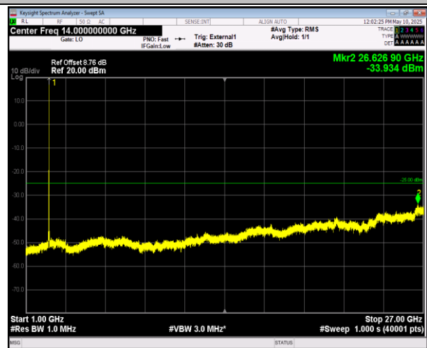
41-41-20MHz-10MHz-16QAM-16QAM-39750-39894-100RB #0-50RB#0-1000~27000MHz-PASS
