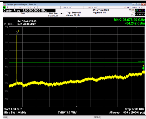
41-41-20MHz-10MHz-16QAM-16QAM-39750-39894-1RB#0 -ORB#0-1000~27000MHz-PASS
