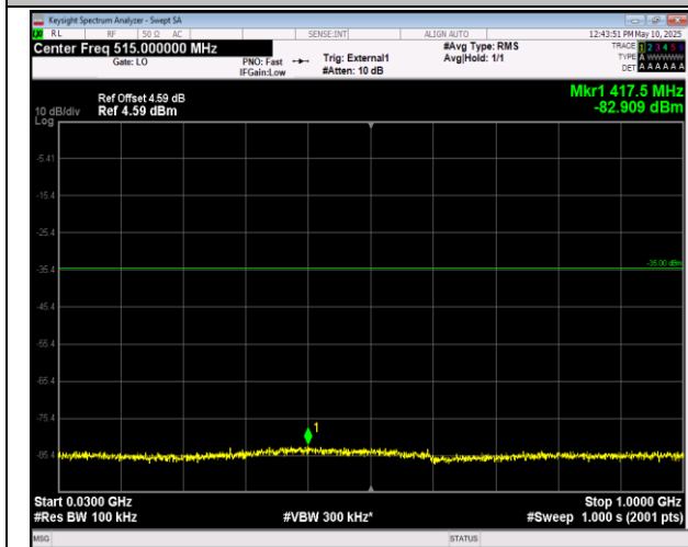
41-41-5MHz-20MHz-QPSK-QPSK-41373-41490-1RB#0-ORB#0-30~1000MHz-PASS
