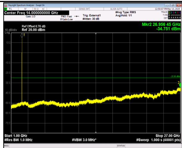
41-41-5MHz-20MHz-16QAM-16QAM-41373-41490-1RB#0- ORB#0-1000~27000MHz-PASS
