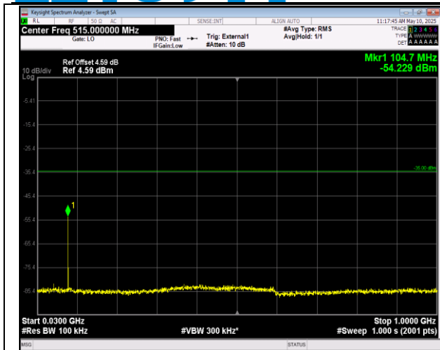
41-41-20MHz-5MHz-QPSK-QPSK-41440-41557-1RB#0-1RB#24-30~1000MHz-PASS
