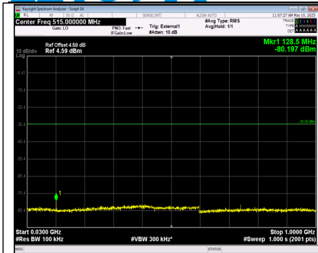
41-41-20MHz-5MHz-QPSK-QPSK-39750-39867-1RB#99 -ORB#0-30~1000MHz-PASS
