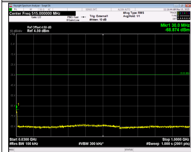
41-41-20MHz-5MHz-QPSK-QPSK-41440-41557-1RB#0-ORB#0-30~1000MHz-PASS
