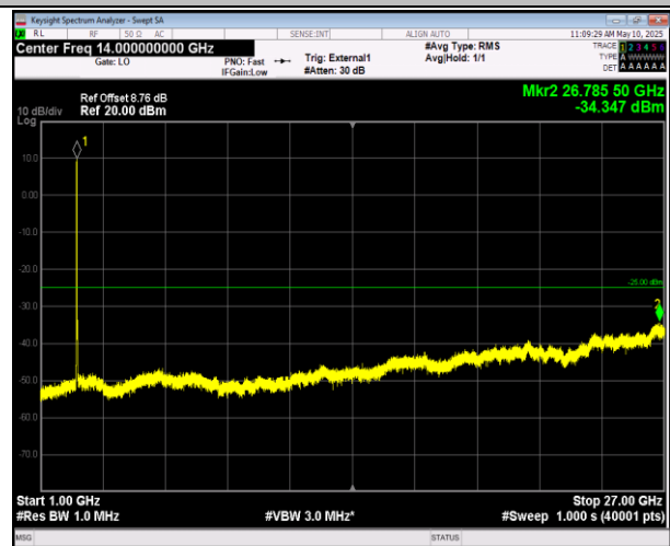
41-41-20MHz-5MHz-16QAM-16QAM-39750-39867-1RB#0- ORB#0-1000~27000MHz-PASS
