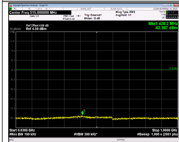
41-41-20MHz-10MHz-16QAM-16QAM-39750-39894-1RB #0-ORB#0-30~1000MHz-PASS
