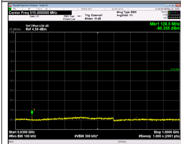
41-41-20MHz-5MHz-QPSK-QPSK-39750-39867-1RB#0-0 1RB#24-30~1000MHz-PASS
