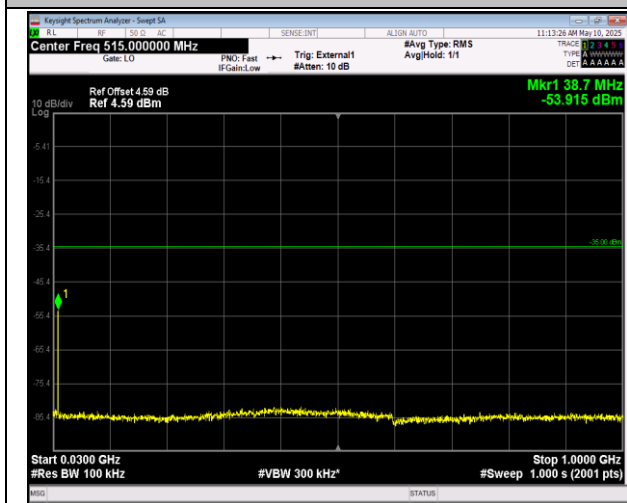
41-41-20MHz-5MHz-16QAM-16QAM-40595-40712-100RB# B#0-25RB#0-30~1000MHz-PASS
