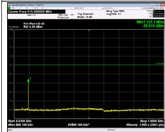
41-41-20MHz-5MHz-QPSK-QPSK-41440-41557-100RB#0-25RB#0-30~1000MHz-PASS
