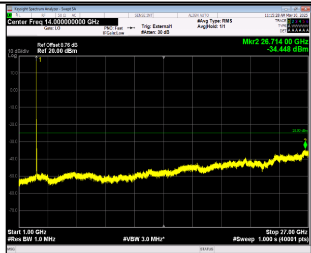
41-41-20MHz-5MHz-16QAM-16QAM-40595-40712-1RB#99 -ORB#0-1000~27000MHz-PASS
