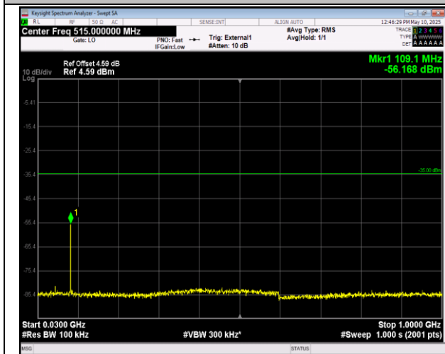
41-41-5MHz-20MHz-QPSK-QPSK-41373-41490-25RB#0-100RB#0-30~1000MHz-PASS
