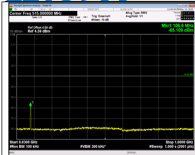
41-41-5MHz-20MHz-16QAM-16QAM-41373-41490-1RB# 0-ORB#0-30~1000MHz-PASS
