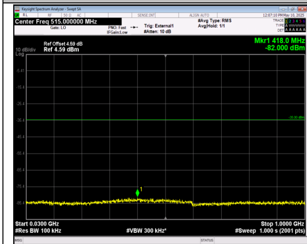
41-41-20MHz-10MHz-16QAM-16QAM-40571-40715-1RB #0-1RB#49-30~1000MHz-PASS
