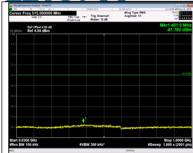
41-41-20MHz-5MHz-16QAM-16QAM-40595-40712-1RB# 99-ORB#0-30~1000MHz-PASS
