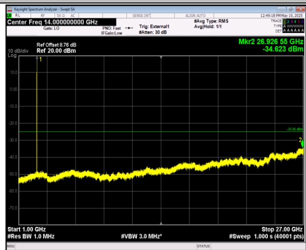
41-41-5MHz-20MHz-16QAM-16QAM-41373-41490-1RB#24 -ORB#0-1000~27000MHz-PASS
