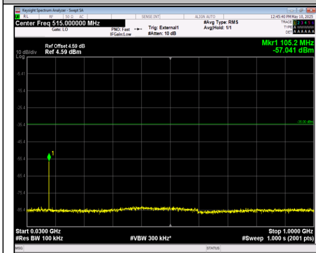
41-41-5MHz-20MHz-16QAM-16QAM-41373-41490-1RB# 0-1RB#99-30~1000MHz-PASS
