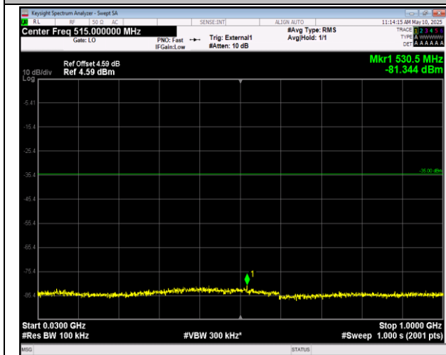
41-41-20MHz-5MHz-QPSK-QPSK-40595-40712-1RB#99-0RB#0-30~1000MHz-PASS
