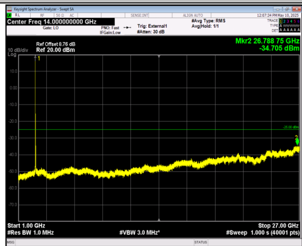
41-41-20MHz-10MHz-16QAM-16QAM-40571-40715-1RB#0 -1RB#49-1000~27000MHz-PASS
