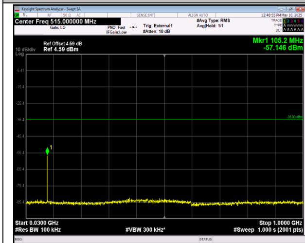
41-41-5MHz-20MHz-16QAM-16QAM-41373-41490-1RB# 24-ORB#0-30~1000MHz-PASS
