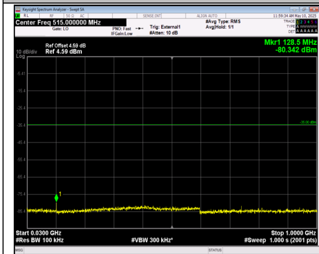
41-41-20MHz-10MHz-QPSK-QPSK-39750-39894-1RB#0 -1RB#49-30~1000MHz-PASS
