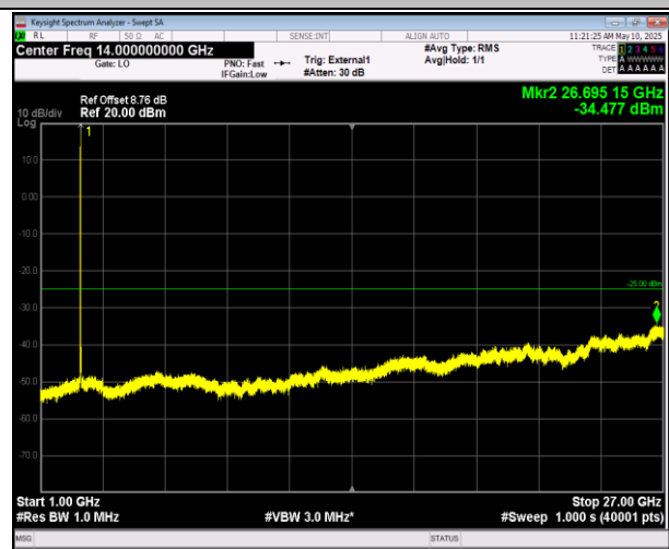
41-41-20MHz-5MHz-QPSK-QPSK-41440-41557-1RB#99-0RB#0-1000~27000MHz-PASS
