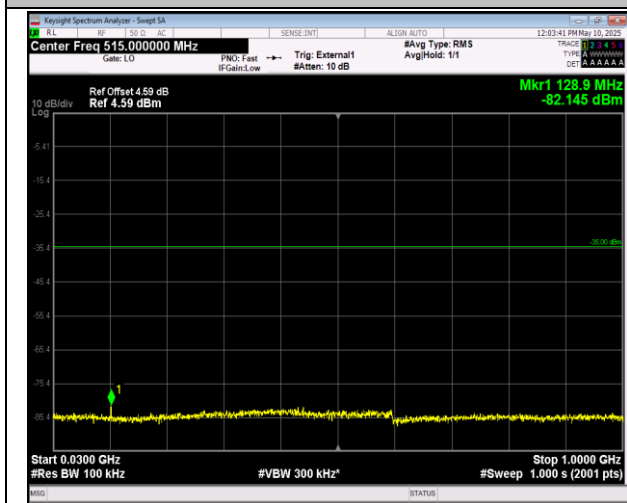
41-41-20MHz-10MHz-16QAM-16QAM-39750-39894-1RB #99-0RB#0-30~1000MHz-PASS
