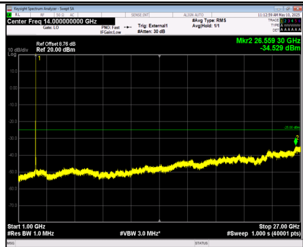
41-41-20MHz-5MHz-QPSK-QPSK-40595-40712-100RB#0- 25RB#0-1000~27000MHz-PASS
