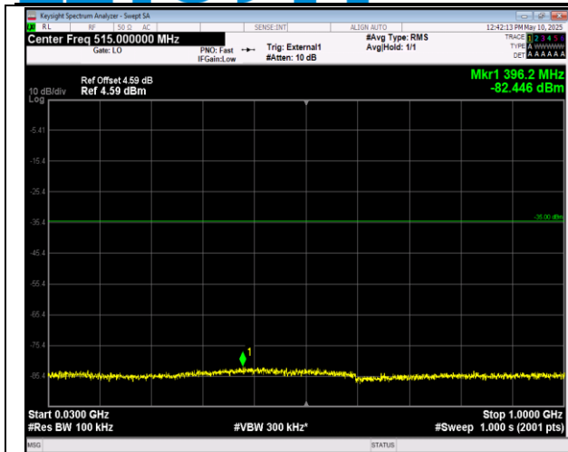
41-41-5MHz-20MHz-16QAM-16QAM-40528-40645-1RB# 24-ORB#0-30~1000MHz-PASS
