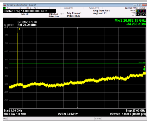
41-41-5MHz-20MHz-QPSK-QPSK-41373-41490-1RB#24-0RB#0-1000~27000MHz-PASS
