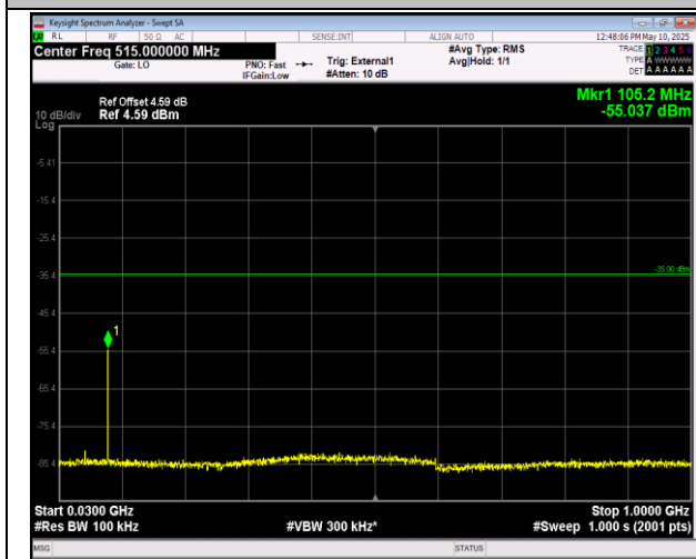
41-41-5MHz-20MHz-QPSK-QPSK-41373-41490-1RB#24-0RB#0-30~1000MHz-PASS
