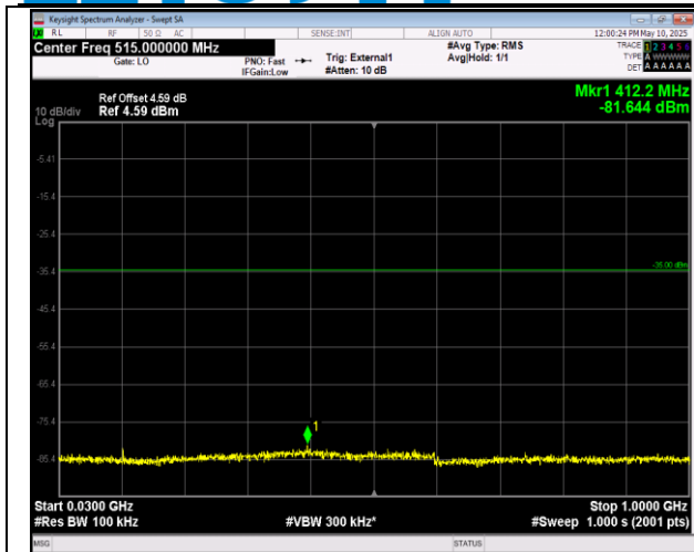
41-41-20MHz-10MHz-16QAM-16QAM-39750-39894-1RB #0-1RB#49-30~1000MHz-PASS
