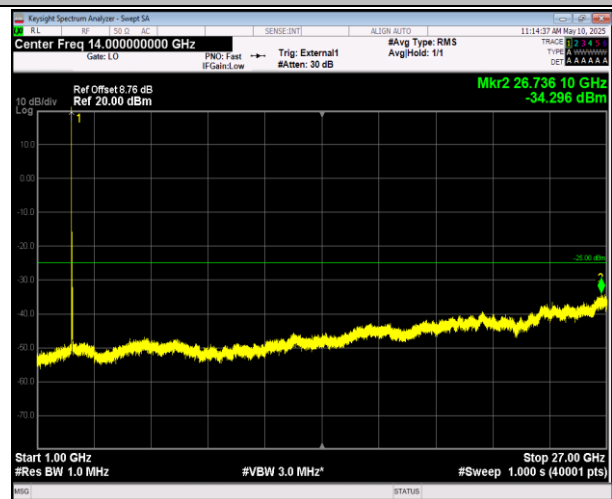
41-41-20MHz-5MHz-QPSK-QPSK-40595-40712-1RB#99-0RB#0-1000~27000MHz-PASS
