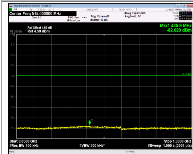
41-41-20MHz-5MHz-16QAM-16QAM-39750-39867-1RB# 0-ORB#0-30~1000MHz-PASS
