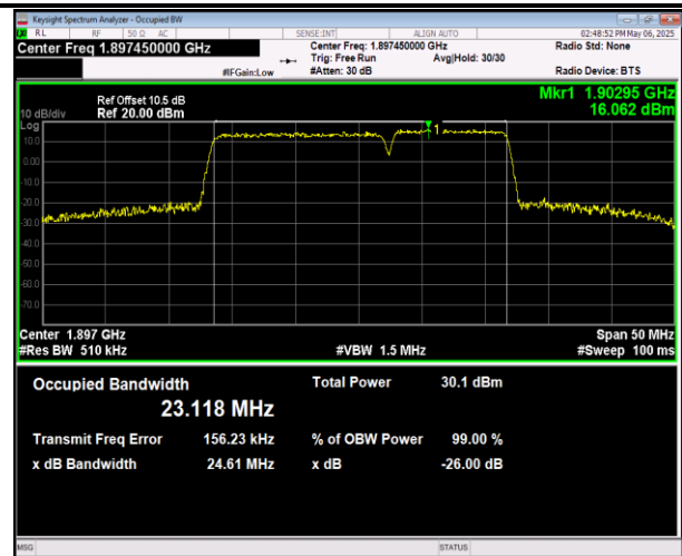
2-2-15MHz-15MHz-16QAM-16QAM-18675-18825-75RB#0-75RB#0-PASS
