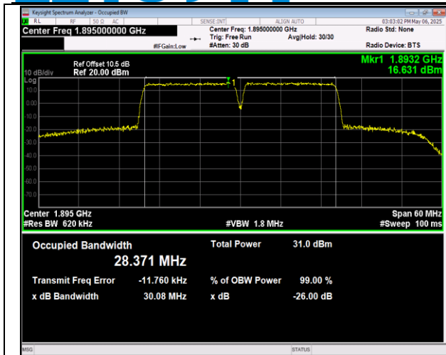
2-2-15MHz-20MHz-QPSK-QPSK-18678-18849-75RB#0-100RB#0-PASS
