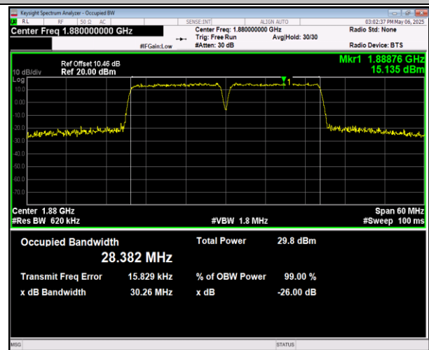
2-2-15MHz-15MHz-16QAM-16QAM-18975-19125-75RB#0-75RB#0-PASS
