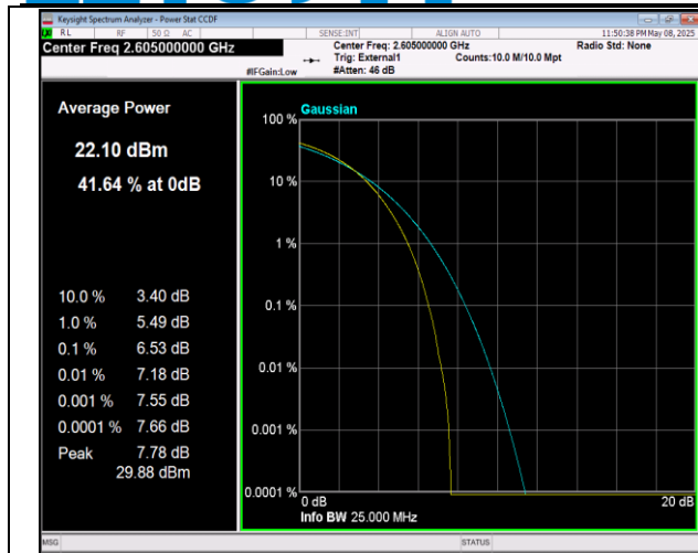
38-38-20MHz-20MHz-QPSK-QPSK-37850-38048-100RB# 0-100RB#0-PASS
