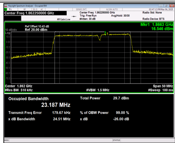
2-2-15MHz-10MHz-16QAM-16QAM-18851-18971-75RB#0-50RB#0-PASS
