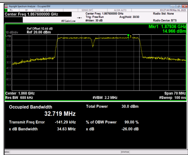
2-2-15MHz-20MHz-16QAM-16QAM-18803-18974-75RB#0-100RB#0-PASS
