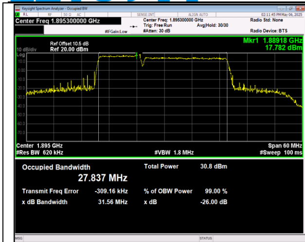
2-2-15MHz-10MHz-QPSK-QPSK-18675-18795-75RB#0-50RB#0-PASS
