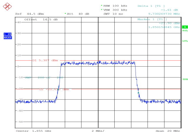
26dB Bandwidth 9.730MHz
