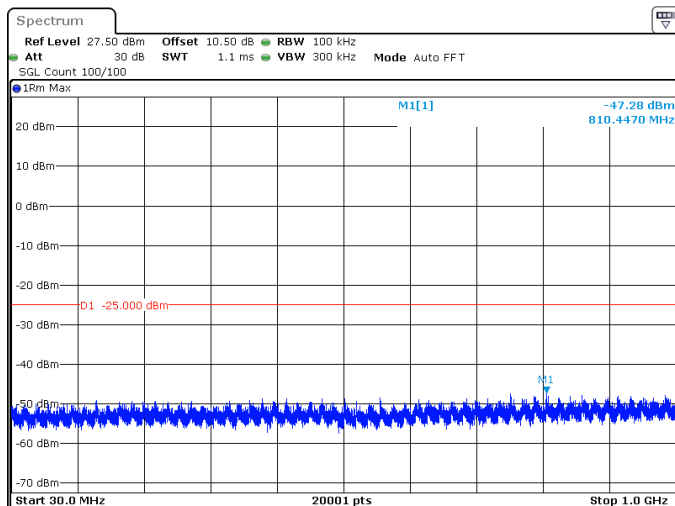
50MHz_15kHz_2664.99MHz_DFT-s-OFDM QPSK_RB270@0 -47.28 dBm
