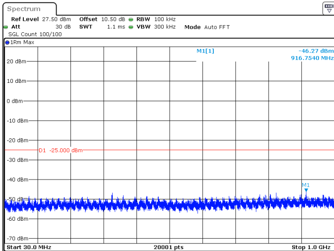
15MHz_15kHz_2503.5MHz_DFT-s-OFDM QPSK_RB1@78 -46.27 dBm
