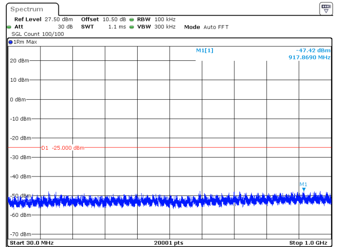
30MHz_30kHz_2592.99MHz_DFT-s-OFDM QPSK_RB1@0 -47.42 dBm
