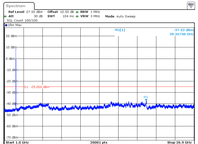
30MHz_15kHz_2511MHz_DFT-s-OFDM QPSK_RB160@0 -37.52 dBm
