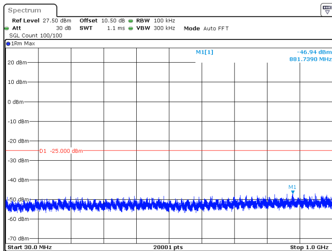
40MHz_15kHz_2516.01MHz_DFT-s-OFDM QPSK_RB1@215 -46.94 dBm
