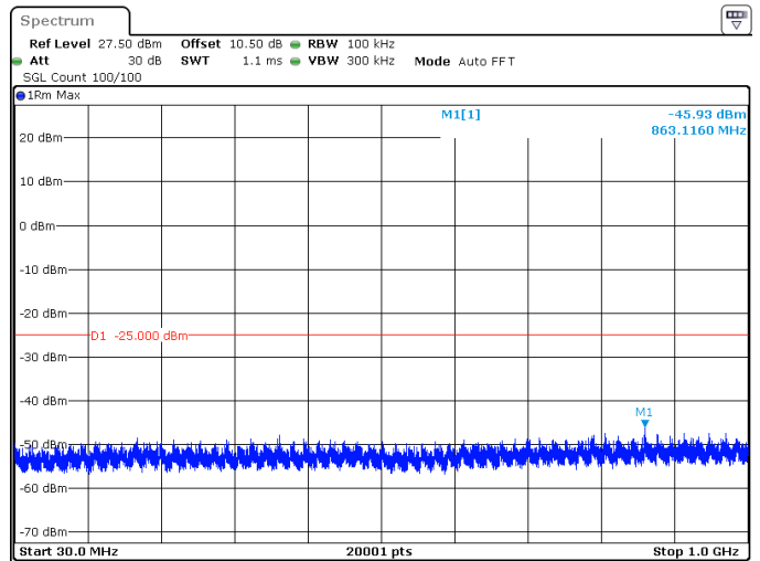
50MHz_15kHz_2593.005MHz_DFT-s-OFDM QPSK_RB1@0 -45.93 dBm
