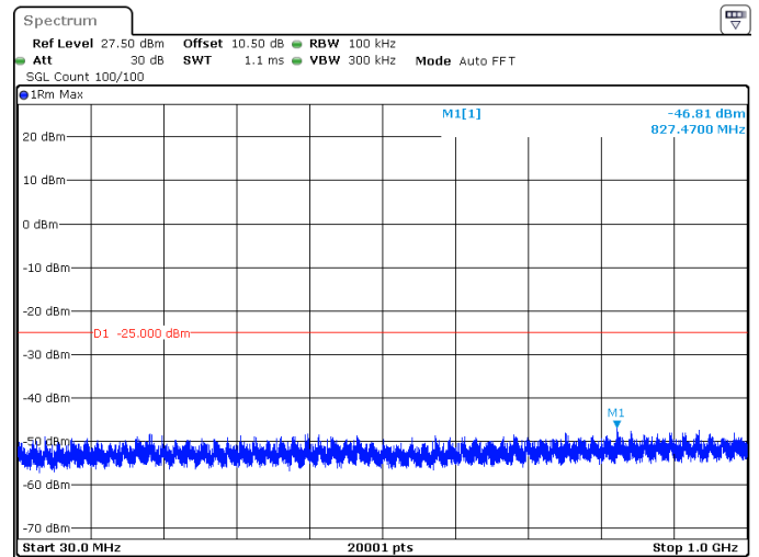
15MHz_30kHz_2592.99MHz_DFT-s-OFDM QPSK_RB1@0 -46.81 dBm
