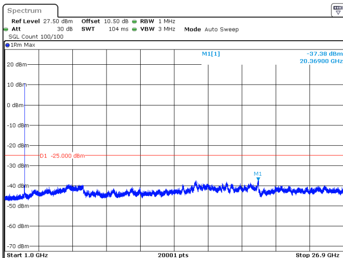
15MHz_15kHz_2503.5MHz_DFT-s-OFDM QPSK_RB75@0 -37.38 dBm
