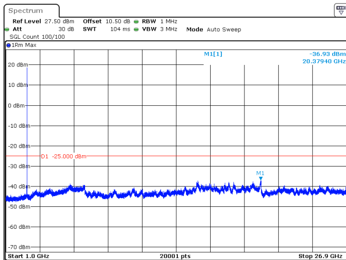
15MHz_30kHz_2592.99MHz_DFT-s-OFDM QPSK_RB1@37 -36.93 dBm
