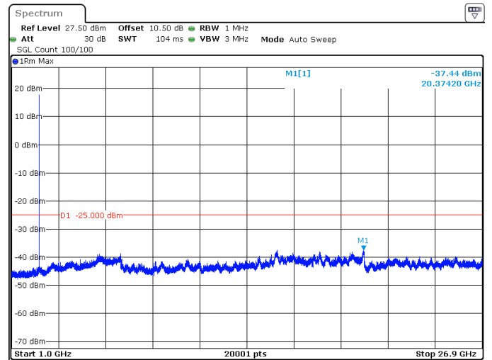
15MHz_30kHz_2503.5MHz_DFT-s-OFDM QPSK_RB1@0 -37.44 dBm
