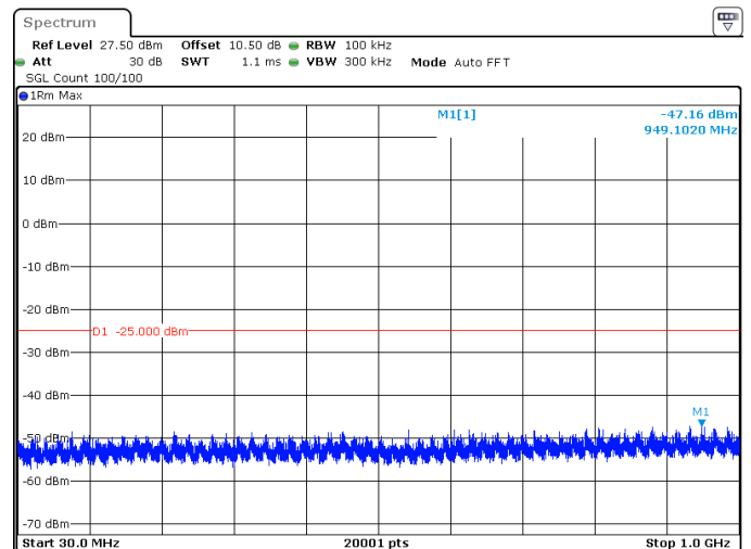
50MHz_30kHz_2521.02MHz_DFT-s-OFDM QPSK_RB128@0 -47.16 dBm
