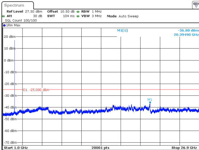
50MHz_30kHz_2521.02MHz_DFT-s-OFDM QPSK_RB1@132 -36.80 dBm
