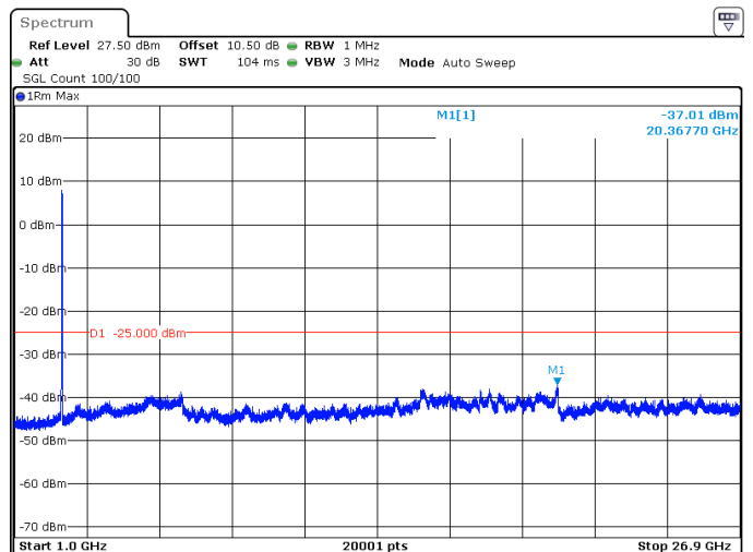
30MHz_15kHz_2674.995MHz_DFT-s-OFDM QPSK_RB160@0 -37.01 dBm
