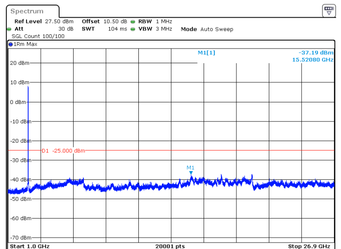
30MHz_30kHz_2592.99MHz_DFT-s-OFDM QPSK_RB75@0 -37.19 dBm
