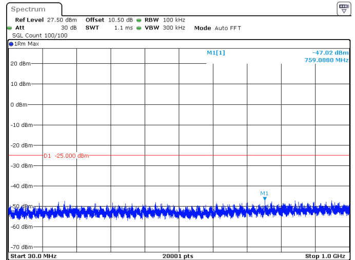
50MHz_30kHz_2521.02MHz_DFT-s-OFDM QPSK_RB1@132 -47.02 dBm
