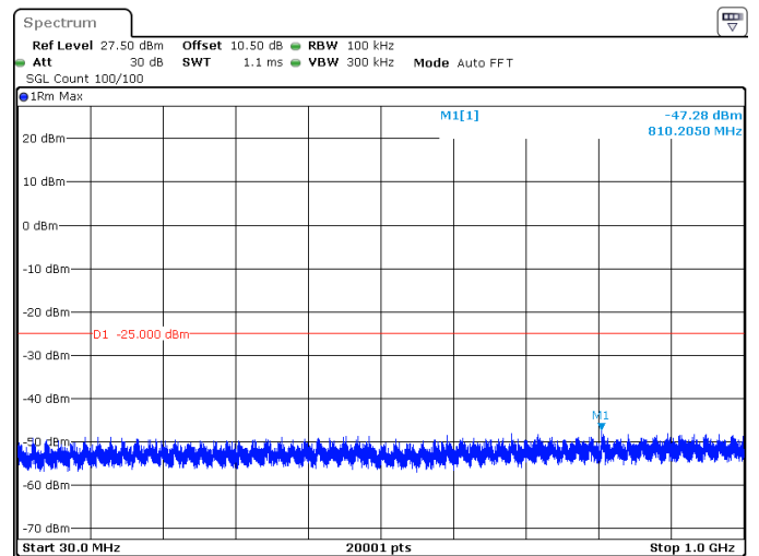
15MHz_30kHz_2503.5MHz_DFT-s-OFDM QPSK_RB1@37 -47.28 dBm
