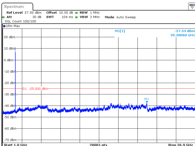
15MHz_15kHz_2682.495MHz_DFT-s-OFDM QPSK_RB75@0 -37.54 dBm
