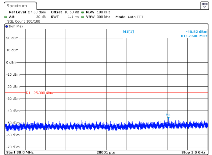
40MHz_15kHz_2516.01MHz_DFT-s-OFDM QPSK_RB1@0 -46.82 dBm
