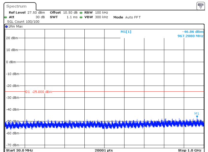
60MHz_30kHz_2526MHz_DFT-s-OFDM QPSK_RB162@0 -46.86 dBm
