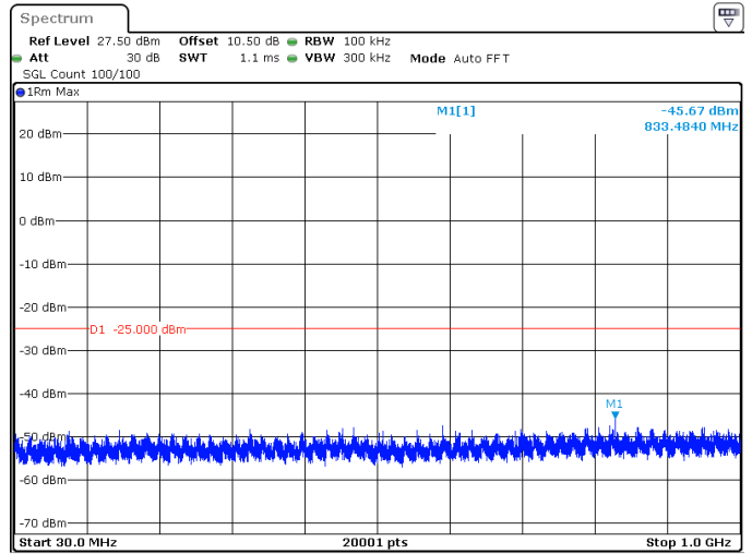
50MHz_15kHz_2521.005MHz_DFT-s-OFDM QPSK_RB1@0 -45.67 dBm
