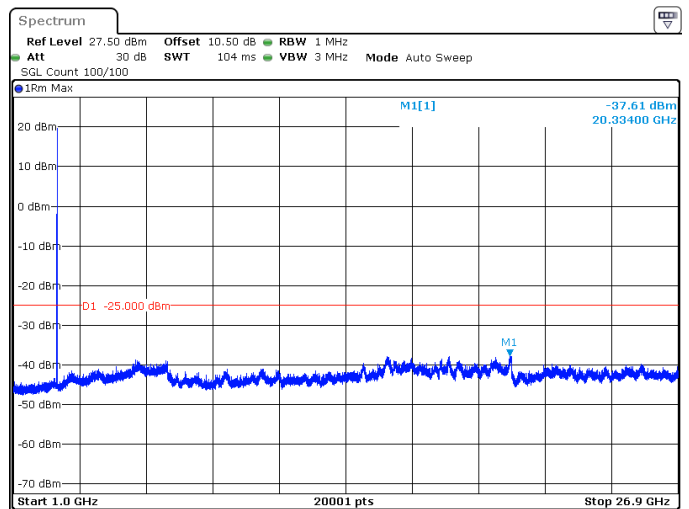
15MHz_15kHz_2682.495MHz_DFT-s-OFDM QPSK_RB1@78 -37.61 dBm
