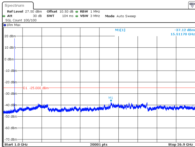
40MHz_30kHz_2516.01MHz_DFT-s-OFDM QPSK_RB1@0 -37.12 dBm
