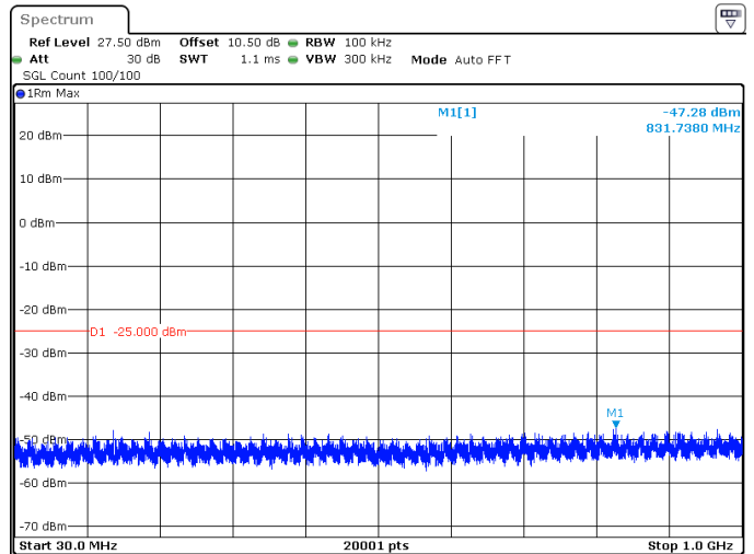
50MHz_15kHz_2593.005MHz_DFT-s-OFDM QPSK_RB1@269 -47.28 dBm
