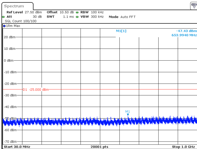
40MHz_30kHz_2592.99MHz_DFT-s-OFDM QPSK_RB1@105 -47.43 dBm
