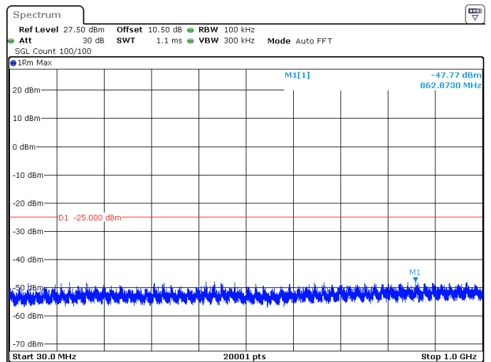
15MHz_15kHz_2593.005MHz_DFT-s-OFDM QPSK_RB1@78 -47.77 dBm
