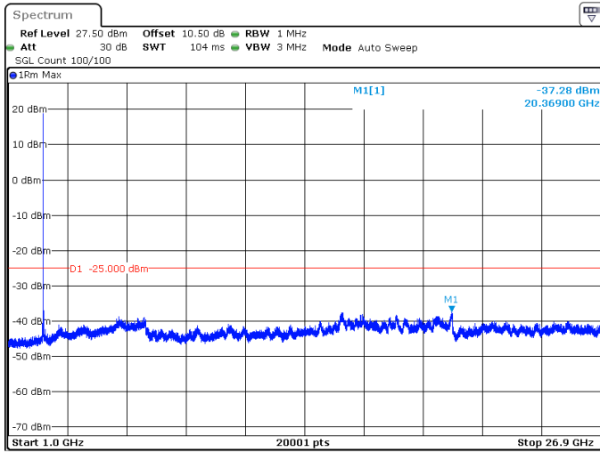
50MHz_15kHz_2521.005MHz_DFT-s-OFDM QPSK_RB1@0 -37.28 dBm
