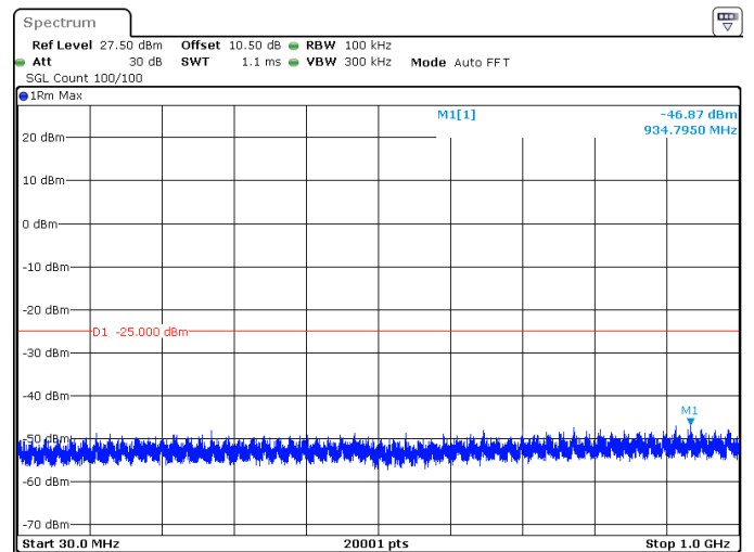
30MHz_30kHz_2511MHz_DFT-s-OFDM QPSK_RB1@77 -46.87 dBm
