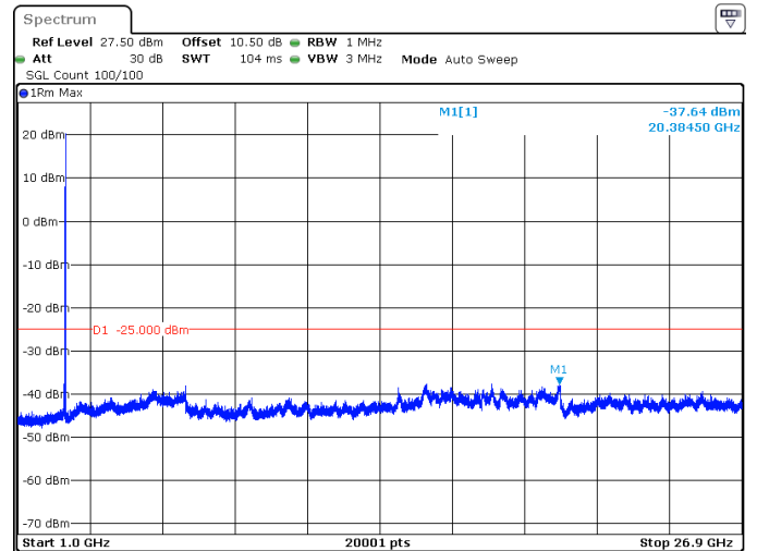
50MHz_15kHz_2664.99MHz_DFT-s-OFDM QPSK_RB1@269 -37.64 dBm
