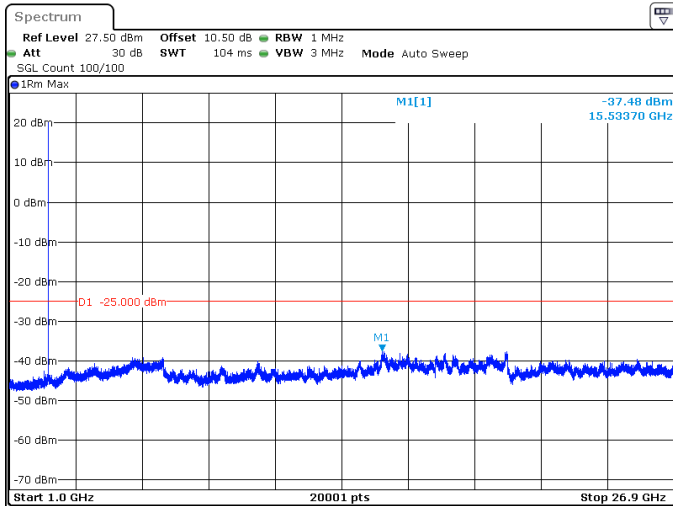
15MHz_15kHz_2503.5MHz_DFT-s-OFDM QPSK_RB1@0 -37.48 dBm
