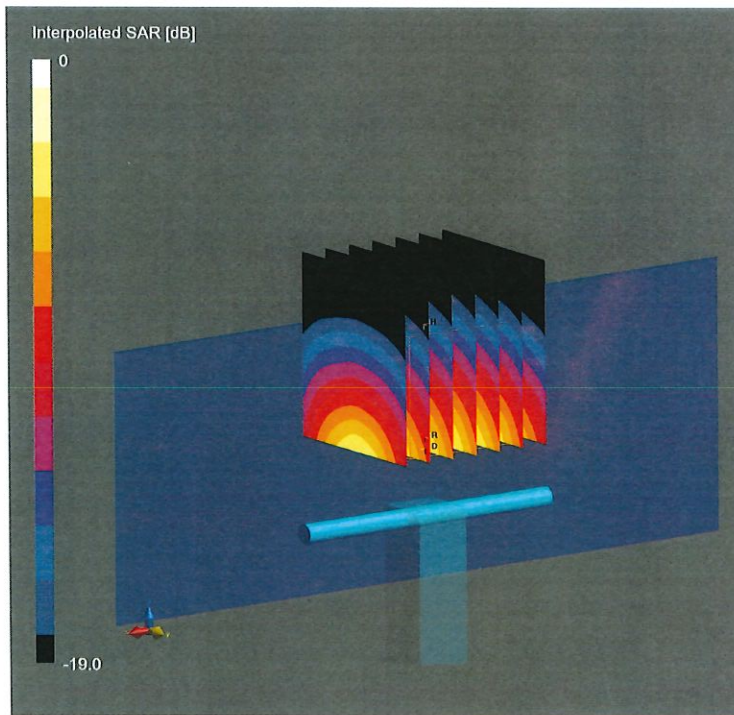
0 dB = 29.0 W/Kg
