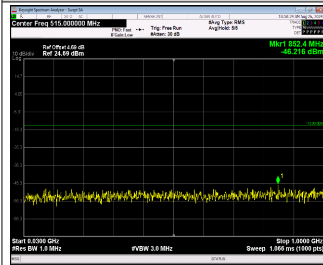
Band4-1.4MHz-QPSK-20175-1RB#0-Range1:30~100 OMHz
