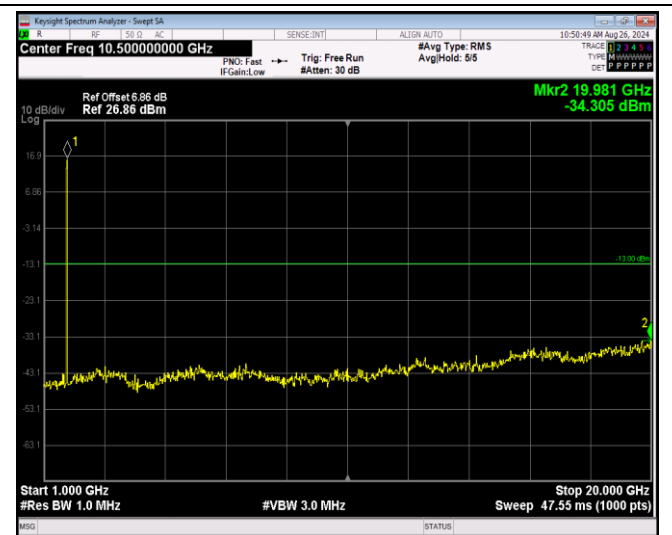
Band4-1.4MHz-16QAM-20393-1RB#0-Range2:1000~20000MHz
