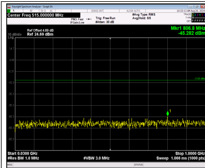
Band4-1.4MHz-QPSK-19957-1RB#0-Range1:30~100 OMHz
