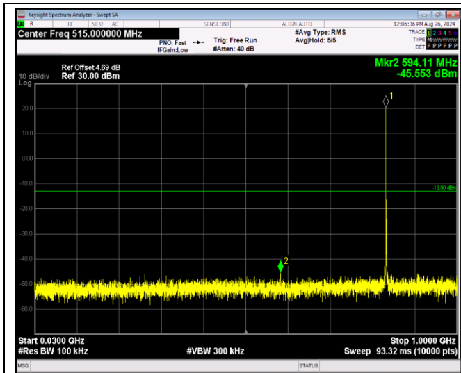
Band5-1.4MHz-QPSK-20643-1RB#0-Range1:30~100 OMHz
