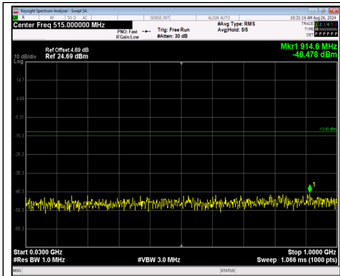
Band2-20MHz-16QAM-18900-1RB#0-Range1:30~100 0MHz
