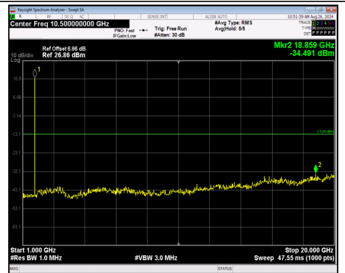
Band4-1.4MHz-64QAM-19957-1RB#0-Range2:1000~20000MHz
