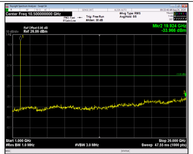
Band2-1.4MHz-64QAM-19193-1RB#0-Range2:1000~20000MHz
