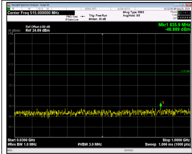
Band2-20MHz-16QAM-19100-1RB#0-Range1:30~100 0MHz
