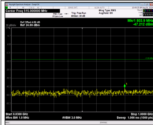
Band4-1.4MHz-QPSK-20175-1RB#0-Range1:30~100 OMHz
