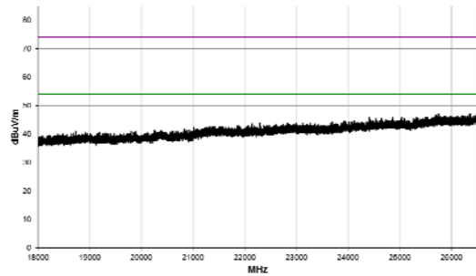
18 GHz – 26.5 GHz
