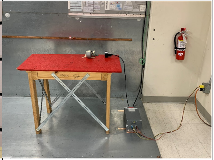
Conducted Emissions
