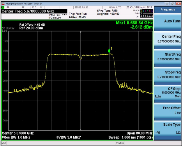
11AC40SISO-Ant1-5670-PASS
