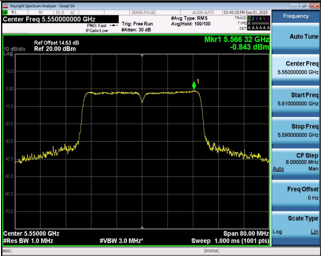
11AC40SISO-Ant1-5550-PASS
