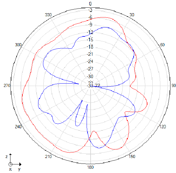
Phi=90 freq=2340MHz
