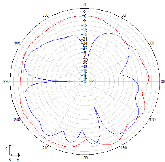
Phi=90 freq=2580MHz
