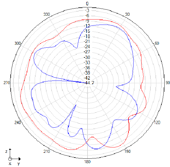
Phi=90 freq=2380MHz
