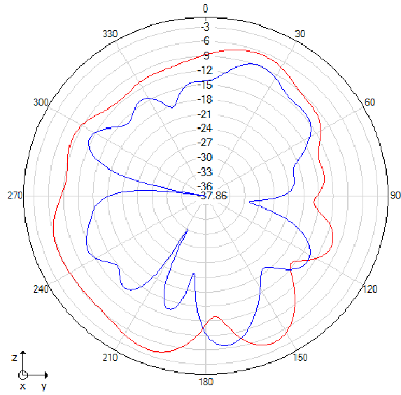
Phi=90 freq=2360MHz
