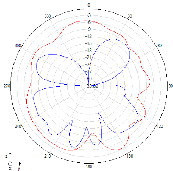
Phi=90 freq=2540MHz
