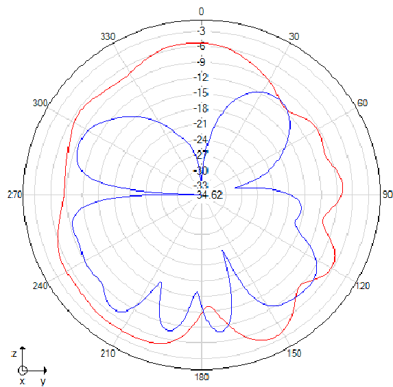
Phi=90 freq=2560MHz
