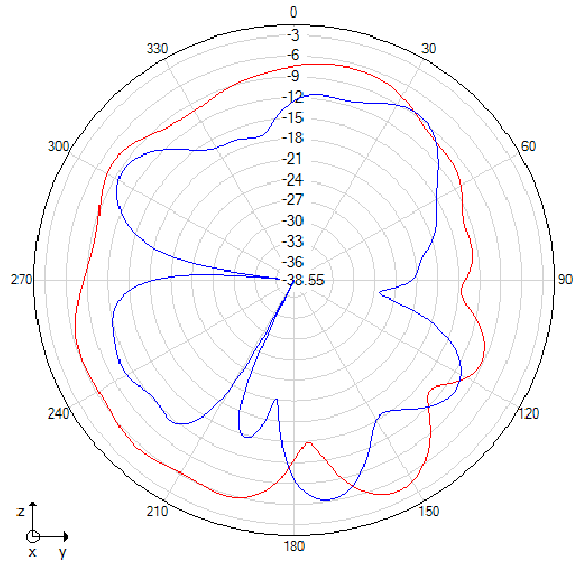
Phi=90 freq=2400MHz
