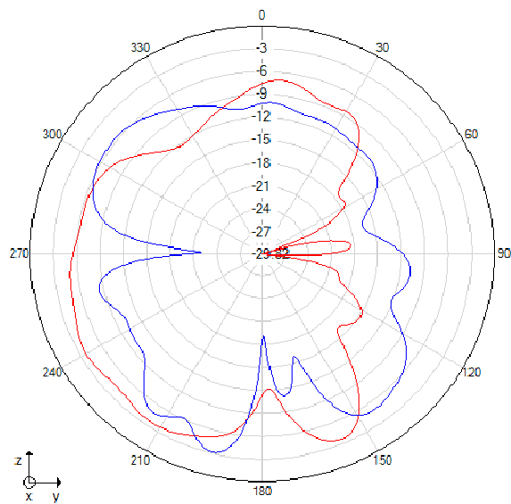
Phi=90 freq=2680MHz
