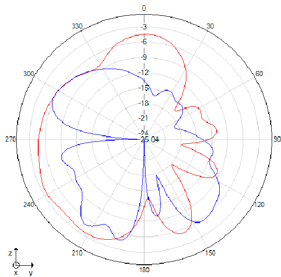
Phi=90 freq=2640MHz
