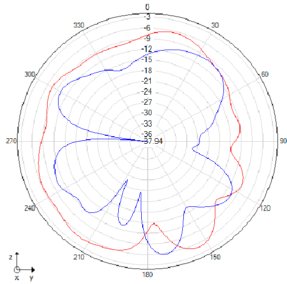
Phi=90 freq=2420MHz
