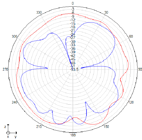
Phi=90 freq=2520MHz
