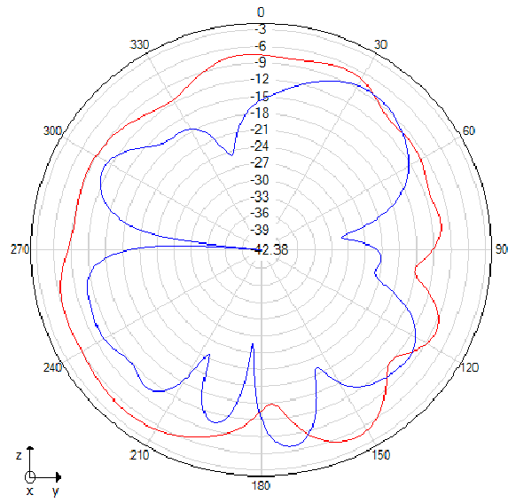
Phi=90 freq=2460MHz
