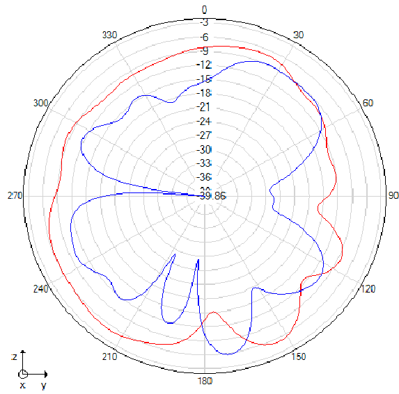
Phi=90 freq=2440MHz
