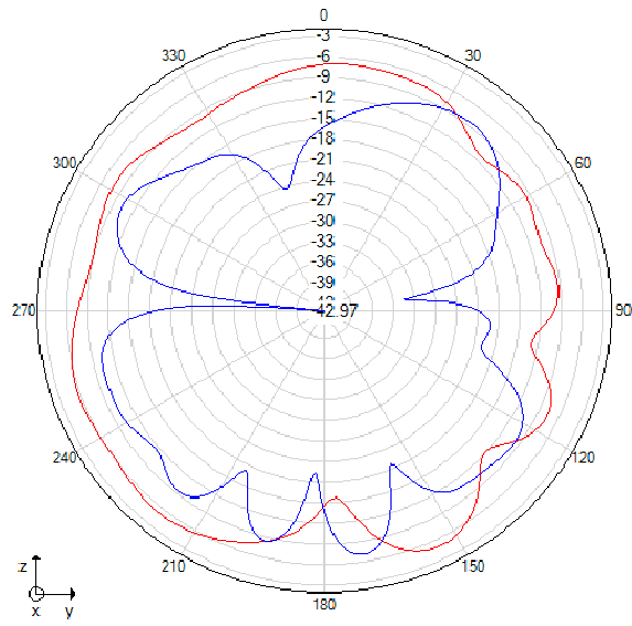
Phi=90 freq=2480MHz
