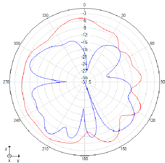
Phi=90 freq=2600MHz
