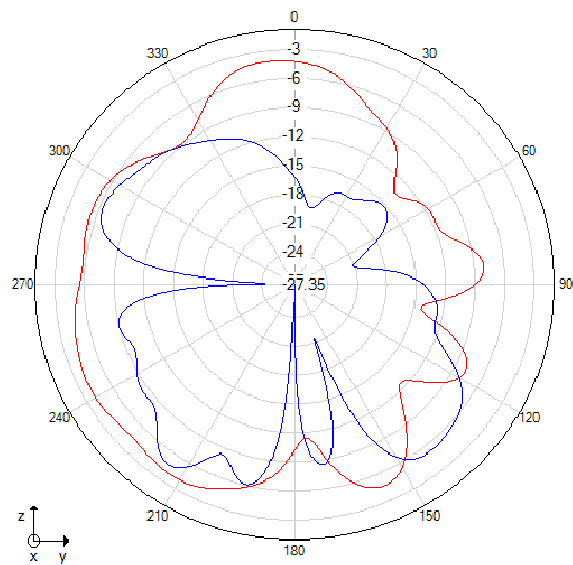
Phi=90 freq=2620MHz
