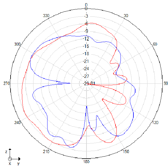
Phi=90 freq=2660MHz
