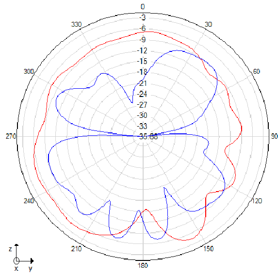
Phi=90 freq=2500MHz
