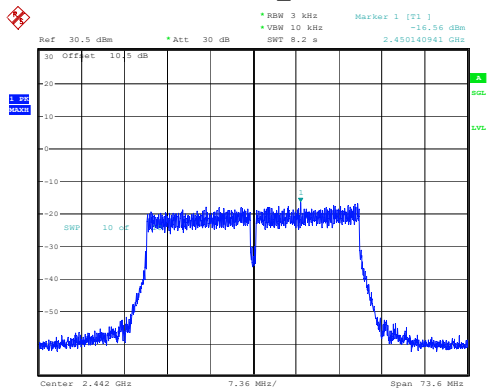
802.11n40_2442MHz
