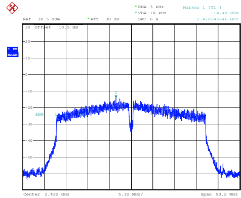
802.11n40_2422MHz
