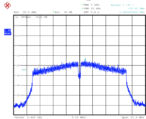
802.11n40_2462MHz
