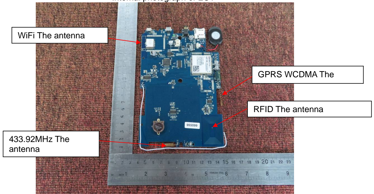
Internal photograph of EUT
