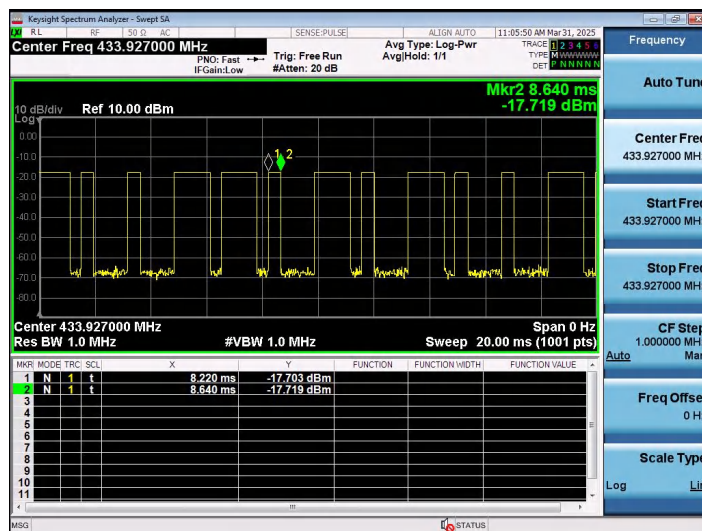
(Time per burst: 0.42ms*16pcs)
