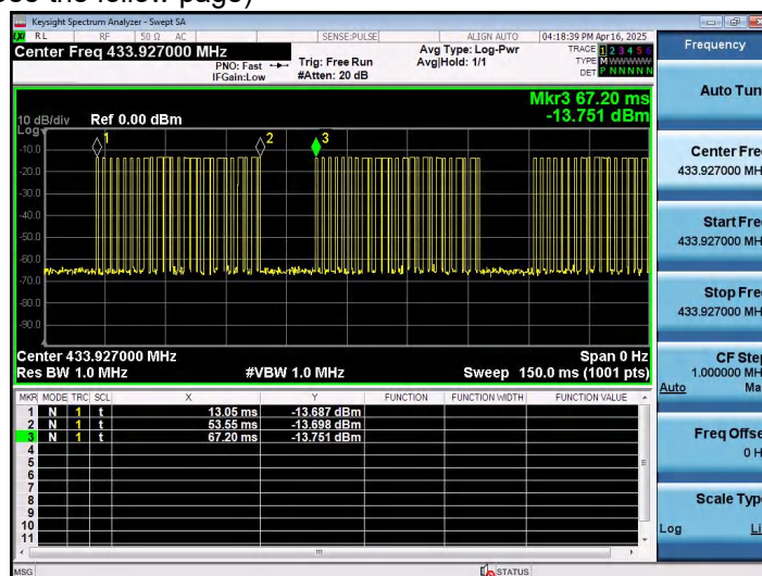
(Transmit cycle 54.6ms)
