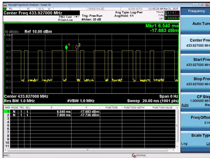
(Time per burst: 1.26ms*9pcs)
