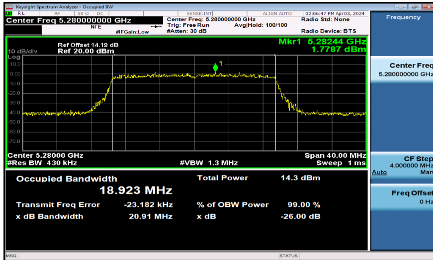
11AX20SISO-Ant1-5280
