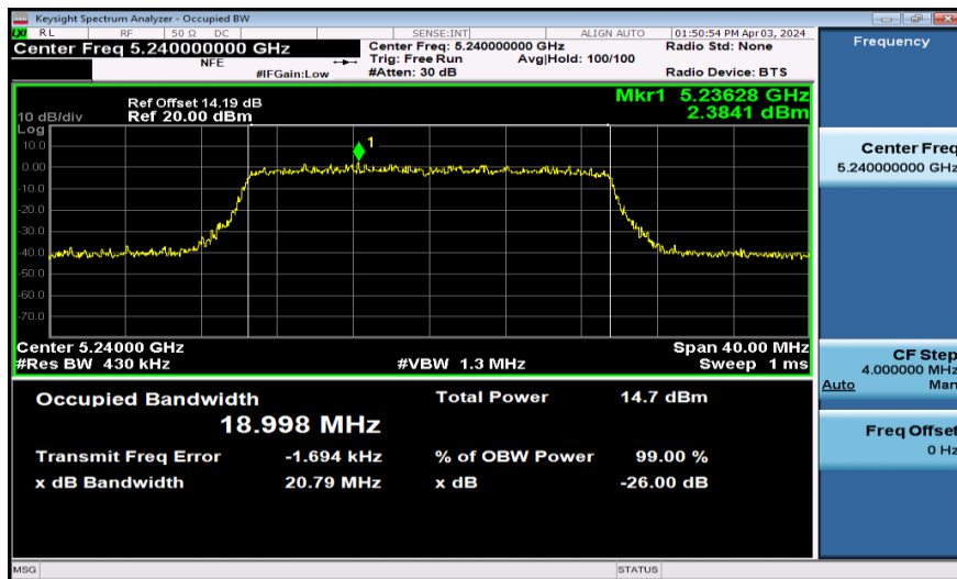
11AX20SISO-Ant1-5240
