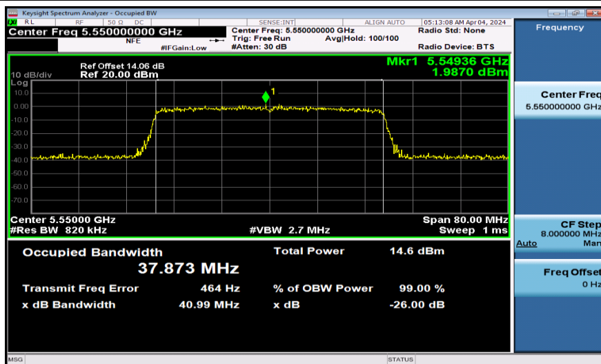
11AX40SISO-Ant1-5550
