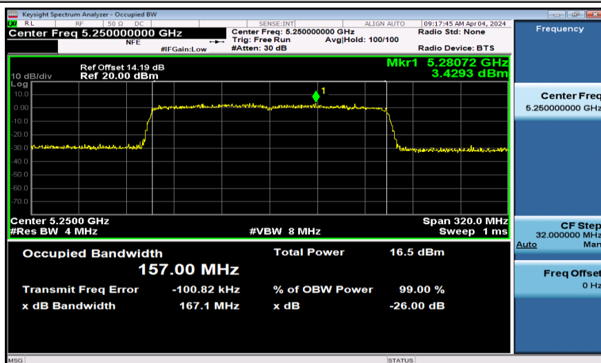
11AX160SISO-Ant1-5250
