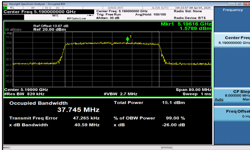
11AX40SISO-Ant1-5190
