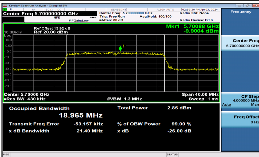
11AX20SISO-Ant1-5700
