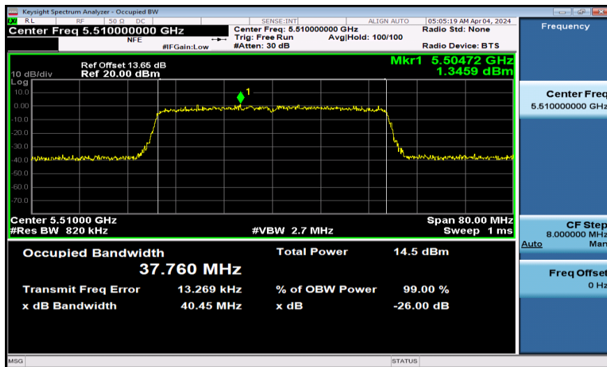
11AX40SISO-Ant1-5510
