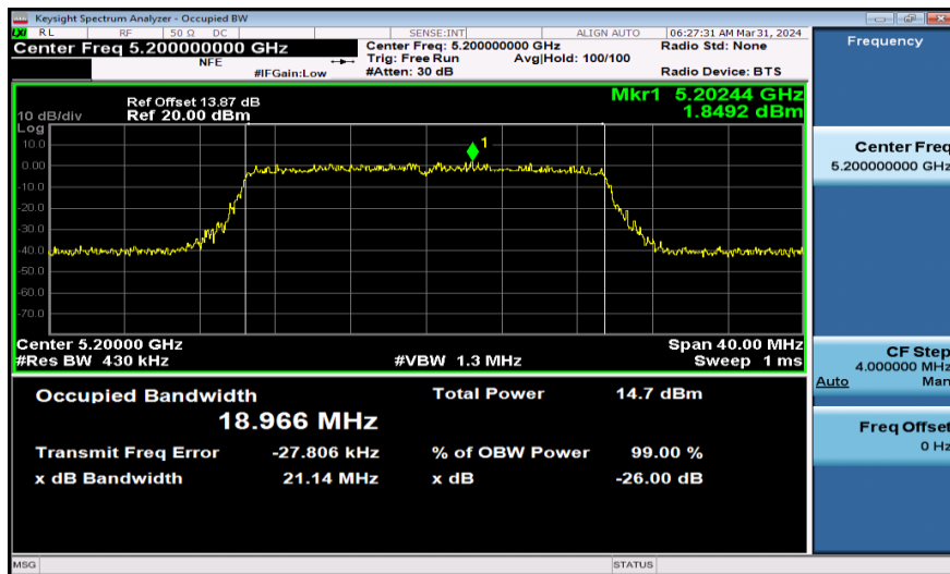
11AX20SISO-Ant1-5200-242Tone
