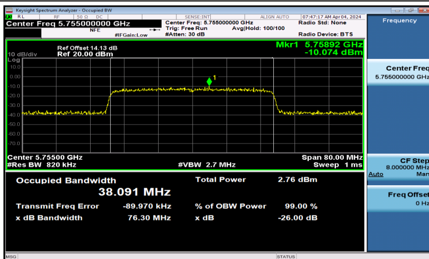
11AX40SISO-Ant1-5755
