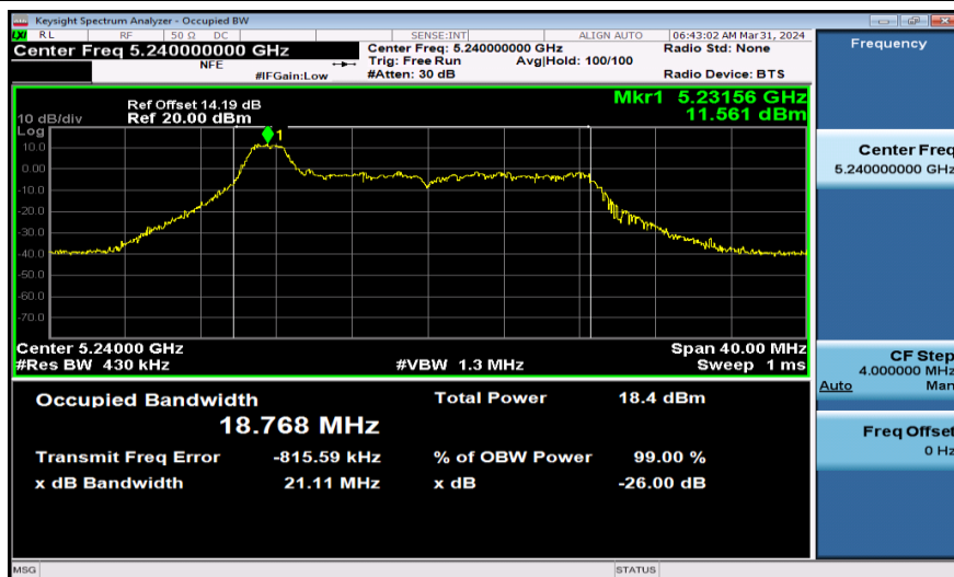
11AX20SISO-Ant1-5240-26Tone
