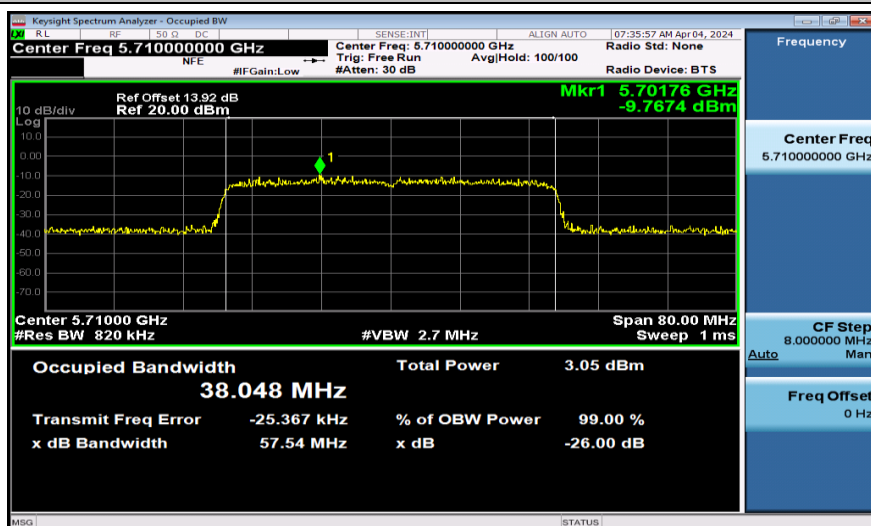
11AX40SISO-Ant1-5710
