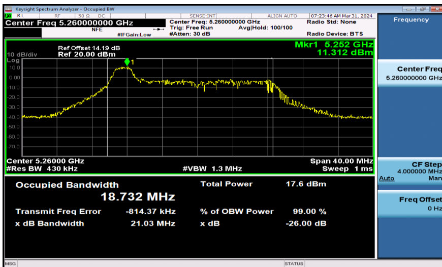
11AX20SISO-Ant1-5260-26Tone
