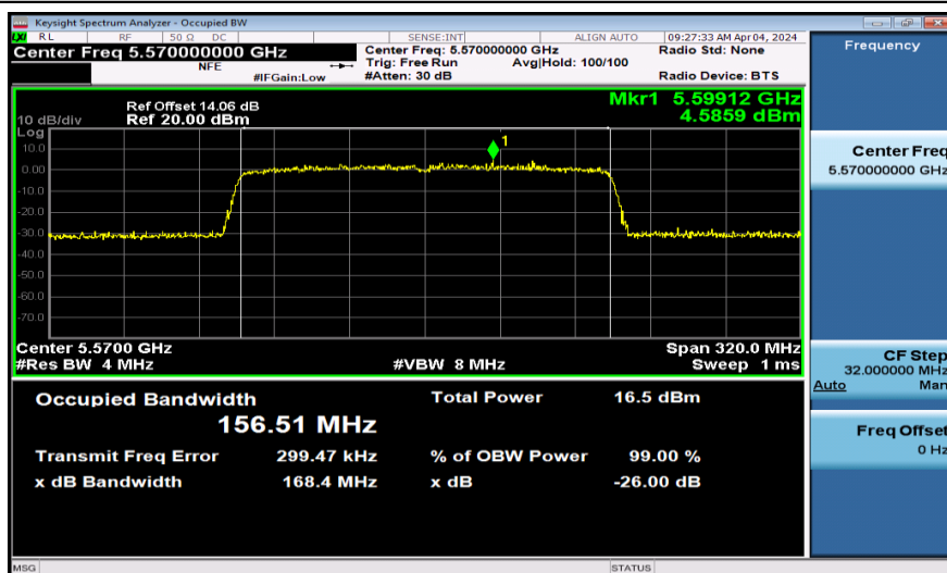
11AX160SISO-Ant1-5570
