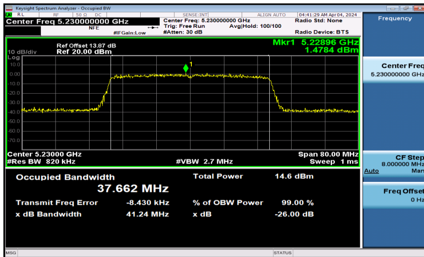
11AX40SISO-Ant1-5230
