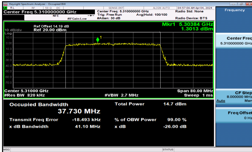
11AX40SISO-Ant1-5310
