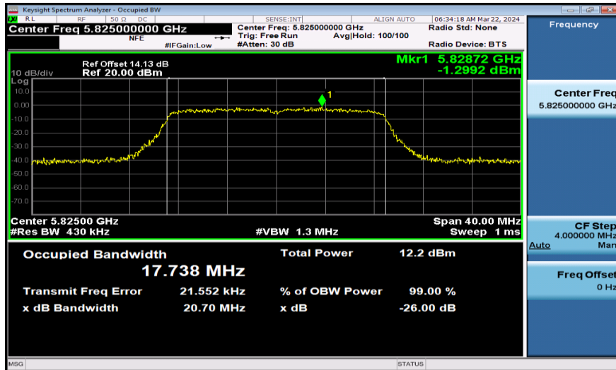
11AC20SISO-Ant1-5825
