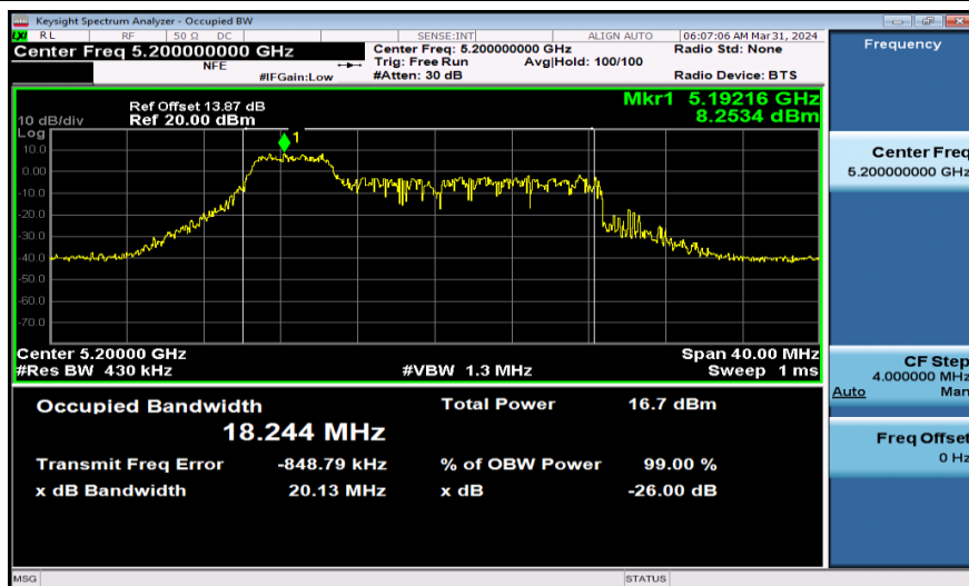
11AX20SISO-Ant1-5200-52Tone
