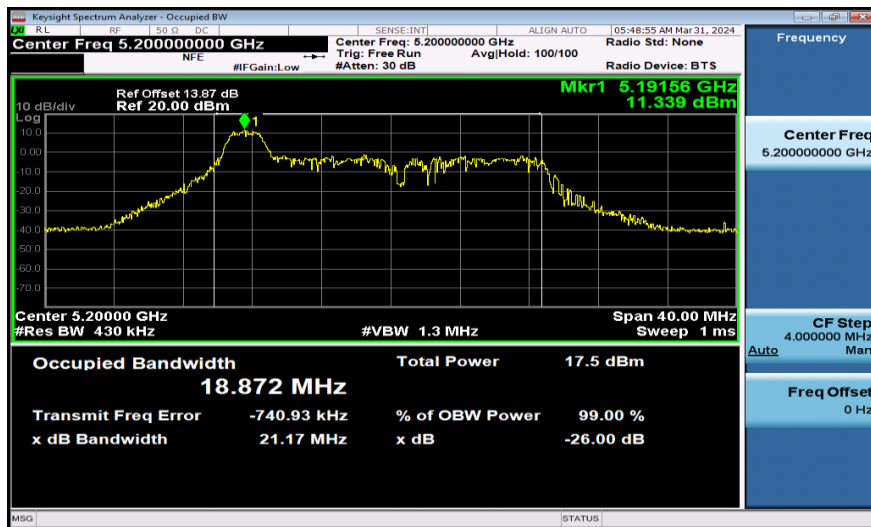
11AX20SISO-Ant1-5200-26Tone
