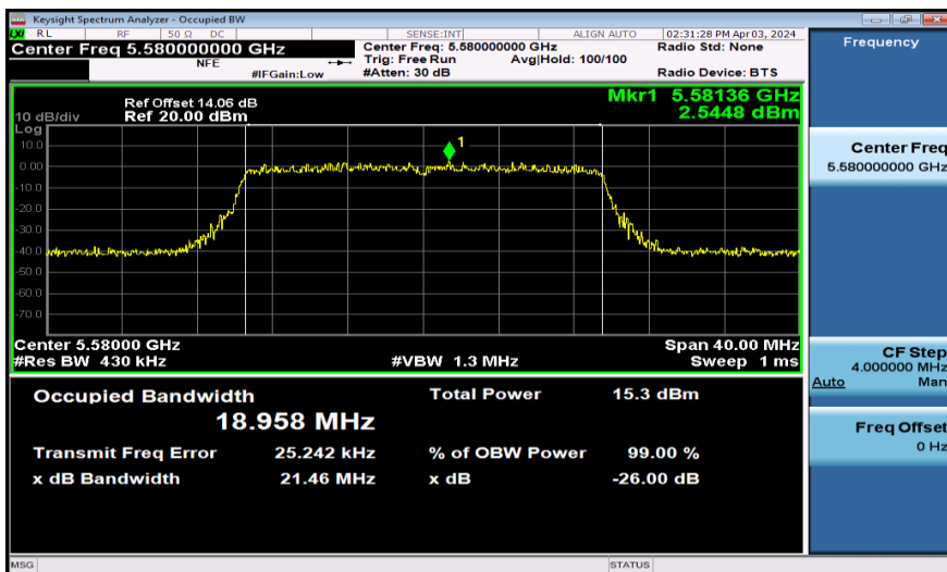
11AX20SISO-Ant1-5580
