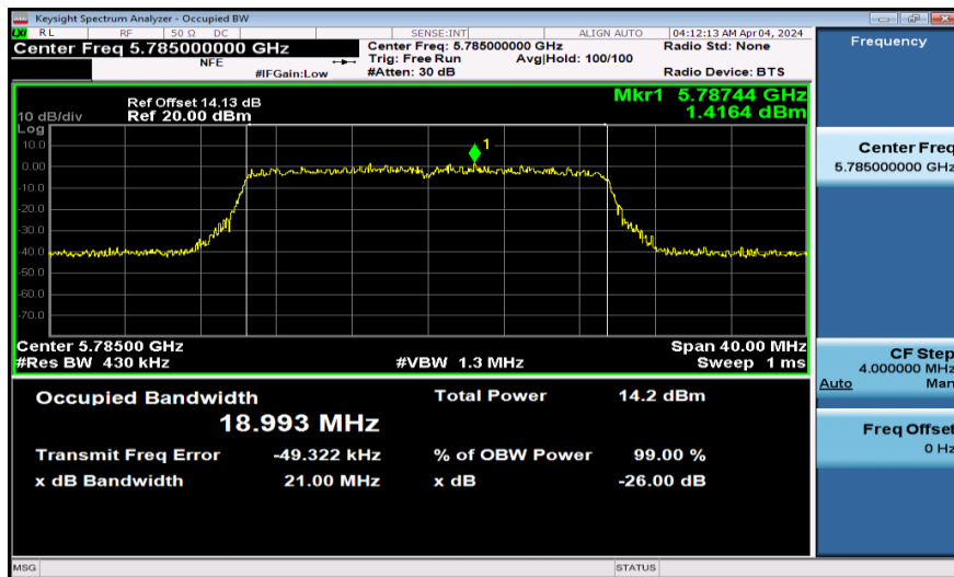
11AX20SISO-Ant1-5785
