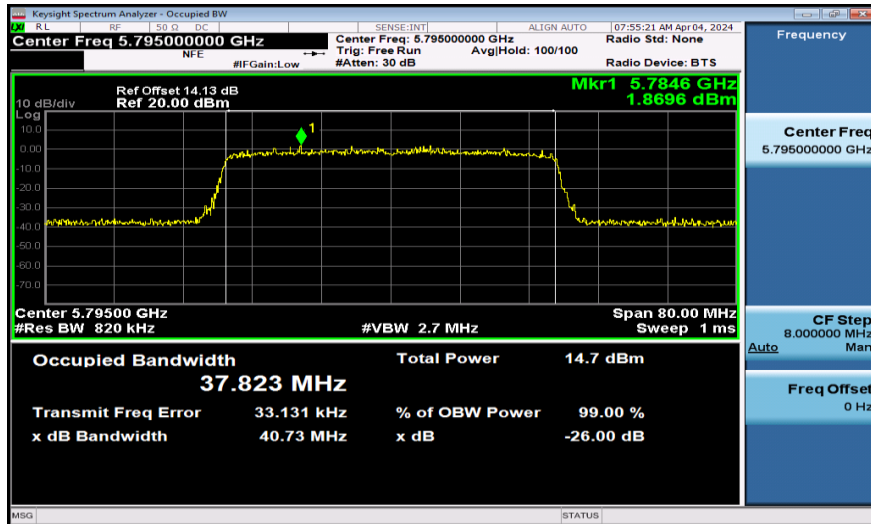
11AX40SISO-Ant1-5795
