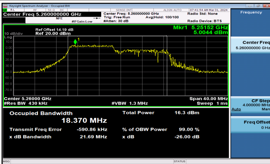
11AX20SISO-Ant1-5260-106Tone
