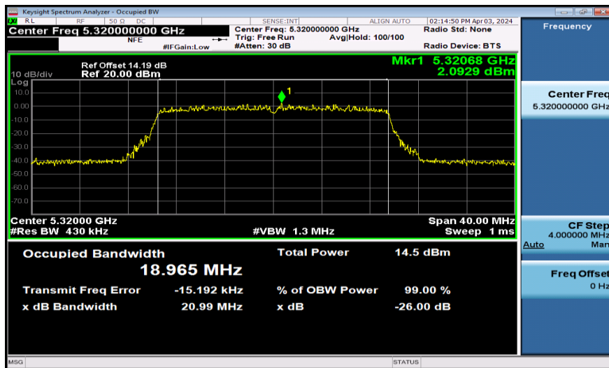
11AX20SISO-Ant1-5320
