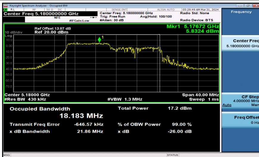
11AX20SISO-Ant1-5180-106Tone
