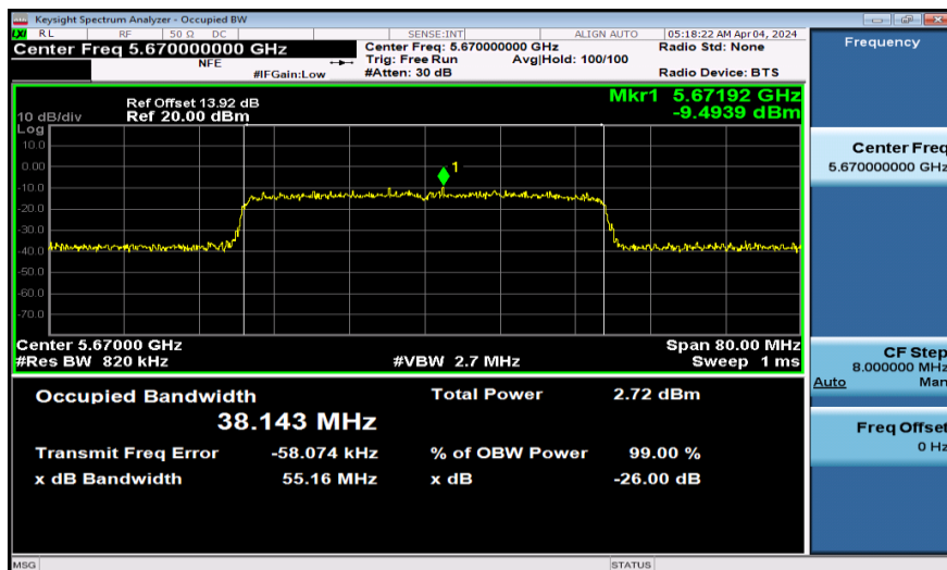
11AX40SISO-Ant1-5670
