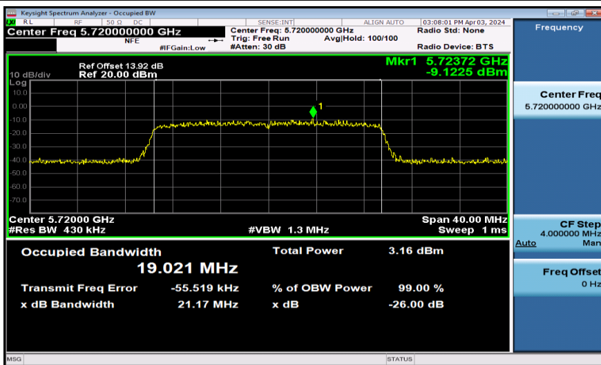
11AX20SISO-Ant1-5720
