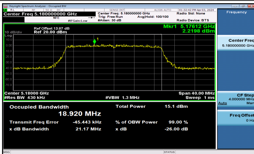
11AX20SISO-Ant1-5180
