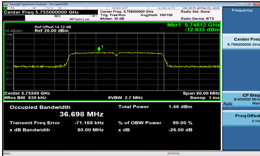
11AC40SISO-Ant1-5755
