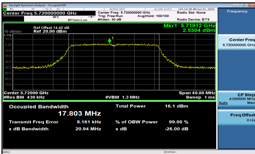
11AC20SISO-Ant1-5720
