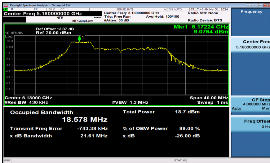
11AX20SISO-Ant1-5180-52Tone
