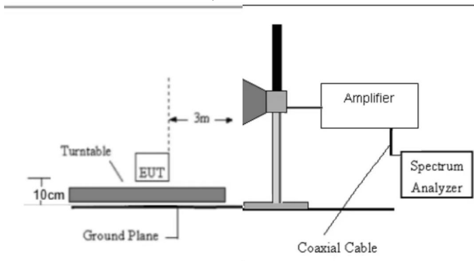
(C) Radiated Emission Test-Up Frequency Above 1GHz
