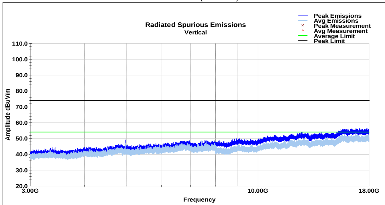
BLE Channel 39 Vertical Plot (3-18GHz)
