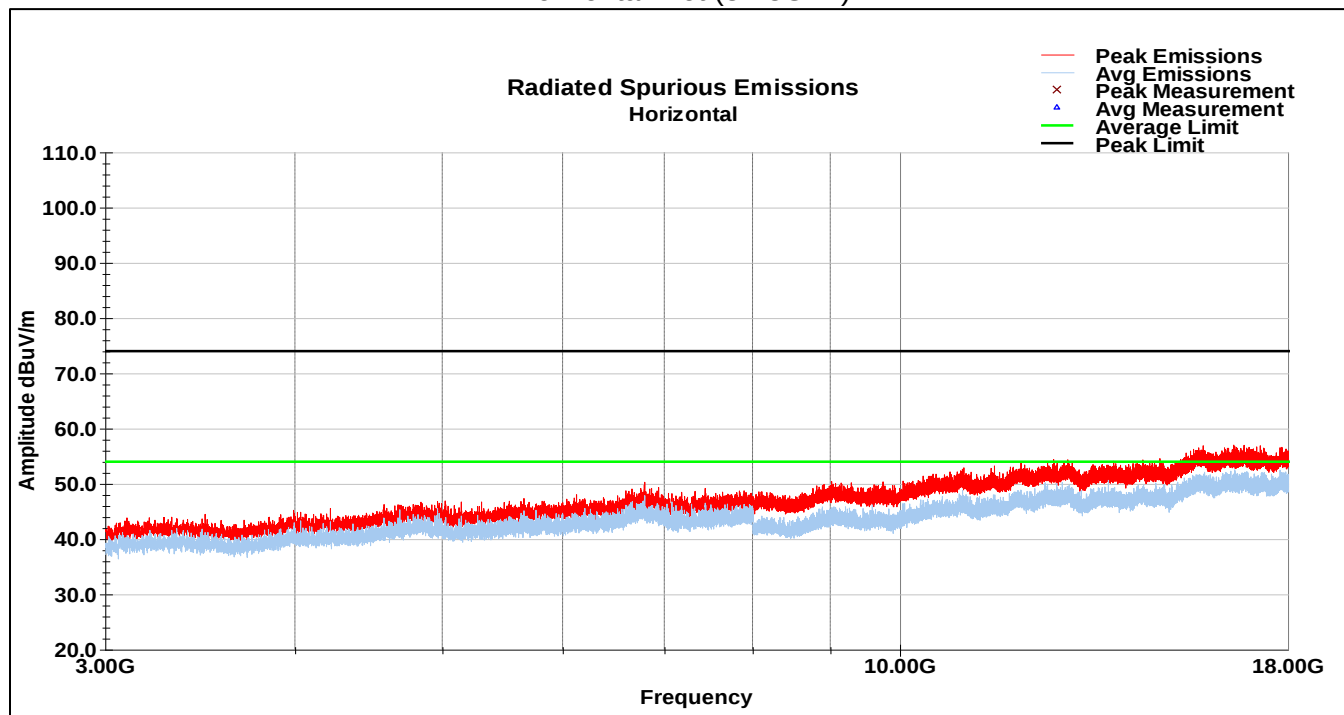
BLE Channel 39 Horizontal Plot (3-18GHz)
