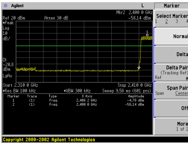
BDR mode ( \pi/4 -DQPSK): Band Edge-Low Channel (Hopping Mode)
