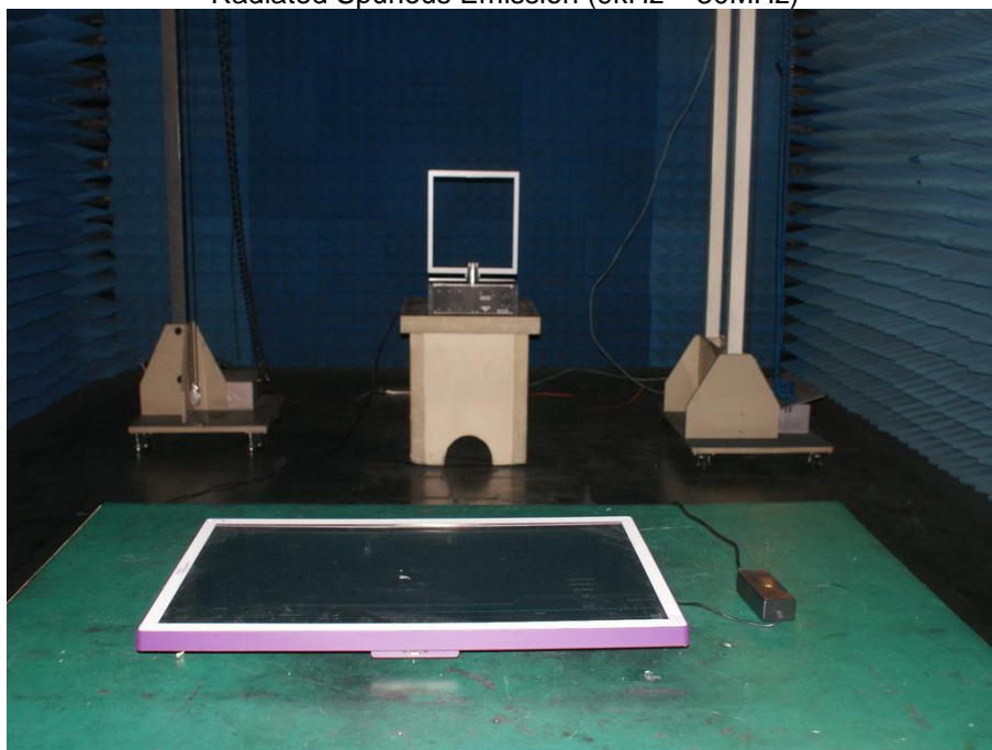
Radiated Spurious Emission (9kHz ~ 30MHz)
