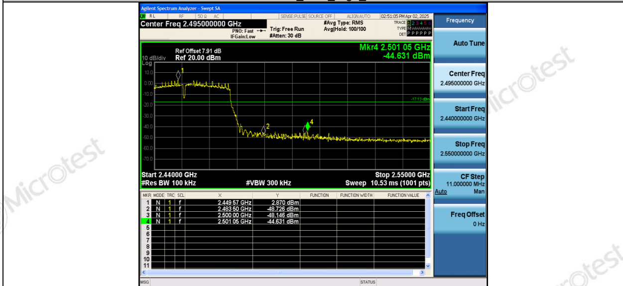
11N40SISO_Ant1_High_2452
