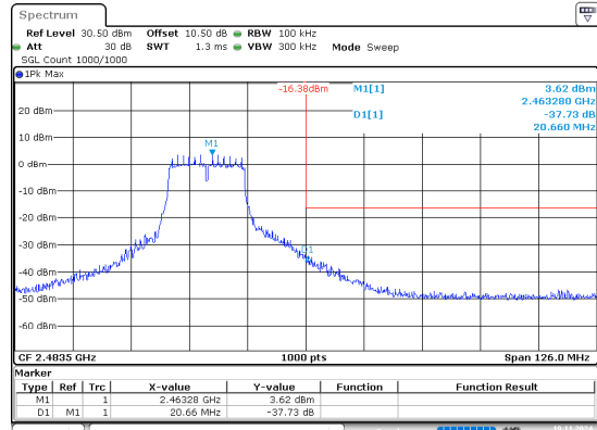
802.11g_2462MHz
