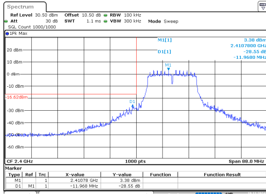
802.11g_2412MHz
