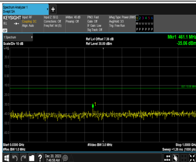
Band2-5MHz-QPSK-18625-1RB#0-Range1:30~1000MHz
