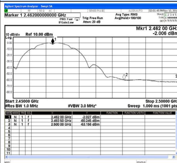
802.11b-High channel(Average)
