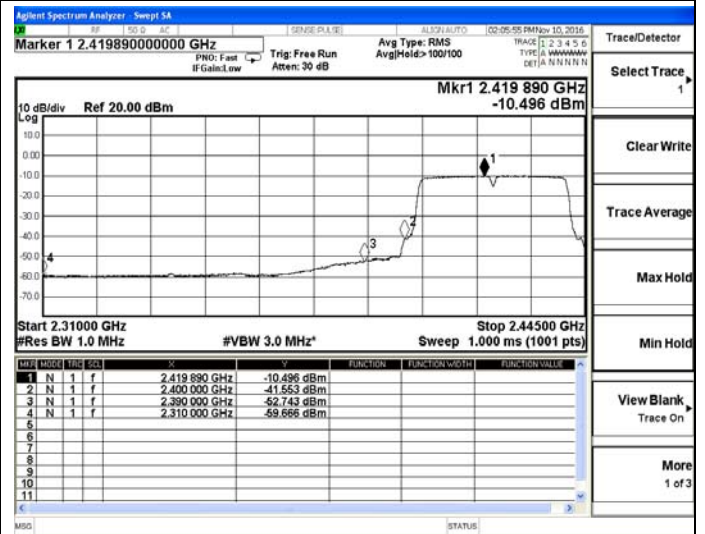
802.11n(HT40)-Low channel(Average)
