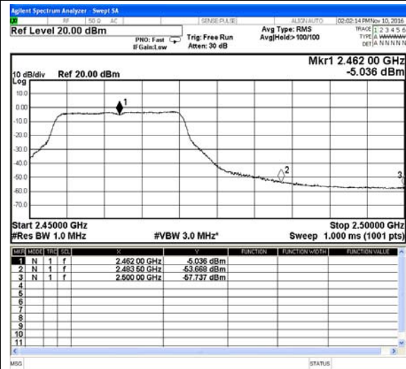
802.11g-High channel(Average)
