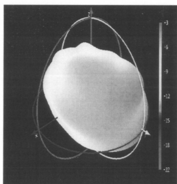
Phi=90 freq=2450MHz
