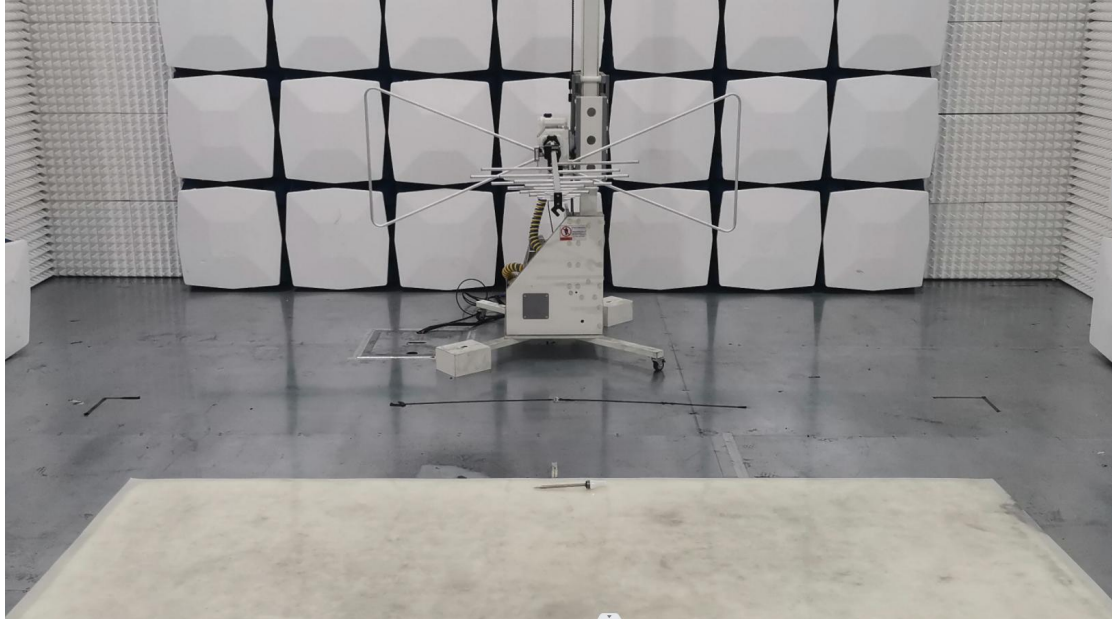
RADIATED EMISSION MEASUREMENT (below 1G)
