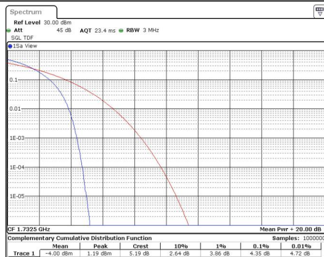
Band4-10MHz-QPSK-20175-1RB#0
