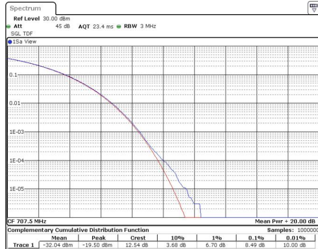
Band12-1.4MHz-16QAM-23095-6RB#0
