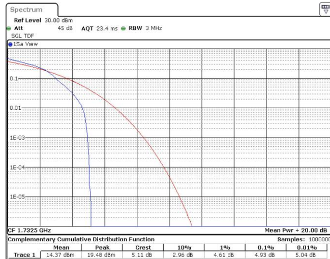
Band4-5MHz-16QAM-20175-25RB#0
