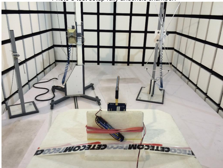
Photo 3 test setup fully anechoic chamber:
