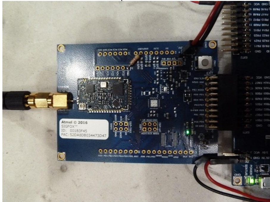
Photo 7 test setup semi anechoic chamber:
