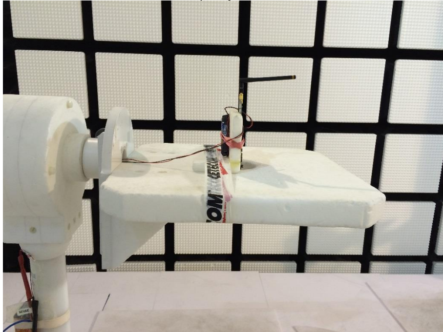
Photo 1 test setup fully anechoic chamber:
