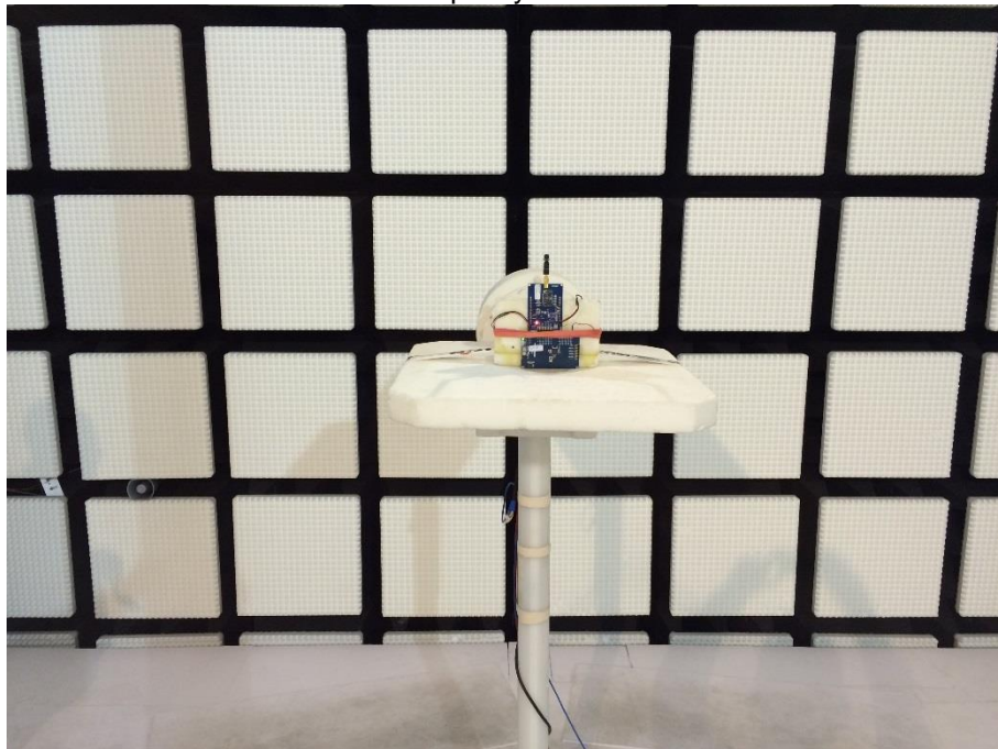
Photo 2 test setup fully anechoic chamber:
