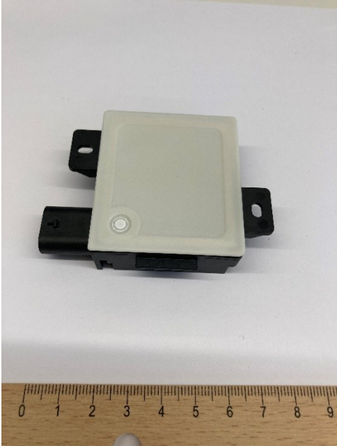
Top Side (Radar Cover with applicated Membrane)
