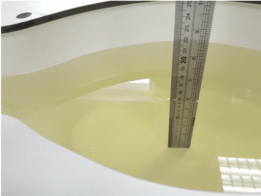
Photograph of the depth in the flat Phantom (835MHz, 15.0cm depth)
