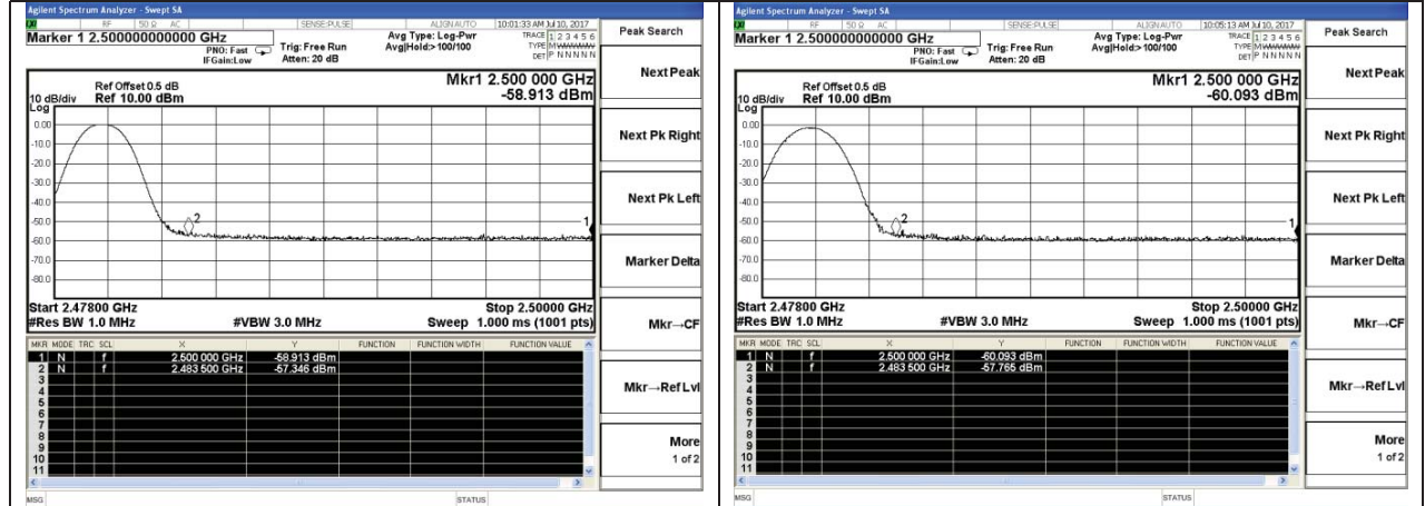
Channel 78 / 2480 MHz – Non-Hopping – Peak
