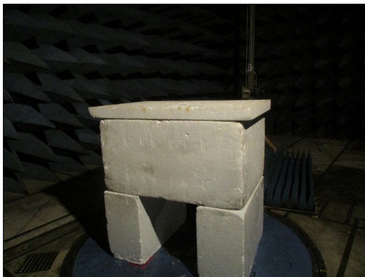
Figure 12: Radiated Emissions above 1 GHz – Back View – EUT Flat
