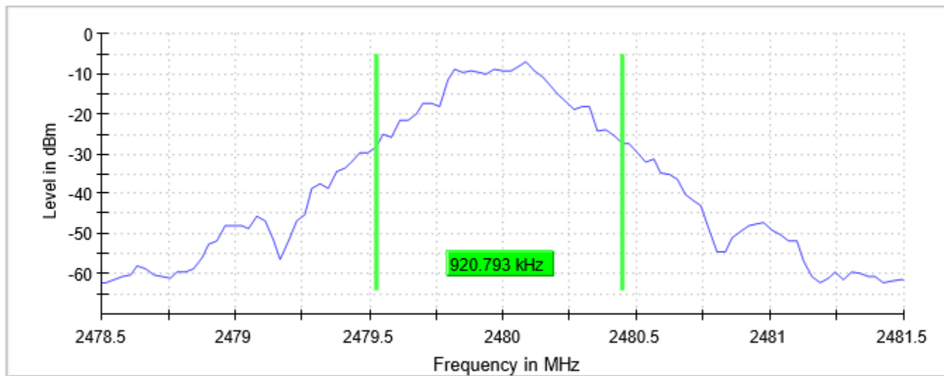
20 dB Bandwidth
