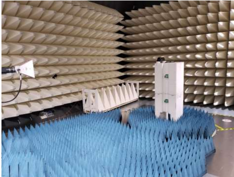
9. High Range Radiated Emission test setup
