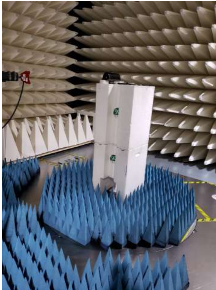
10. High Range Radiated Emission test setup 2
