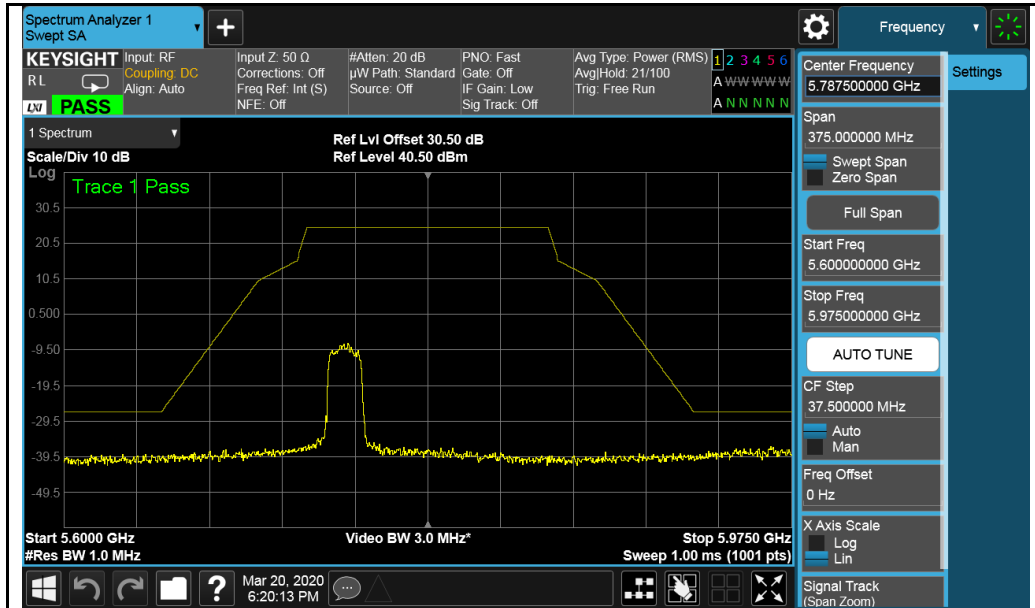
802.11a-5745MHz
