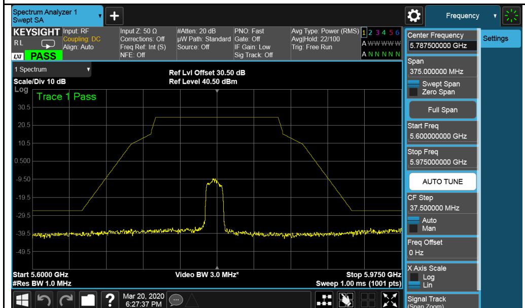
802.11a-5785MHz
