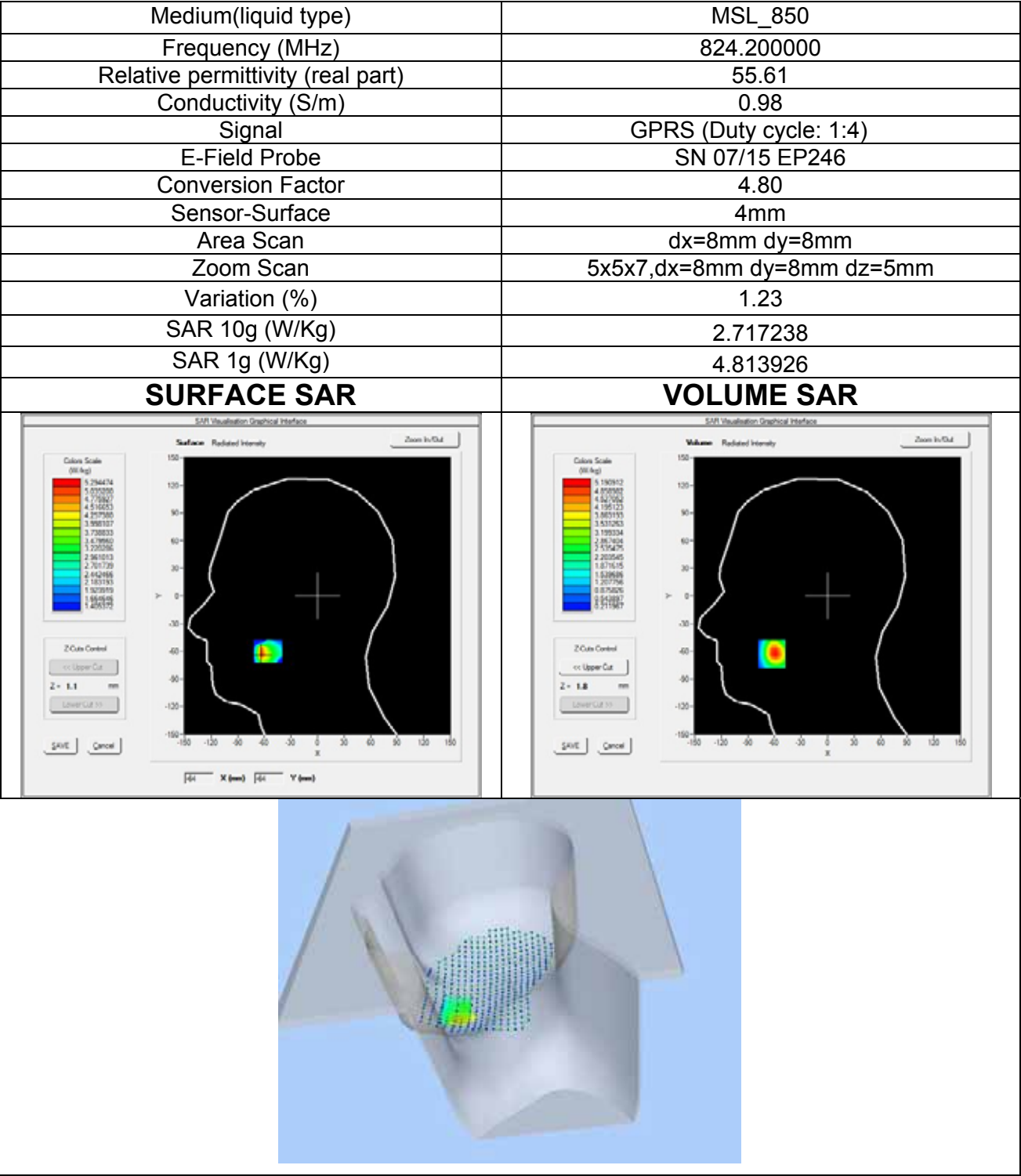
Plot 4: Right Head with Back side device position on Low Channel in GSM mode
