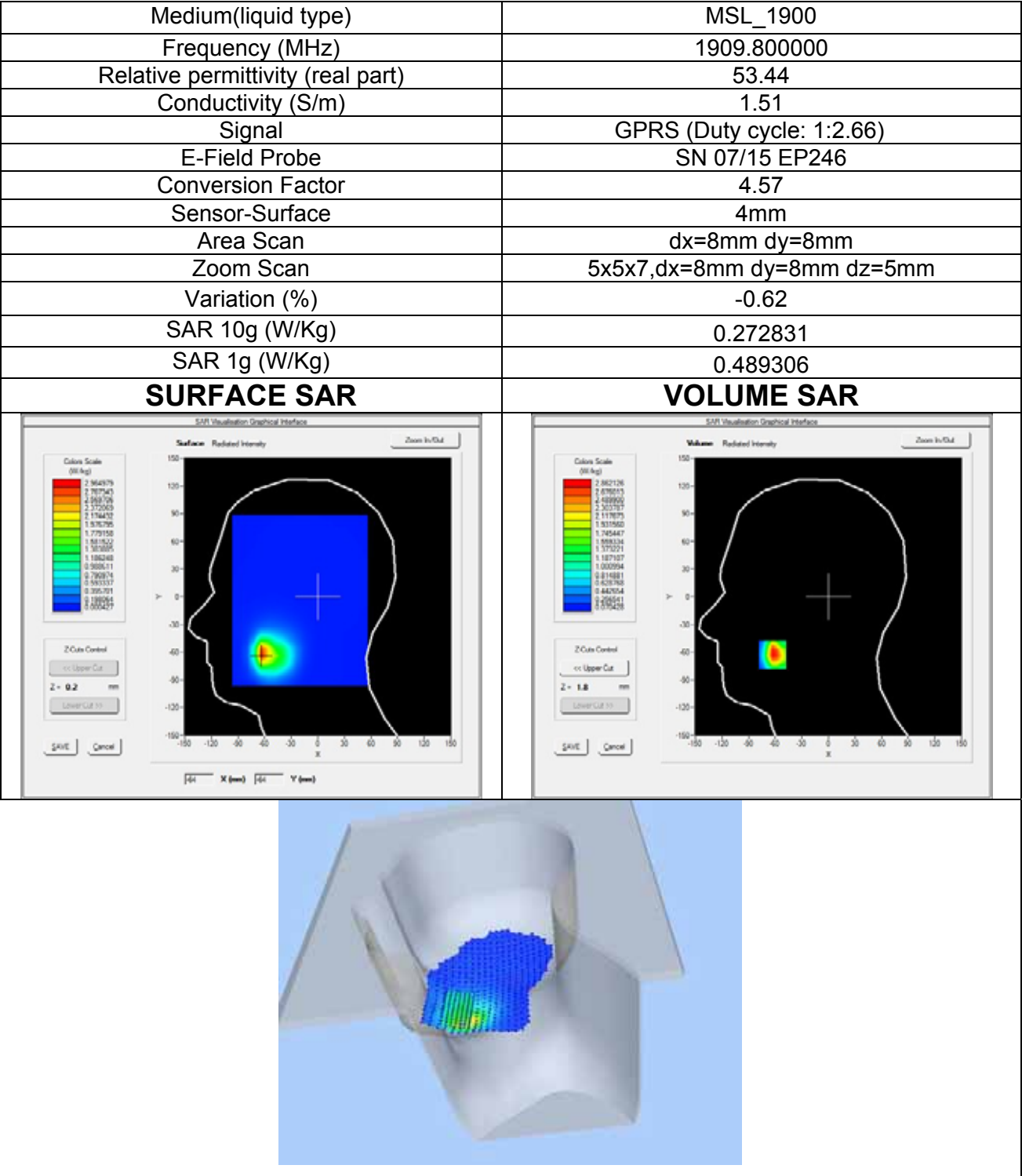
Plot 6: Right Head with Back side device position on High Channel in GSM mode
