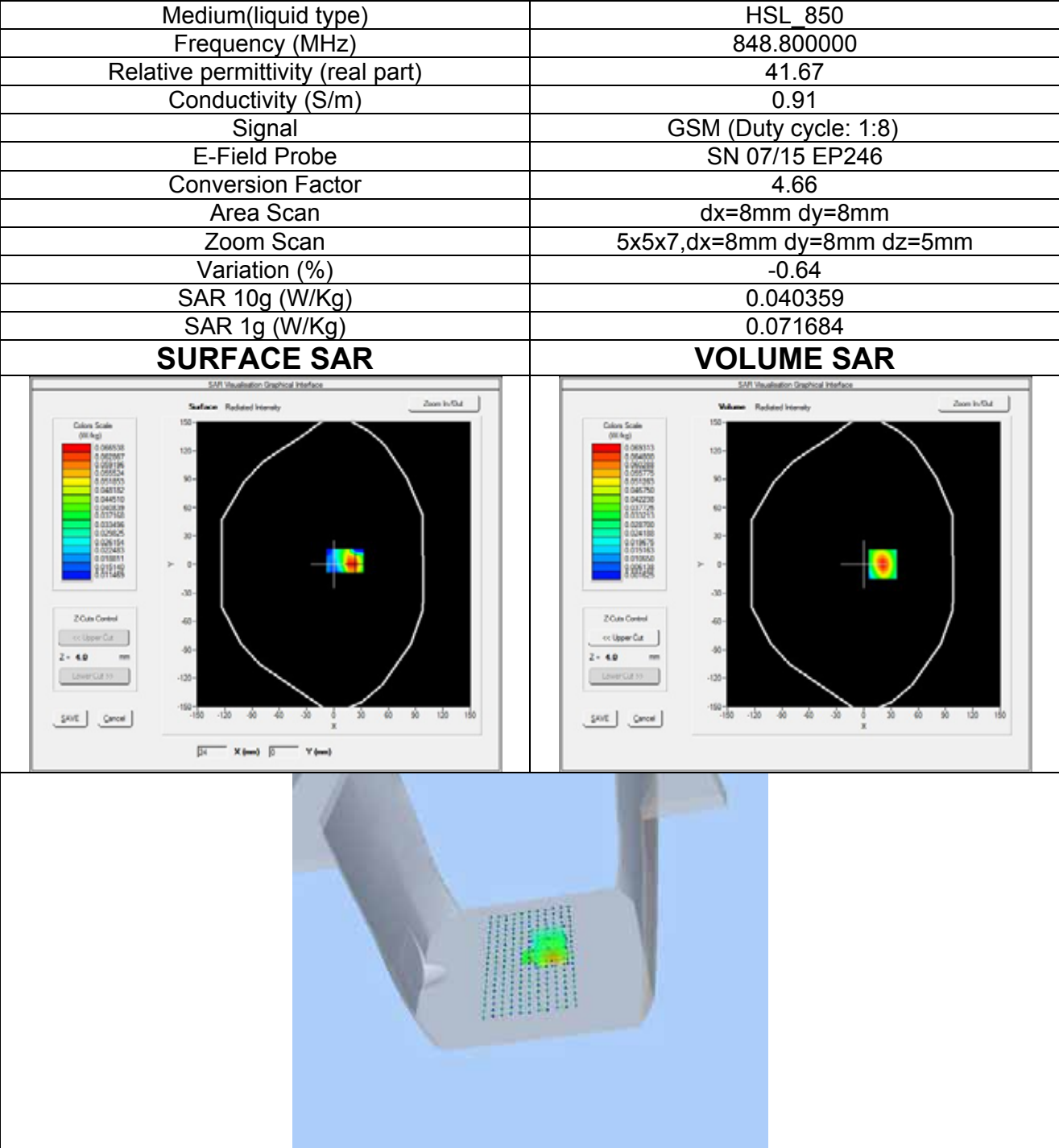
Plot 1: Flat Plane with Front side(Near to Mouth) device position on High Channel in GSM mode
