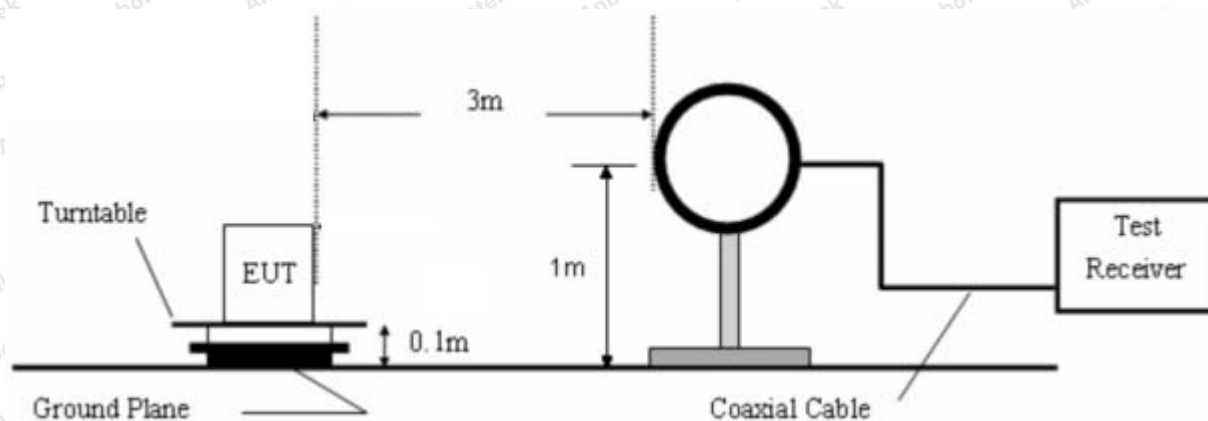
Figure 1. Below 30MHz
