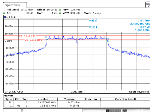
g_2437MHz_Chain 0
