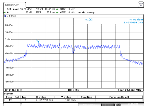
g_2462MHz_Chain 0
