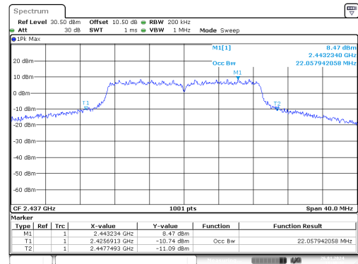
n20_2437MHz_Chain 0
