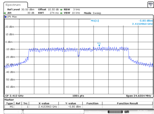
g_2412MHz_Chain 0
