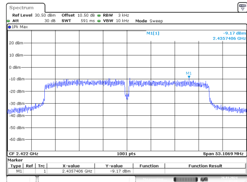
n40_2422MHz_Chain 0
