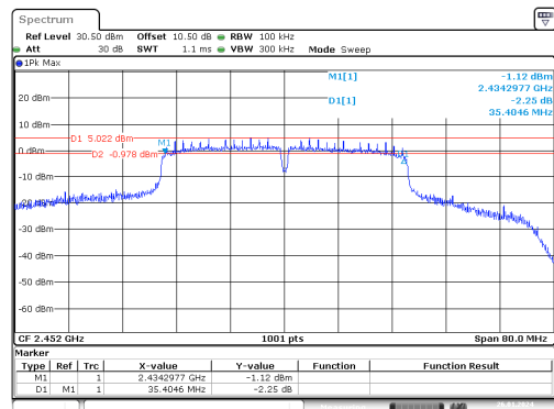
n40_2452MHz_Chain 0
