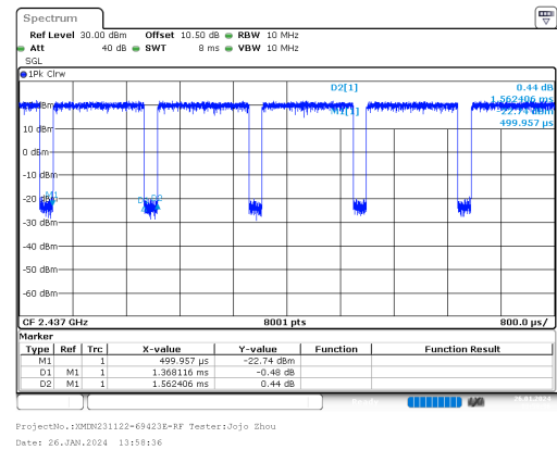
g_2437MHz_Chain 0
