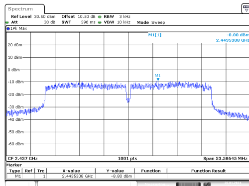
n40_2437MHz_Chain 0
