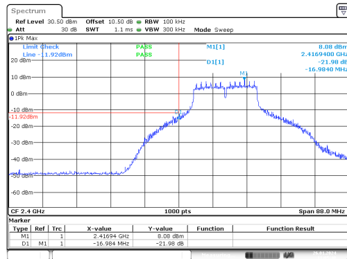
g_2412MHz_Chain 0
