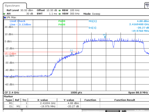
n40_2422MHz_Chain 0
