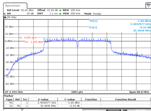
n40_2422MHz_Chain 0
