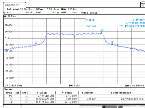
g_2437MHz_Chain 0
