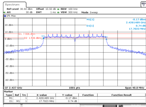
n20_2437MHz_Chain 0
