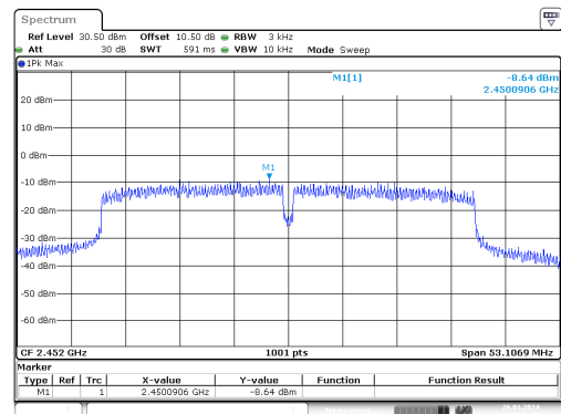
n40_2452MHz_Chain 0
