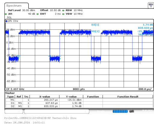
N40_2437MHz_Chain 0
