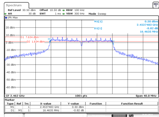
g_2462MHz_Chain 0
