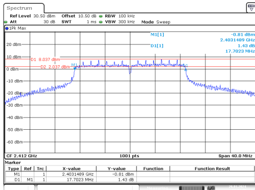
n20_2412MHz_Chain 0
