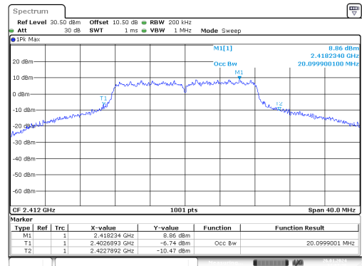
g_2412MHz_Chain 0
