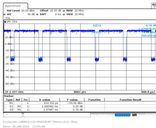
n20_2437MHz_Chain 0
