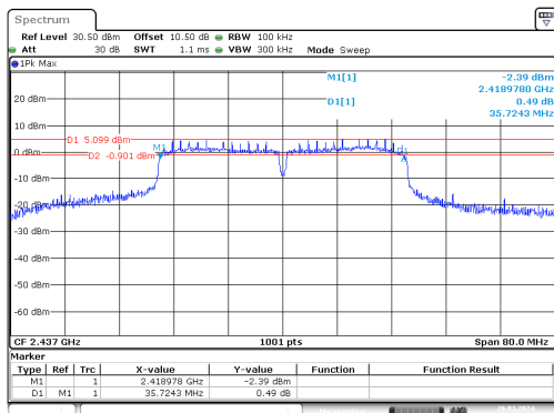
n40_2437MHz_Chain 0
