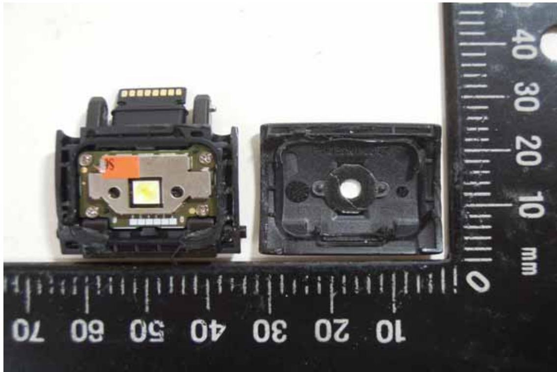
Open View of EUT-10 (Flashlight module)
