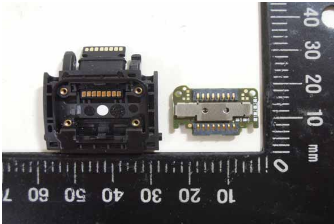
Open View of EUT-8 (Heart Rate module)
