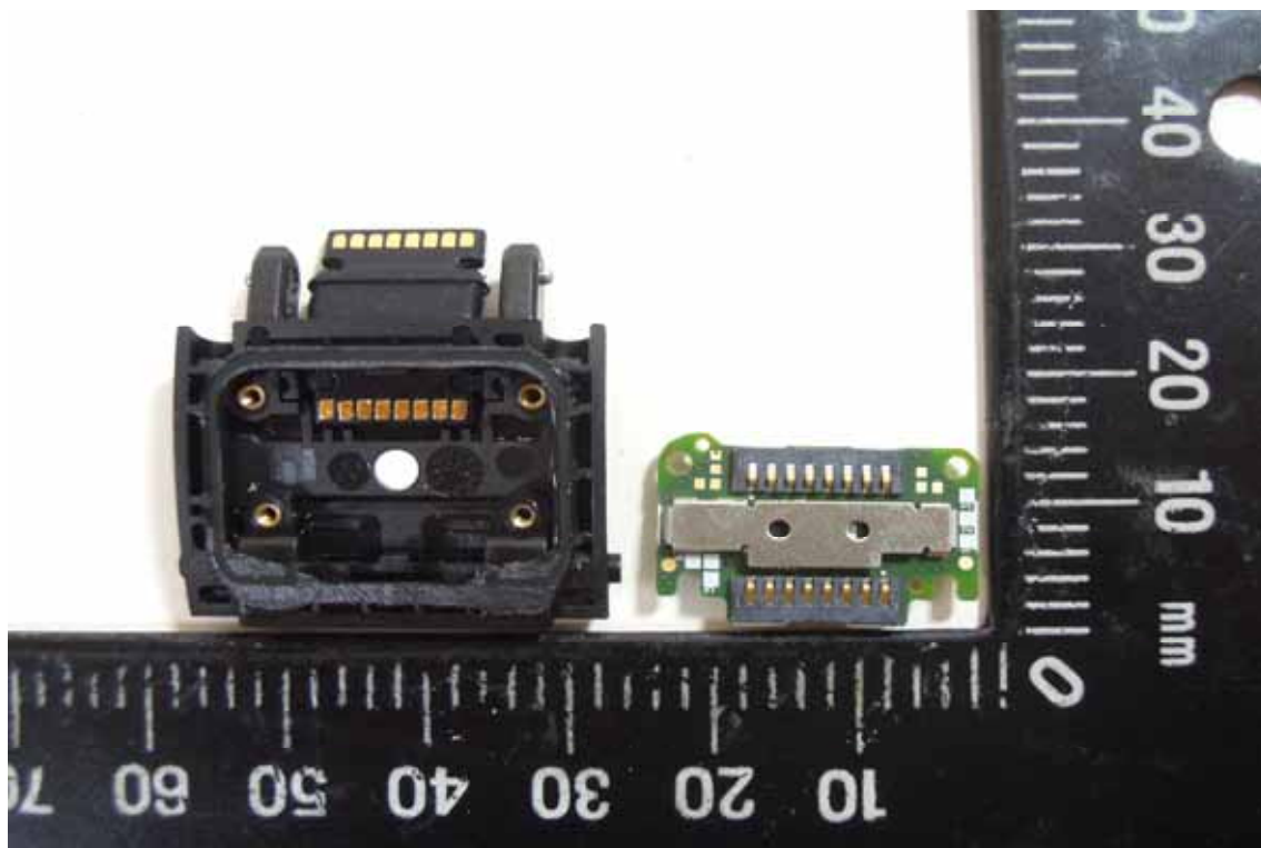
Open View of EUT-6 (Programmable button module)
