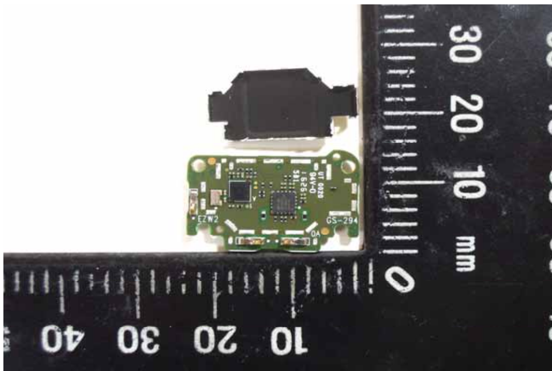
Internal View of EUT-11 (Heart Rate module)
