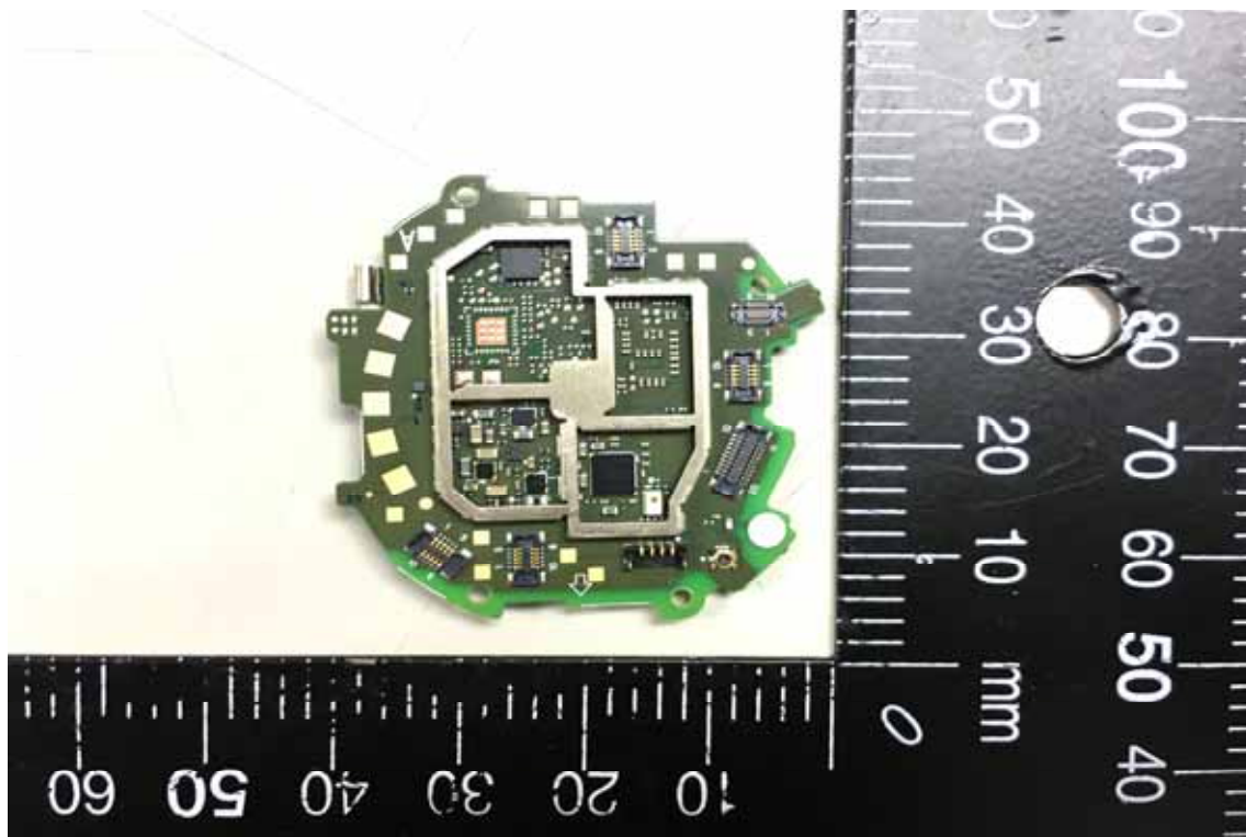
Internal View of EUT-7 (GPS module)
