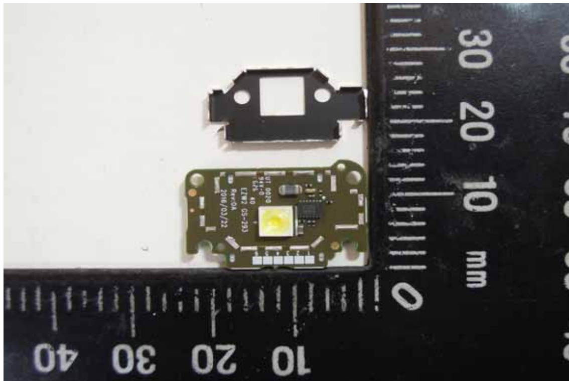
Internal View of EUT-15 (Adventure module)
