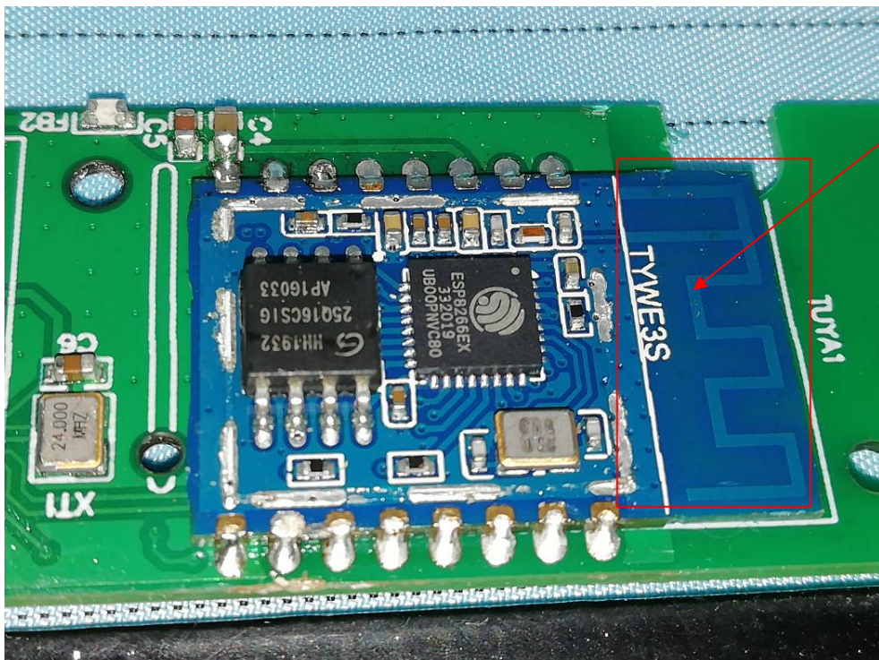
Wi-Fi Antenna
