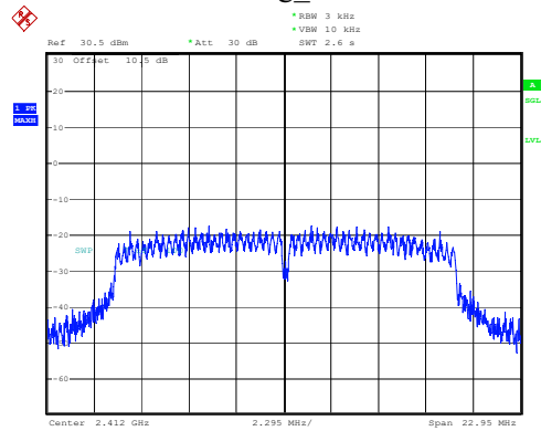
802.11g_2412MHz
