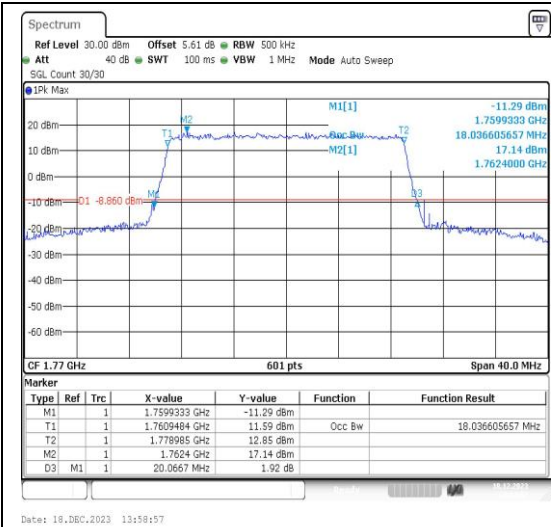
Band66-20MHz-QPSK-132572-100RB#0-PASS
