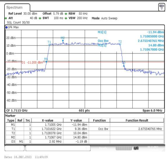
Band66-3MHz-16QAM-131987-15RB#0-PASS
