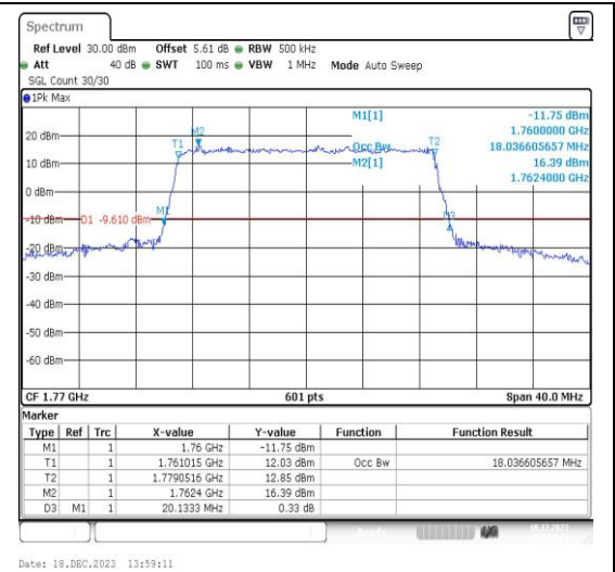
Band66-20MHz-16QAM-132572-100RB#0-PASS
