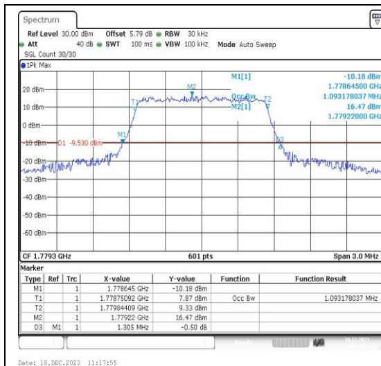
Band66-1.4MHz-QPSK-132665-6RB#0-PASS
