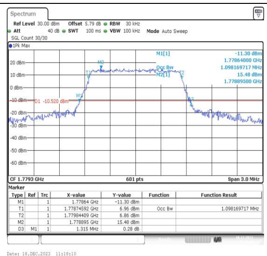
Band66-1.4MHz-16QAM-132665-6RB#0-PASS
