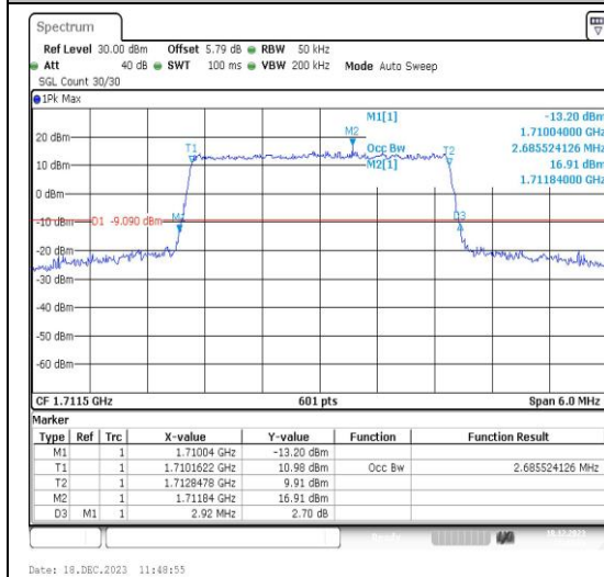
Band66-3MHz-QPSK-131987-15RB#0-PASS
