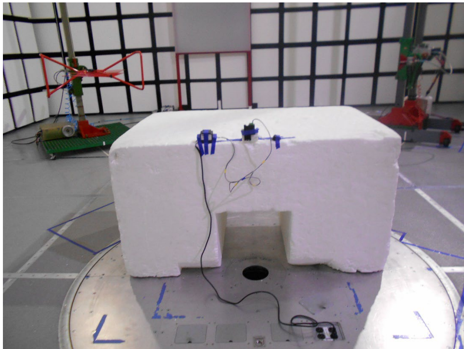
RADIATED BELOW 1GHz BACK
