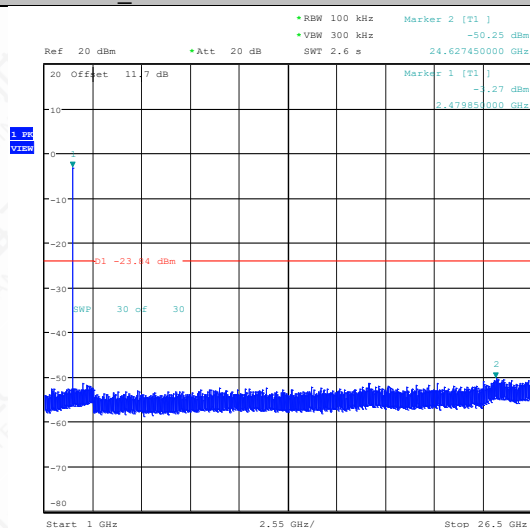
BLE_125K-Ant1-2480-1000~26500-PASS
