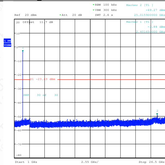
BLE_125K-Ant1-2402-1000~26500-PASS
