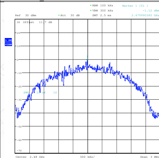
BLE_2M-Ant1-2480-0~Reference-PASS
