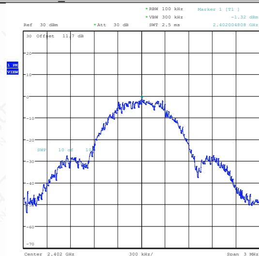
BLE_500K-Ant1-2402-0~Reference-PASS
