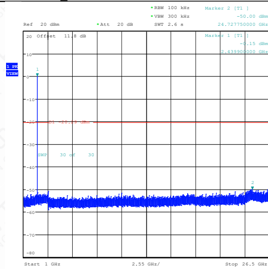
BLE_500K-Ant1-2440-1000~26500-PASS
