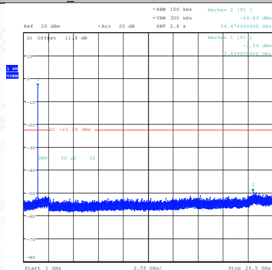
BLE_2M-Ant1-2440-1000~26500-PASS
