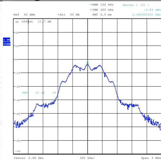
BLE_125K-Ant1-2480-0~Reference-PASS
