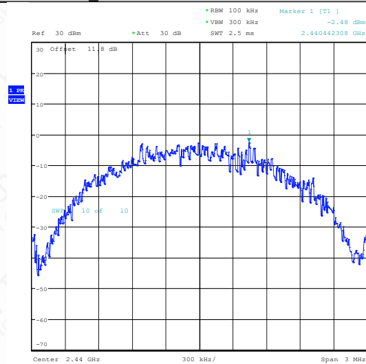
BLE_2M-Ant1-2440-0~Reference-PASS
