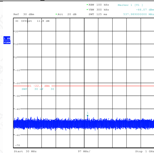
BLE_125K-Ant1-2440-30~1000-PASS
