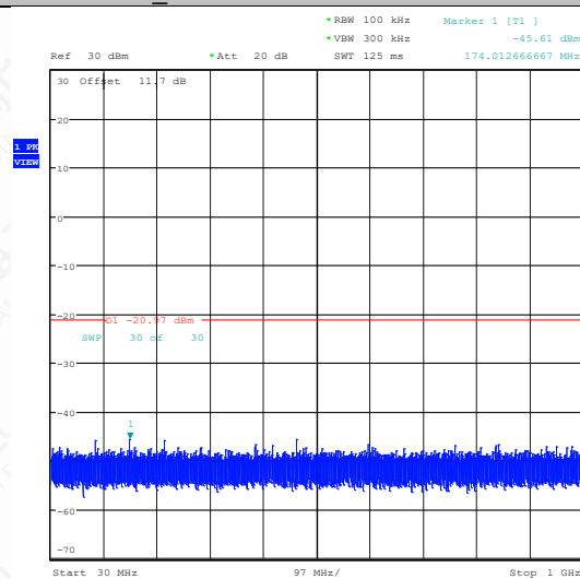
BLE_500K-Ant1-2480-30~1000-PASS
