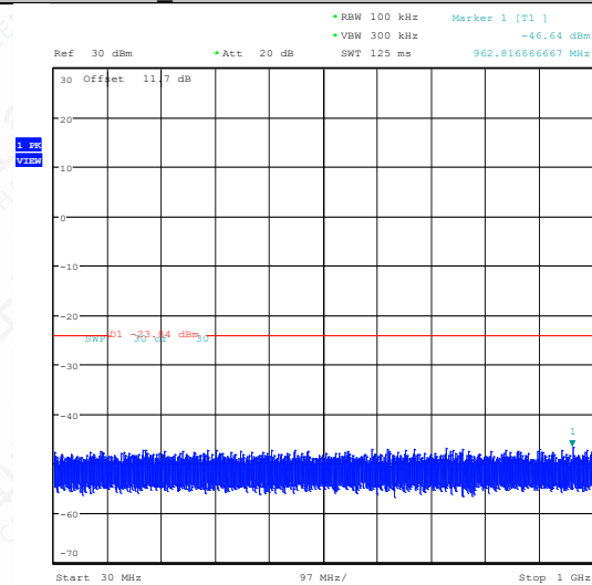
BLE_125K-Ant1-2480-30~1000-PASS
