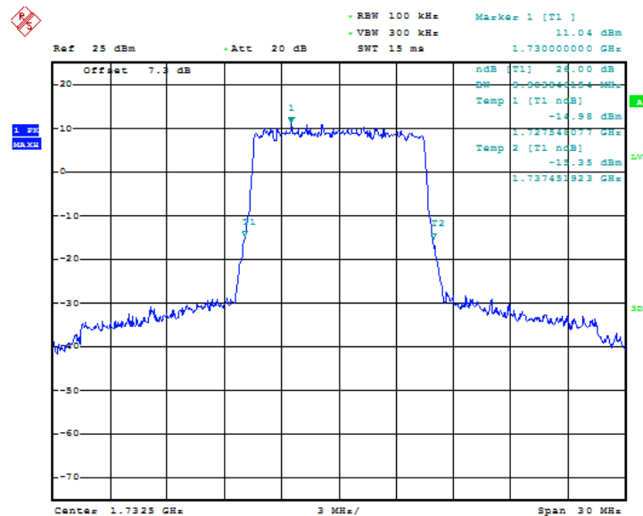
Fig.71 LTE band 4, 10MHz Bandwidth, QPSK (-26dBc BW)
