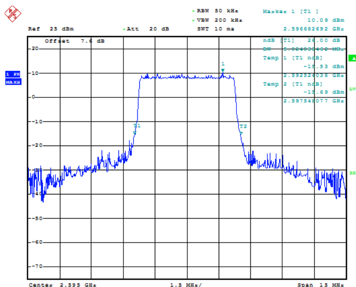
Fig.97 LTE band 41, 5MHz Bandwidth, QPSK (-26dBc BW)
