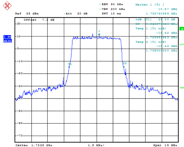
Fig.69 LTE band 4, 5MHz Bandwidth, QPSK (-26dBc BW)
