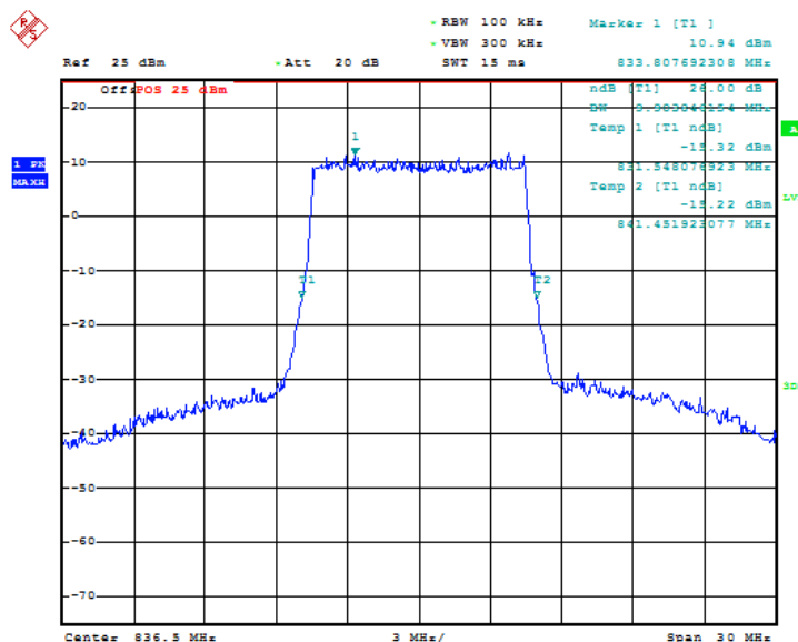
Fig.83 LTE band 5, 10MHz Bandwidth, QPSK (-26dBc BW)
