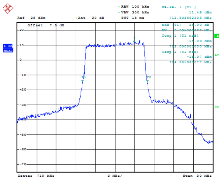
Fig.95 LTE band 17, 10MHz Bandwidth, QPSK (-26dBc BW)
