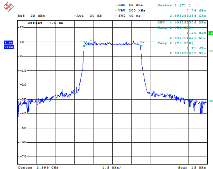
Fig.45 LTE band 41, 5MHz Bandwidth, QPSK (99% BW)
