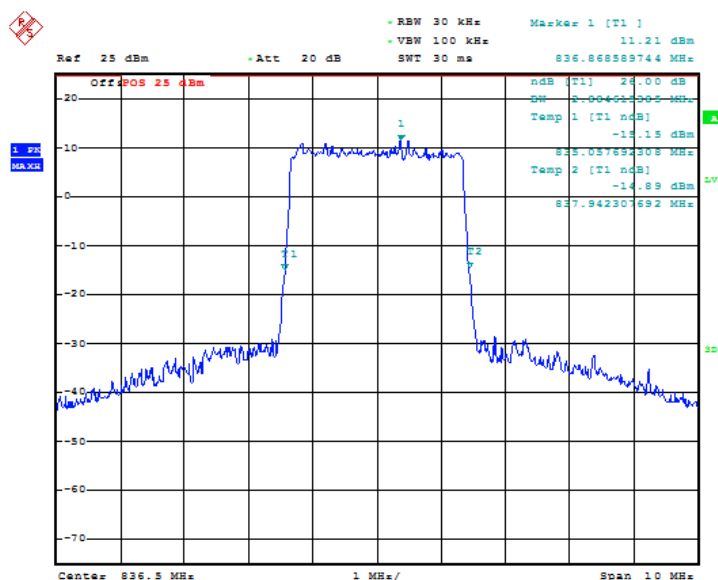
Fig.79 LTE band 5, 3MHz Bandwidth, QPSK (-26dBc BW)
