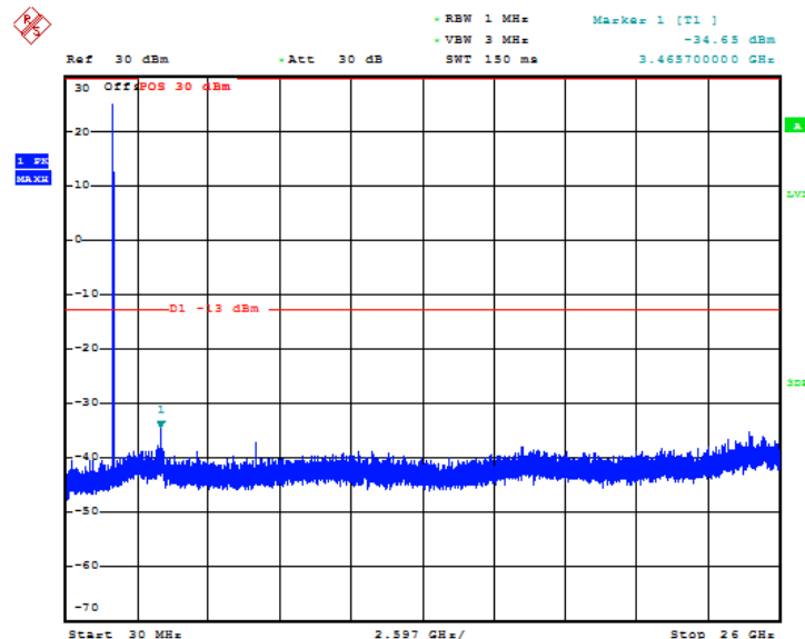
Fig.129 LTE band 2: 30MHz – 26GHz
