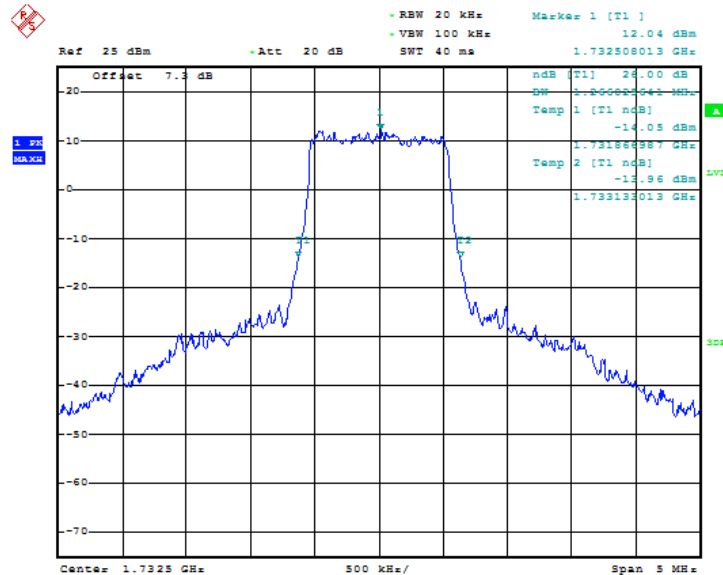
Fig.65 LTE band 4, 1.4MHz Bandwidth, QPSK (-26dBc BW)
