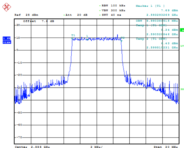
Fig.47 LTE band 41, 10MHz Bandwidth, QPSK (99% BW)
