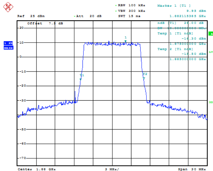
Fig.59 LTE band 2, 10MHz Bandwidth, QPSK (-26dBc BW)
