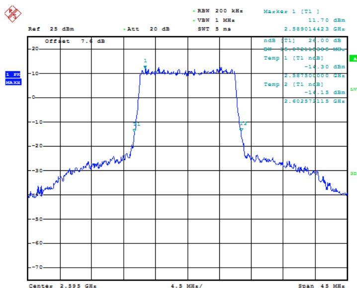
Fig.101 LTE band 41, 15MHz Bandwidth, QPSK (-26dBc BW)
