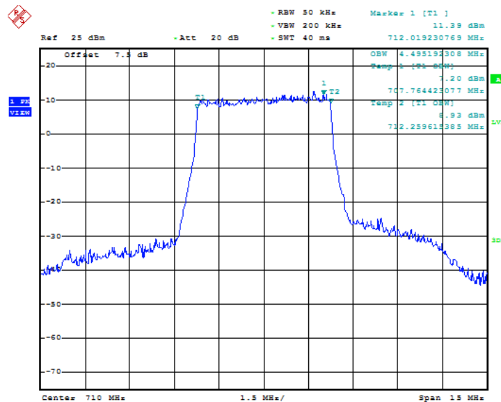
Fig.41 LTE band 17, 5MHz Bandwidth, QPSK (99% BW)
