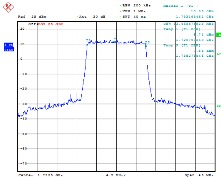
Fig.21 LTE band 4, 15MHz Bandwidth, QPSK (99% BW)
