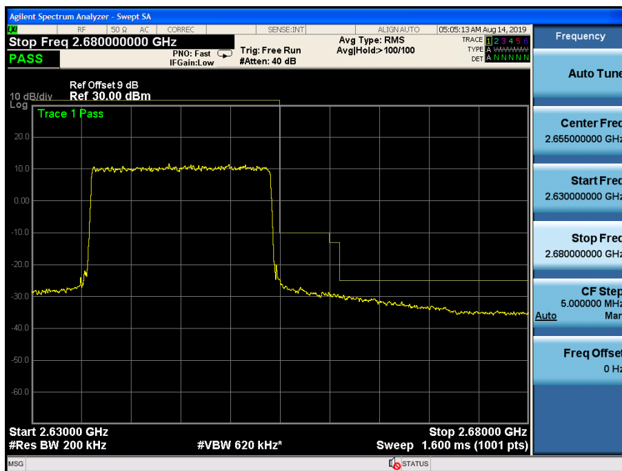
Fig.128 HIGH BAND EDGE BLOCK-20MHz-100%RB
