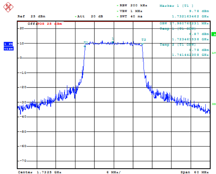
Fig.23 LTE band 4, 20MHz Bandwidth, QPSK (99% BW)
