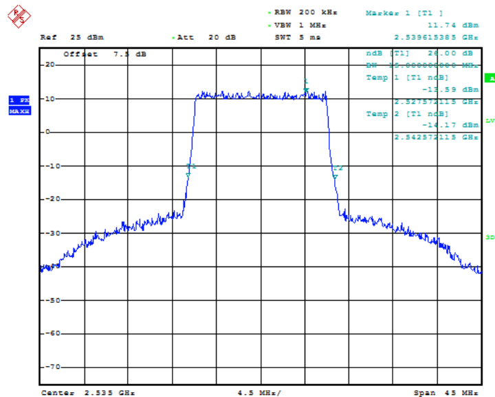
Fig.89 LTE band 7, 15MHz Bandwidth, QPSK (-26dBc BW)
