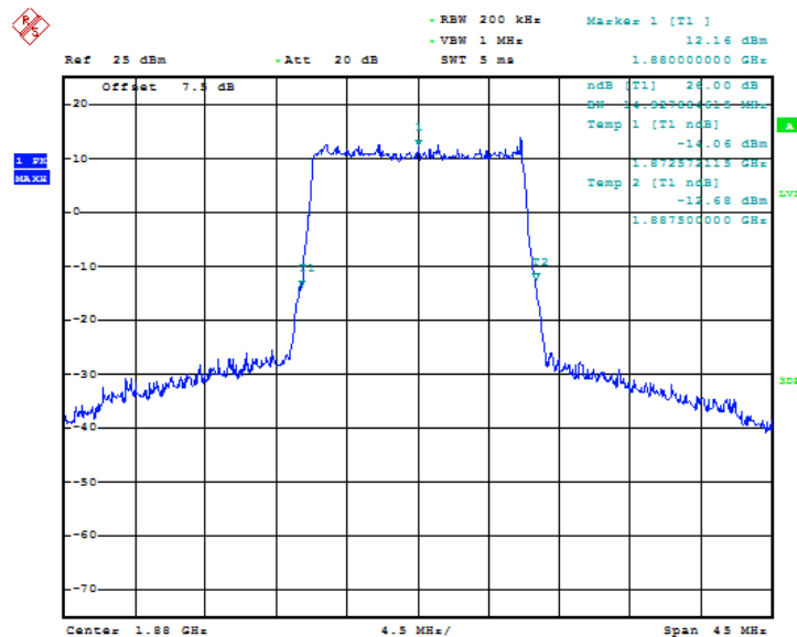
Fig.61 LTE band 2, 15MHz Bandwidth, QPSK (-26dBc BW)
