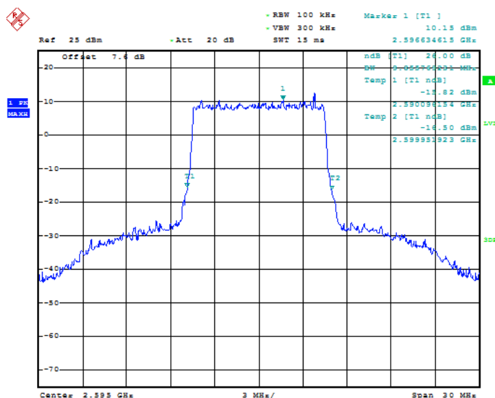
Fig.99 LTE band 41, 10MHz Bandwidth, QPSK (-26dBc BW)
