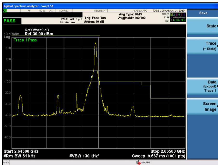
Fig.126 HIGH BAND EDGE BLOCK-1RB-high_offset
