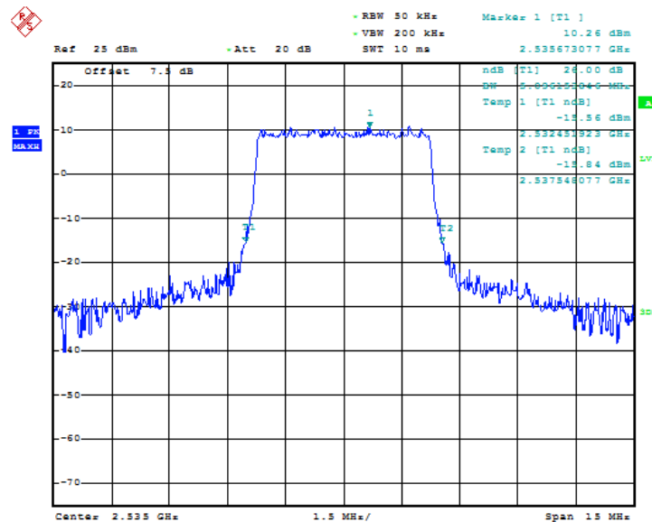
Fig.85 LTE band 7, 5MHz Bandwidth, QPSK (-26dBc BW)
