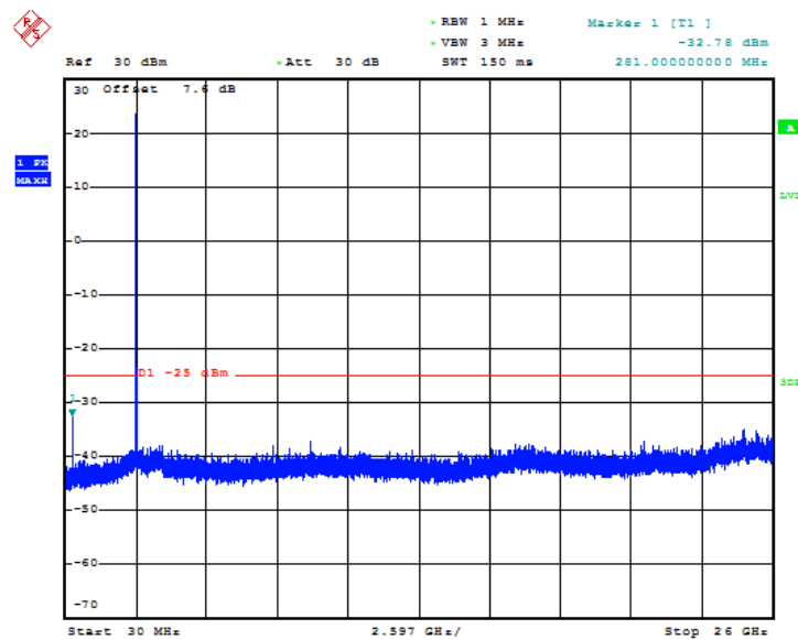
Fig.133 LTE band 17: 30MHz – 26GHz
