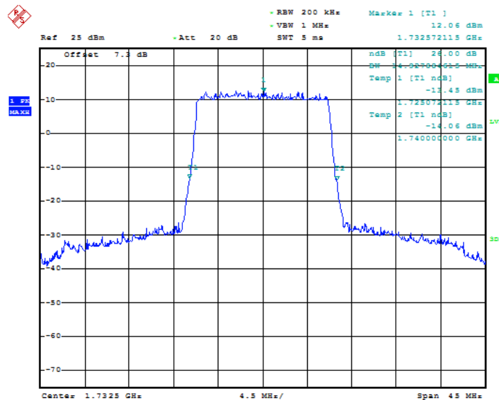
Fig.73 LTE band 4, 15MHz Bandwidth, QPSK (-26dBc BW)
