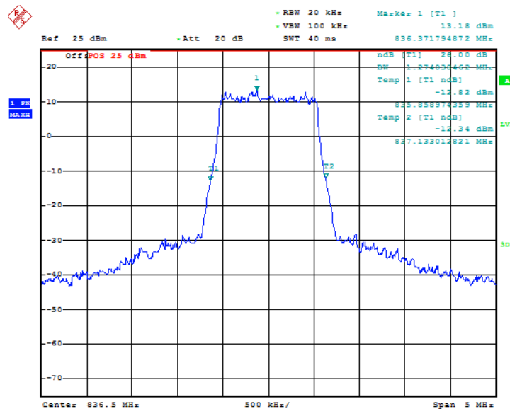
Fig.77 LTE band 5, 1.4MHz Bandwidth, QPSK (-26dBc BW)
