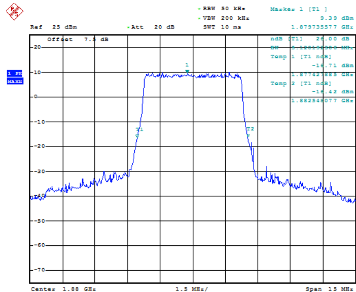
Fig.57 LTE band 2, 5MHz Bandwidth, QPSK (-26dBc BW)
