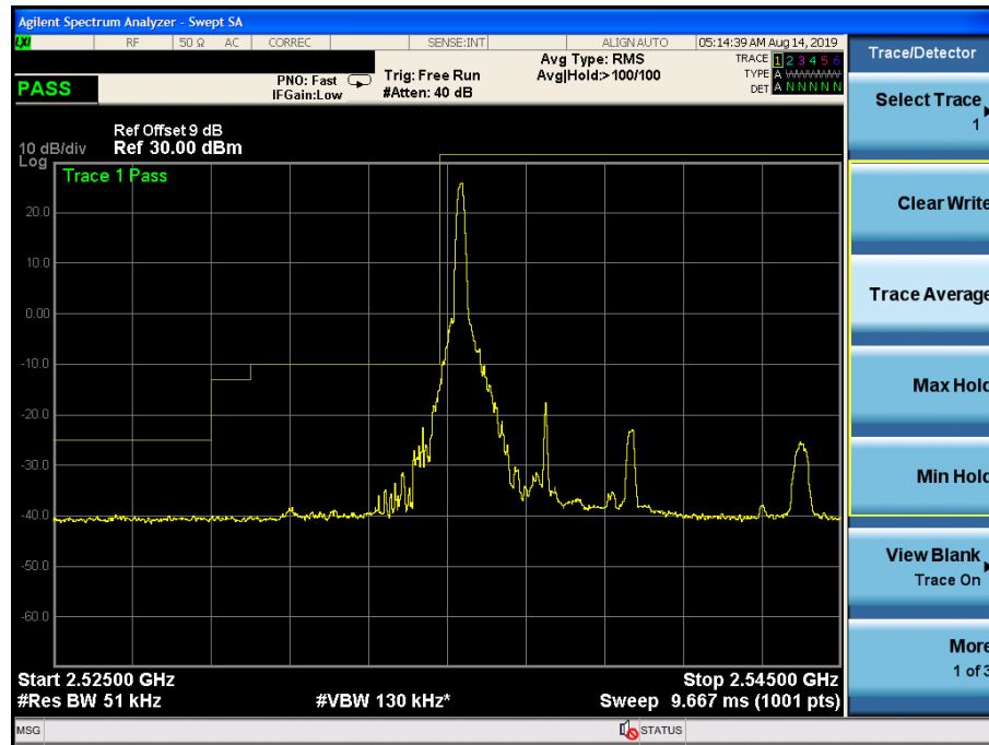
Fig.125 LOW BAND EDGE BLOCK-1RB-low_offset
