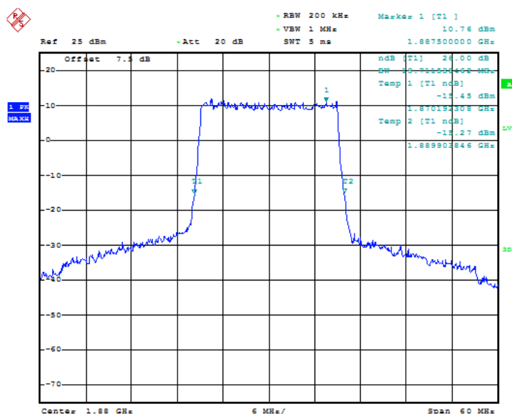
Fig.63 LTE band 2, 20MHz Bandwidth, QPSK (-26dBc BW)
