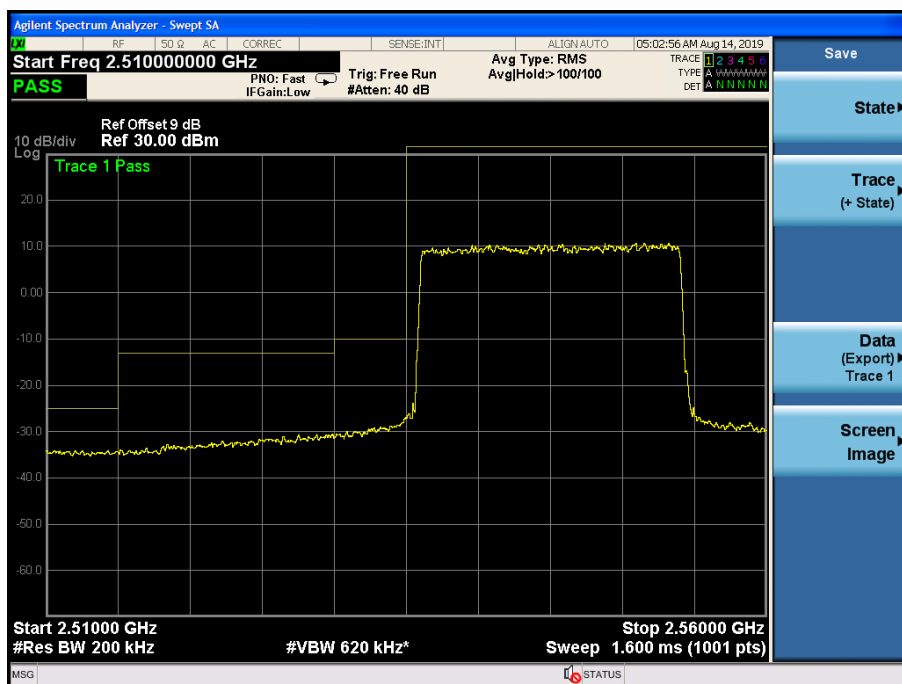
Fig.127 LOW BAND EDGE BLOCK-20MHz-100%RB
