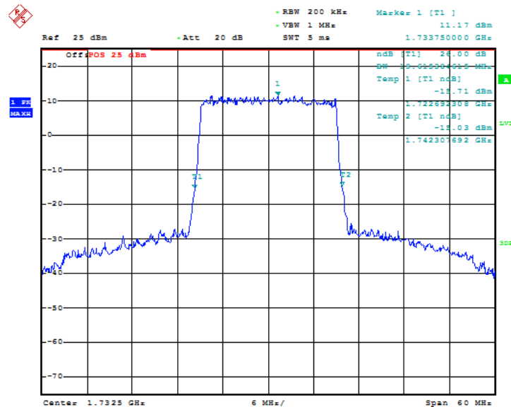
Fig.75 LTE band 4, 20MHz Bandwidth, QPSK (-26dBc BW)
