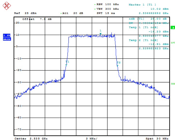
Fig.87 LTE band 7, 10MHz Bandwidth, QPSK (-26dBc BW)
