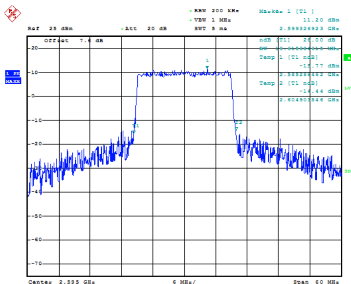
Fig.103 LTE band 41, 20MHz Bandwidth, QPSK (-26dBc BW)
