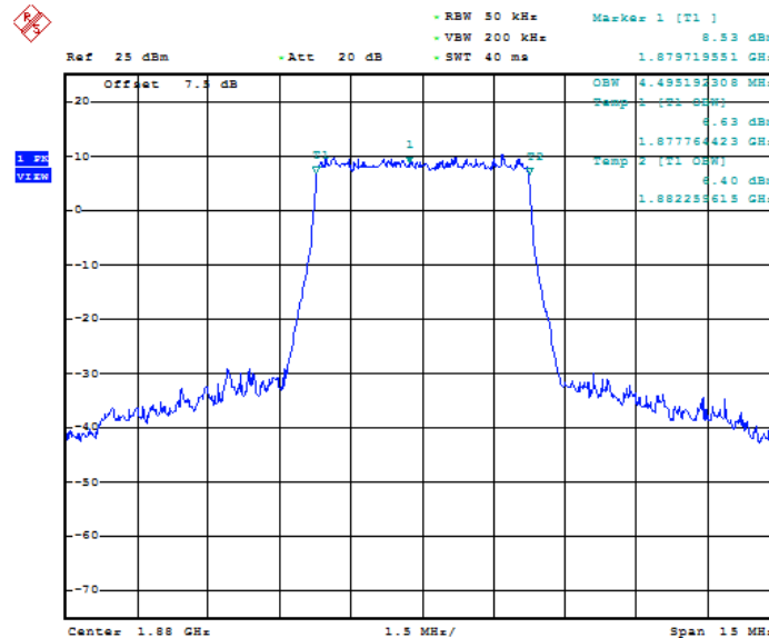
Fig.5 LTE band 2, 5MHz Bandwidth, QPSK (99% BW)
