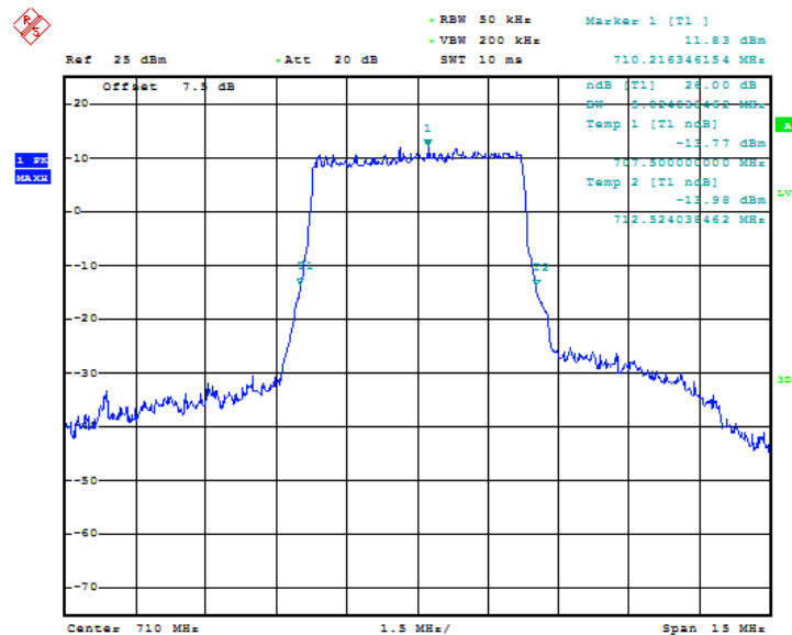
Fig.93 LTE band 17, 5MHz Bandwidth, QPSK (-26dBc BW)
