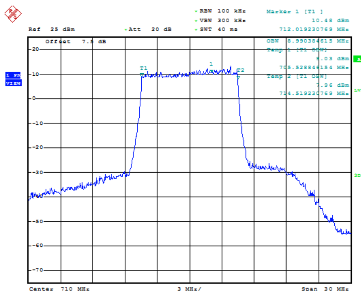
Fig.43 LTE band 17, 10MHz Bandwidth, QPSK (99% BW)
