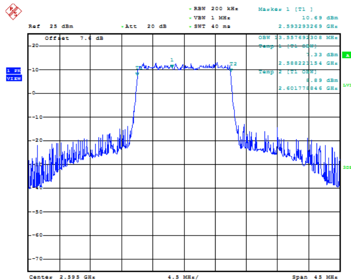
Fig.49 LTE band 41, 15MHz Bandwidth, QPSK (99% BW)
