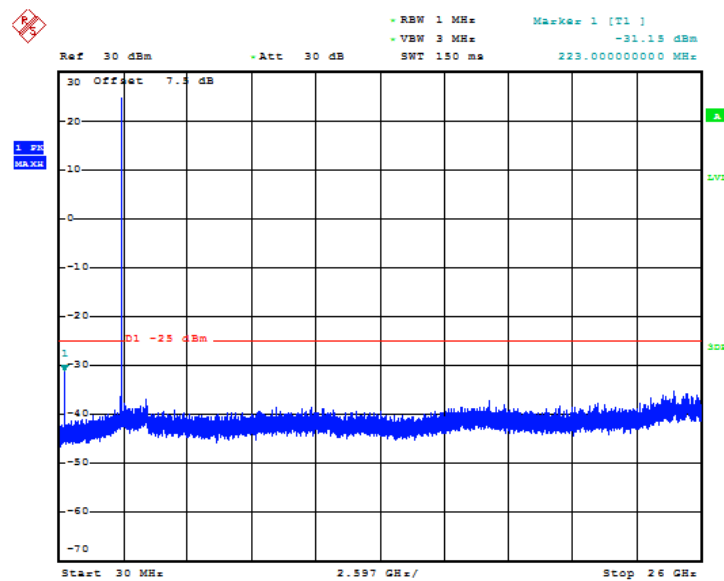
Fig.131 LTE band 5: 30MHz – 26GHz
