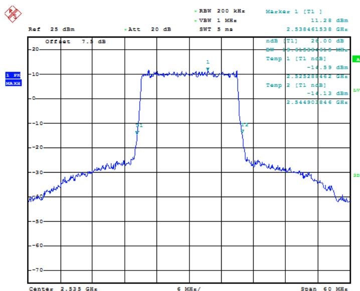
Fig.91 LTE band 7, 20MHz Bandwidth, QPSK (-26dBc BW)
