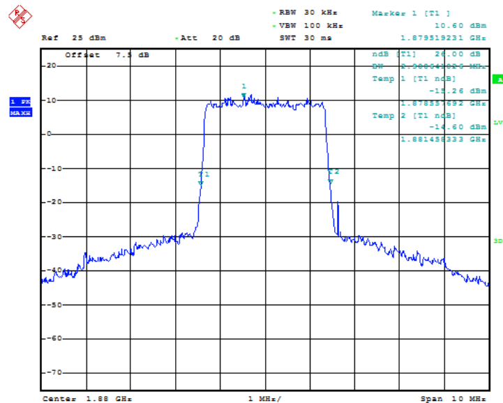
Fig.55 LTE band 2, 3MHz Bandwidth, QPSK (-26dBc BW)
