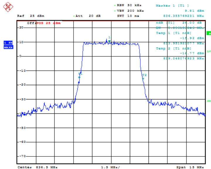
Fig.81 LTE band 5, 5MHz Bandwidth, QPSK (-26dBc BW)
