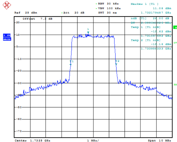
Fig.67 LTE band 4, 3MHz Bandwidth, QPSK (-26dBc BW)
