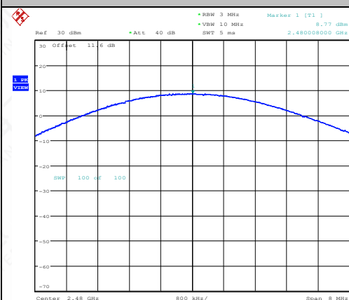
3DH5-Ant1-2480-PASS
