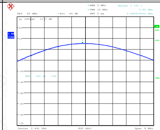
3DH5-Ant1-2441-PASS
