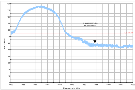
802.11b-Channel 11 Peak
