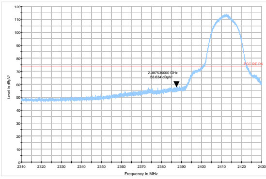
802.11b-Channel 1 Peak
