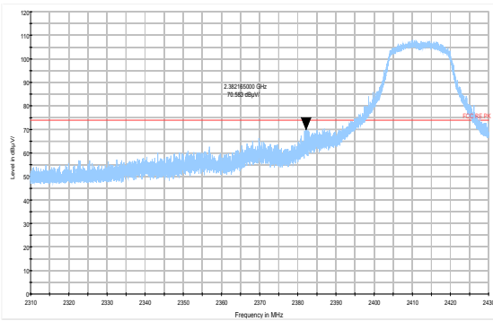
802.11g-Channel 1 Peak
