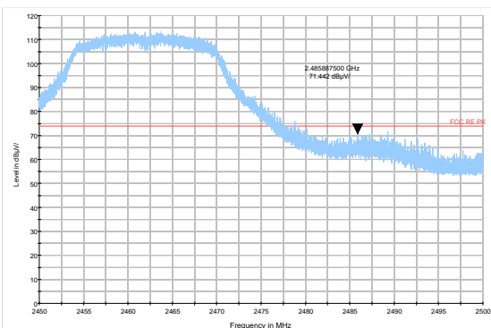
802.11g-Channel 11 Peak
