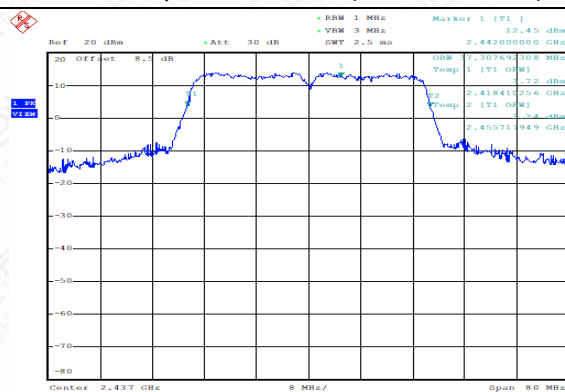
99% Occupied Bandwidth (802.11n40, Ch6)
