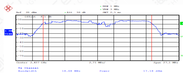
Output Power-Conducted (802.11n-HT20, Ch6)
