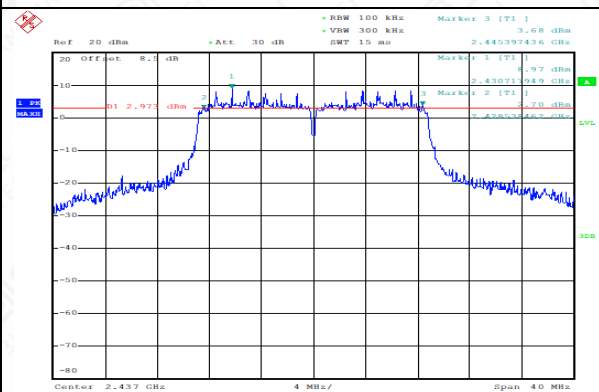
Occupied 6dB Bandwidth (MHz) (802.11n-20MHz, Ch6)
