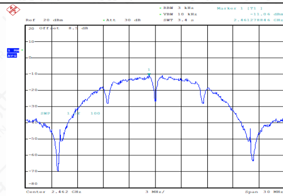
Power Spectral Density (802.11b, Ch11)
