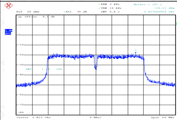
Power Spectral Density (802.11n-40MHz, Ch3)
