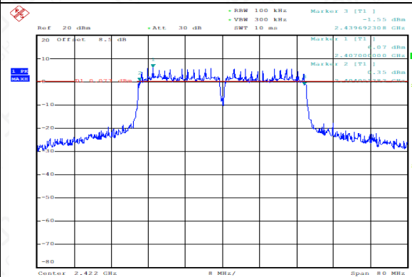
Occupied 6dB Bandwidth (MHz) (802.11n-40MHz, Ch3)
