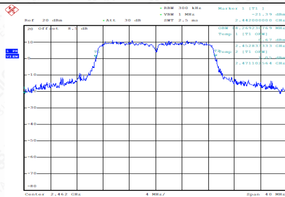
99% Occupied Bandwidth (802.11n20, Ch11)
