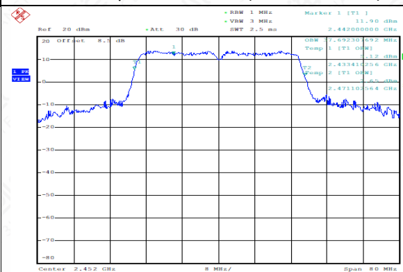
99% Occupied Bandwidth (802.11n40, Ch9)
