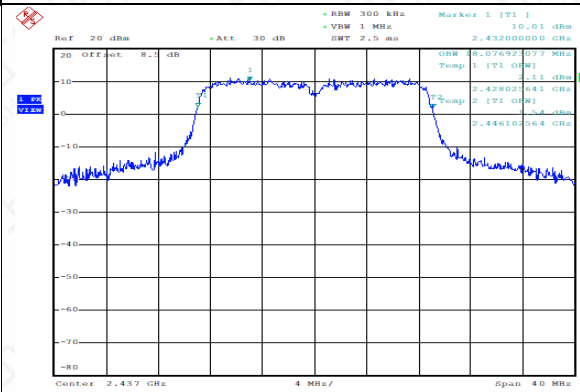
99% Occupied Bandwidth (802.11n20, Ch6)
