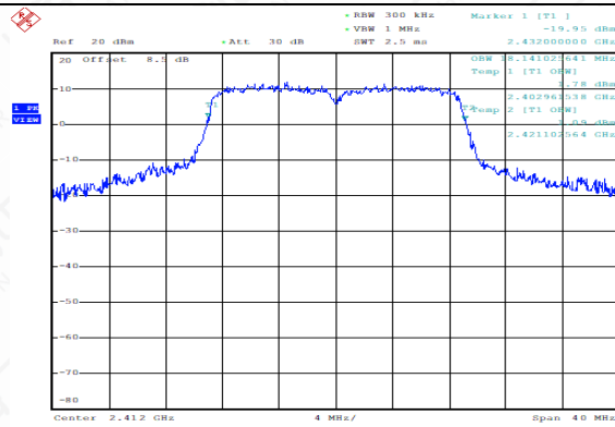
99% Occupied Bandwidth (802.11n20, Ch1)
