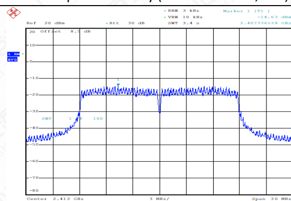
Power Spectral Density (802.11n-20MHz, Ch1)
