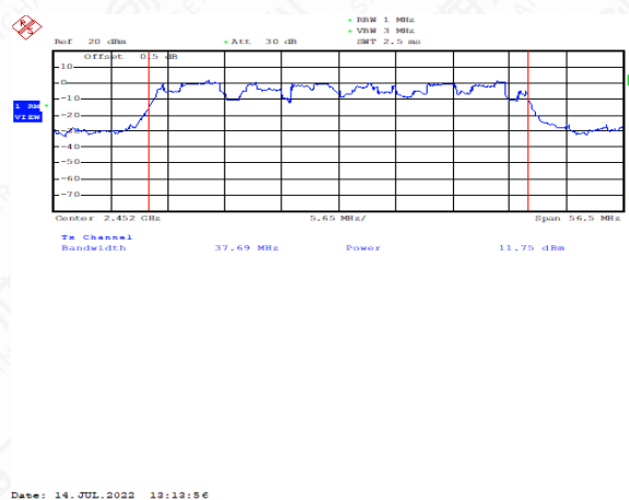
Output Power-Conducted (802.11n-HT40, Ch9)
