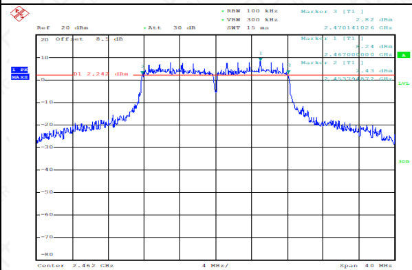
Occupied 6dB Bandwidth (MHz) (802.11g, Ch11)
