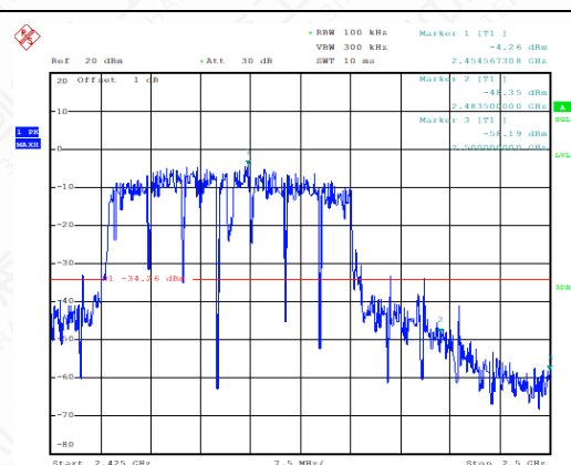
Band Edges (802.11n-20MHz, Ch9)
