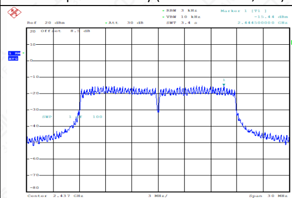
Power Spectral Density (802.11n-20MHz, Ch6)
