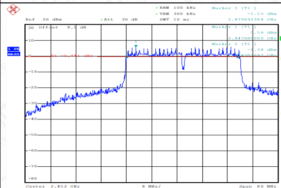
Occupied 6dB Bandwidth (MHz) (802.11n-40MHz, Ch9)
