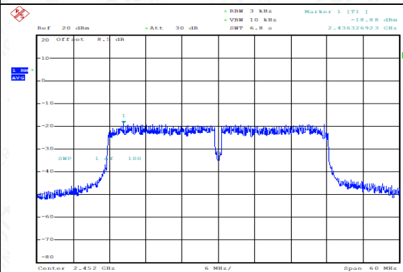
Power Spectral Density (802.11n-40MHz, Ch9)
