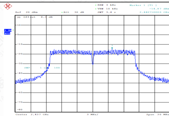
Power Spectral Density (802.11g, Ch6)
