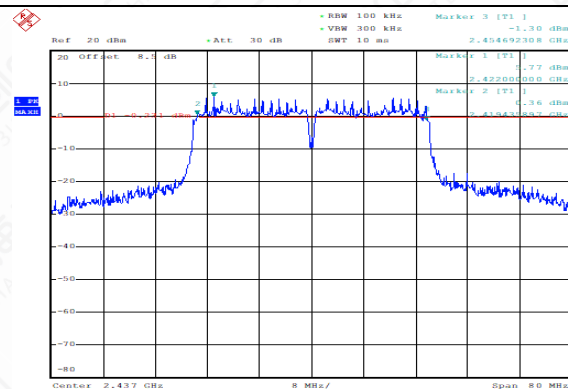
Occupied 6dB Bandwidth (MHz) (802.11n-40MHz, Ch6)
