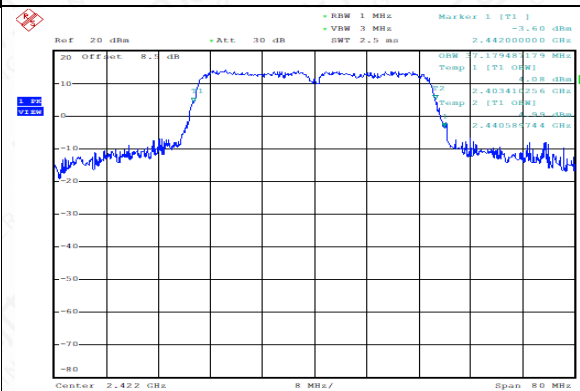
99% Occupied Bandwidth (802.11n40, Ch3)
