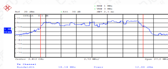
Output Power-Conducted (802.11n-HT20, Ch1)
