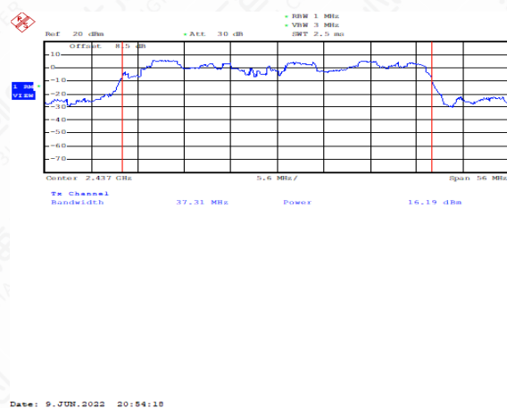
Output Power-Conducted (802.11n-HT40, Ch6)
