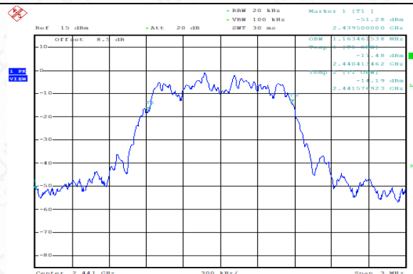
99% Bandwidth: 8DPSK, Ch39
