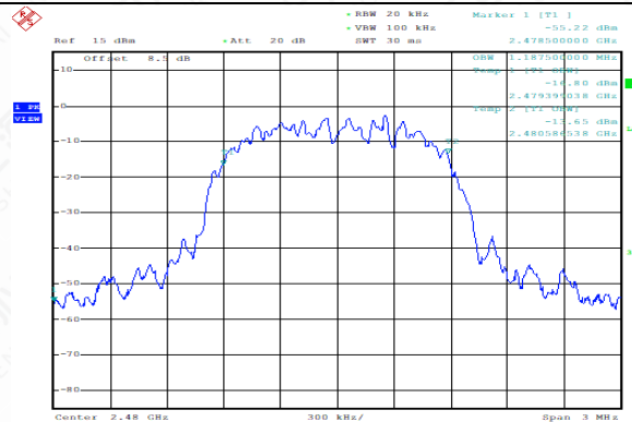
99% Bandwidth: DQPSK, Ch78
