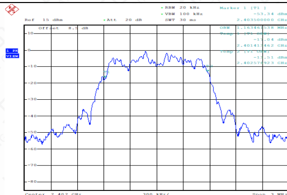
99% Bandwidth: 8DPSK, Ch0
