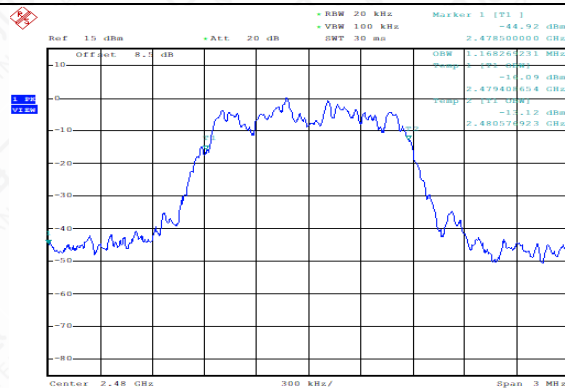
99% Bandwidth: 8DPSK, Ch78
