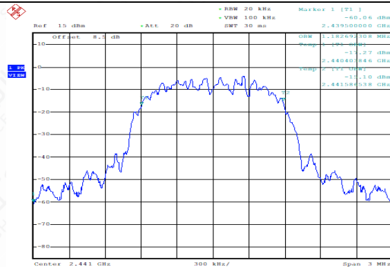
99% Bandwidth: DQPSK, Ch39
