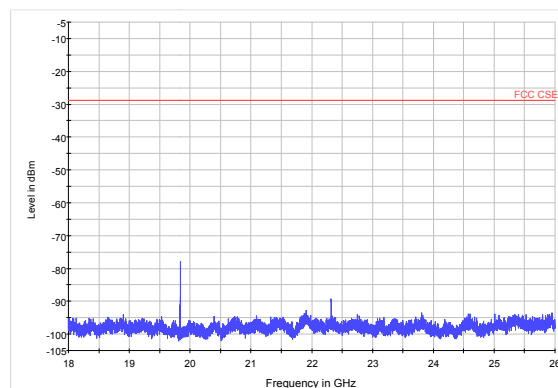
Spurious RF conducted emissions from 18GHz to 26GHz
