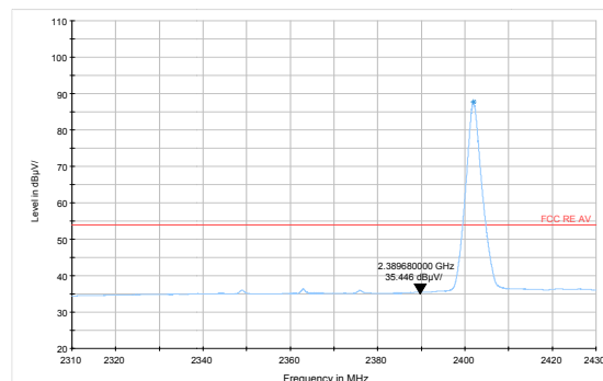
Lower band edge average-CH 0
