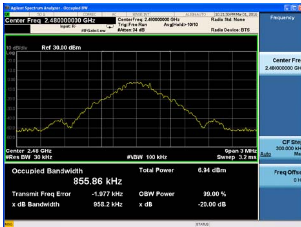
DH5 Channel No.:78
