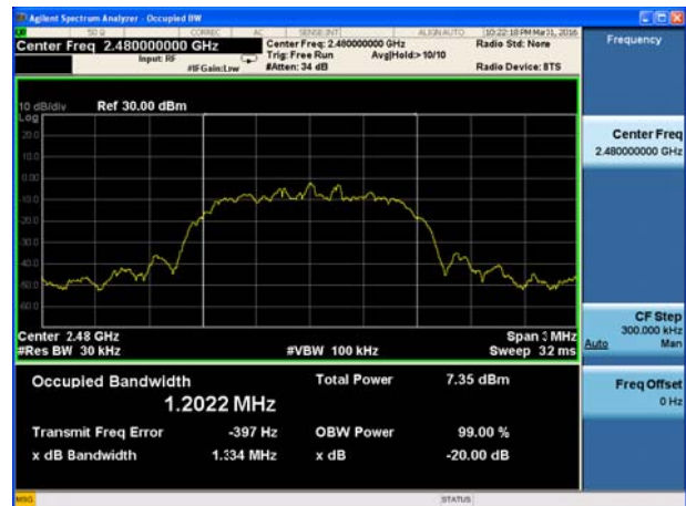
2DH5 Channel No.:78
