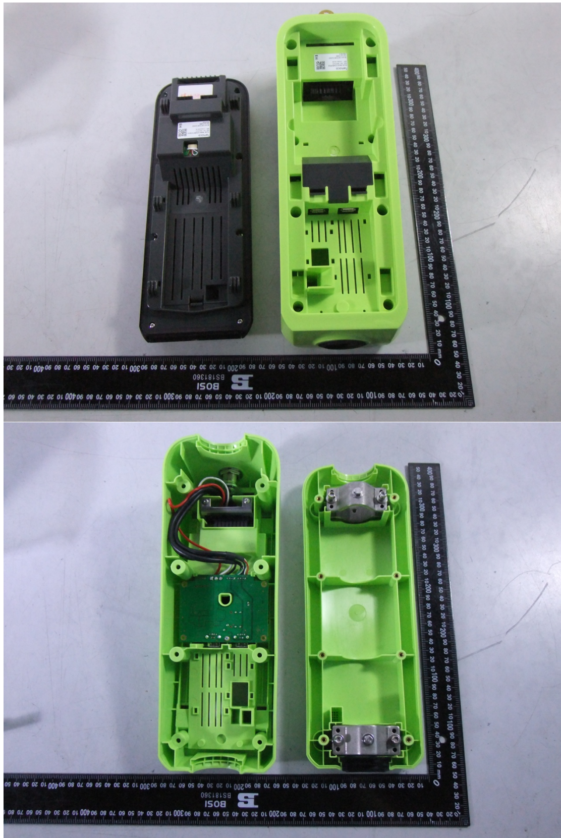
Inside of FX925F PM
