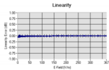
Linearity I±1.14% (±0.05dB)
